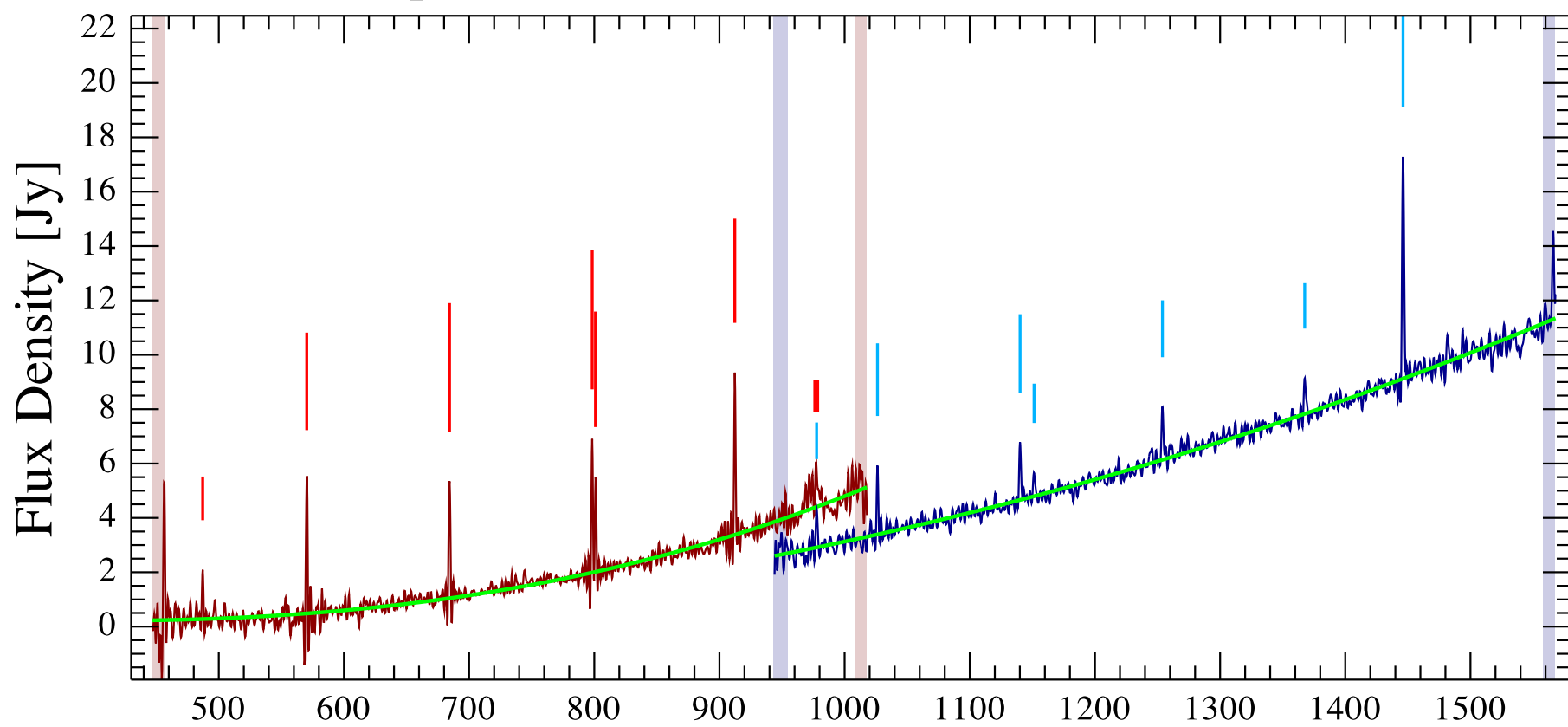
Arp299-C Observation ID 1342199250; (7/5)
