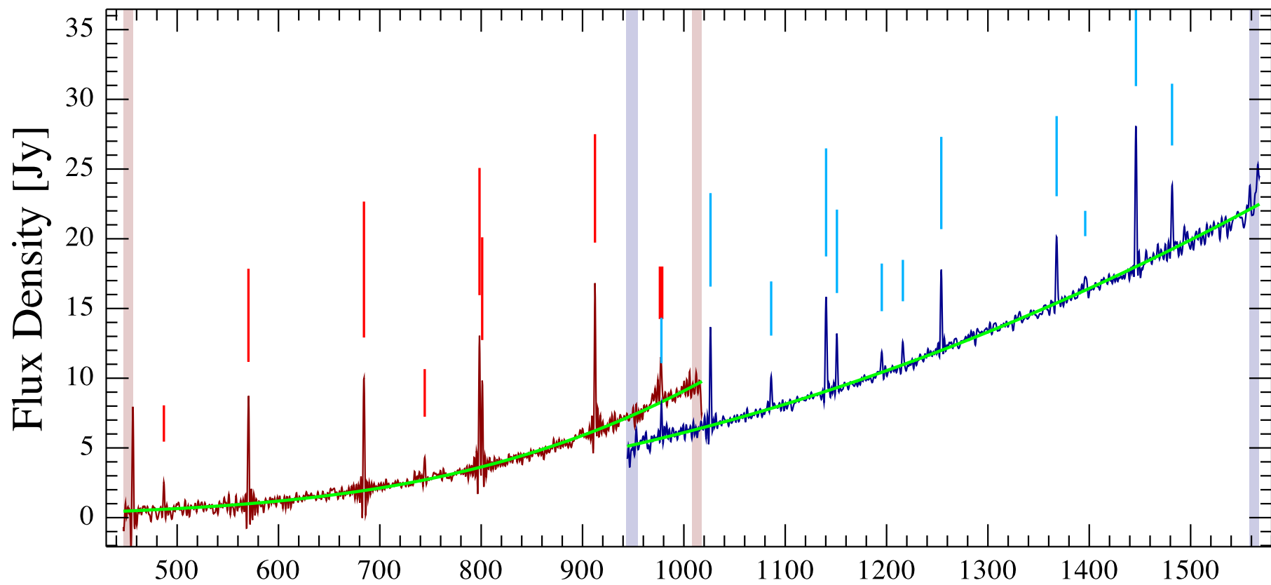
Arp299-A Observation ID 1342199248; (8/12)
