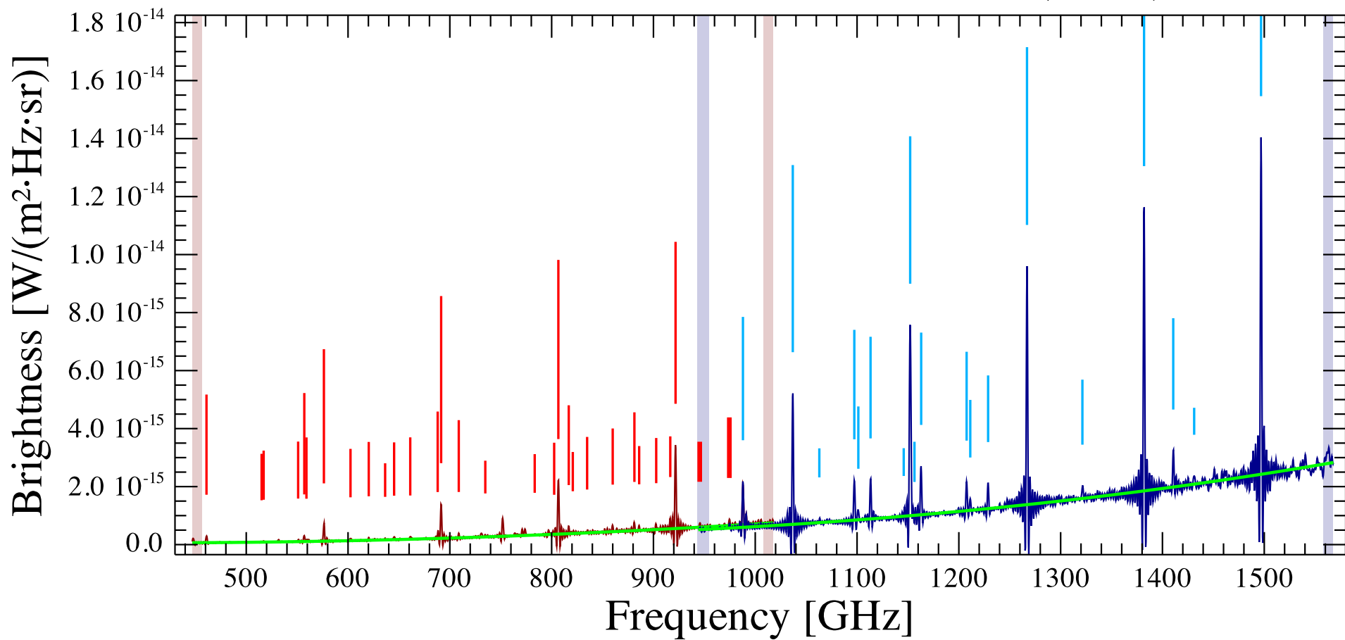
OMC-1 Observation ID 1342193671; (30/19)
