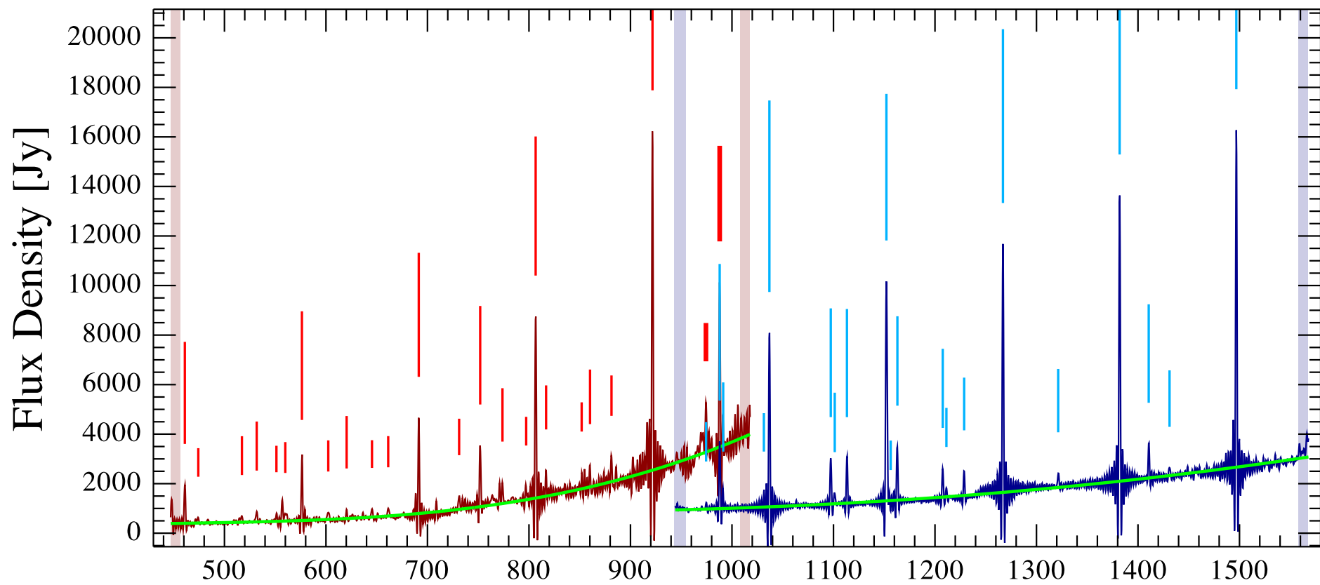
OMC-1 Observation ID 1342193671; (30/19)
