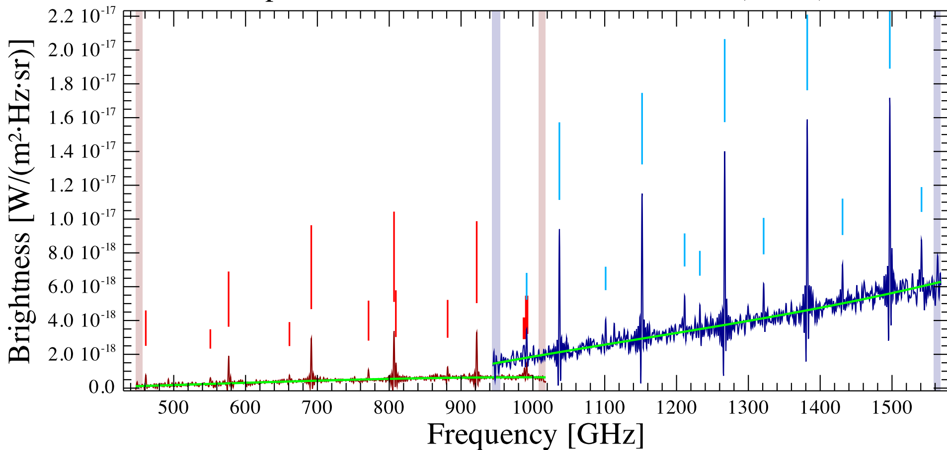
alpha ori Observation ID 1342193663; (12/12)
