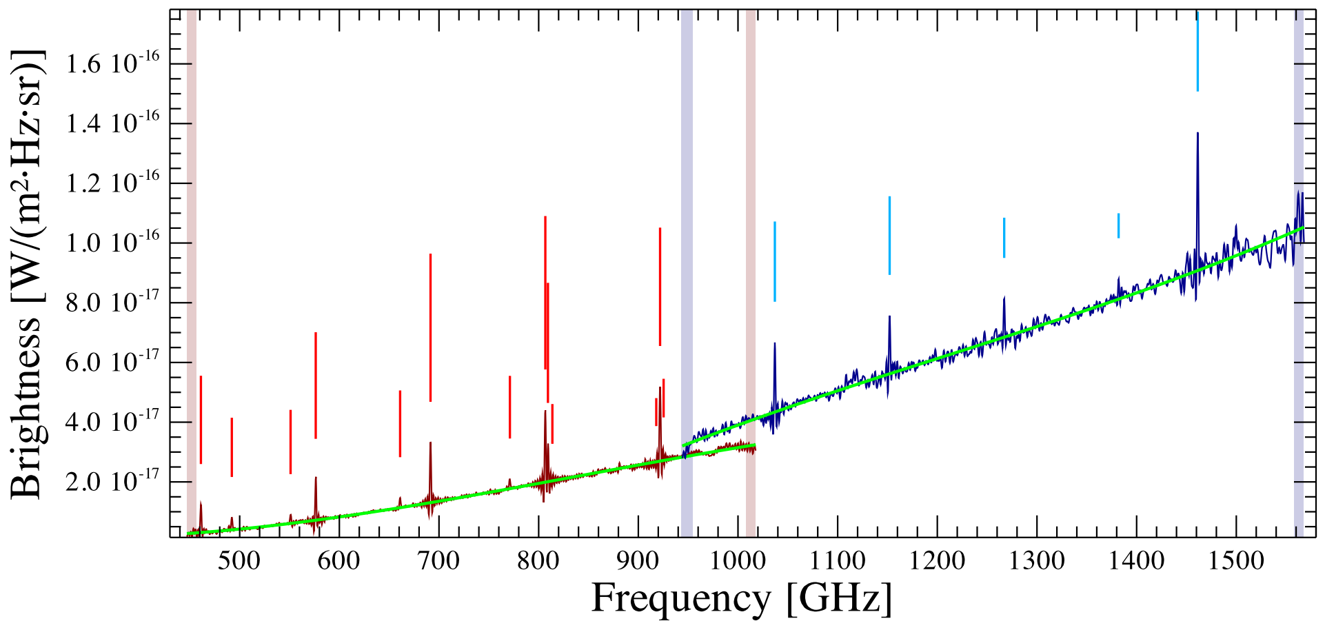
rcw120c2 Observation ID 1342191231; (13/5)
