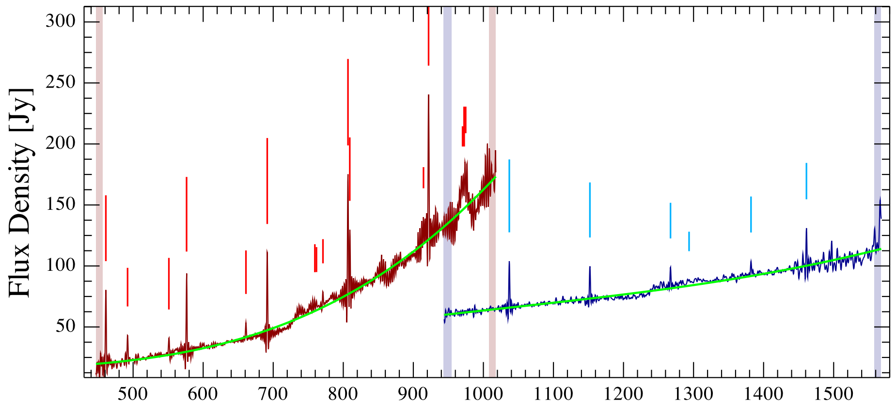
rcw120c2 Observation ID 1342191231; (13/5)
