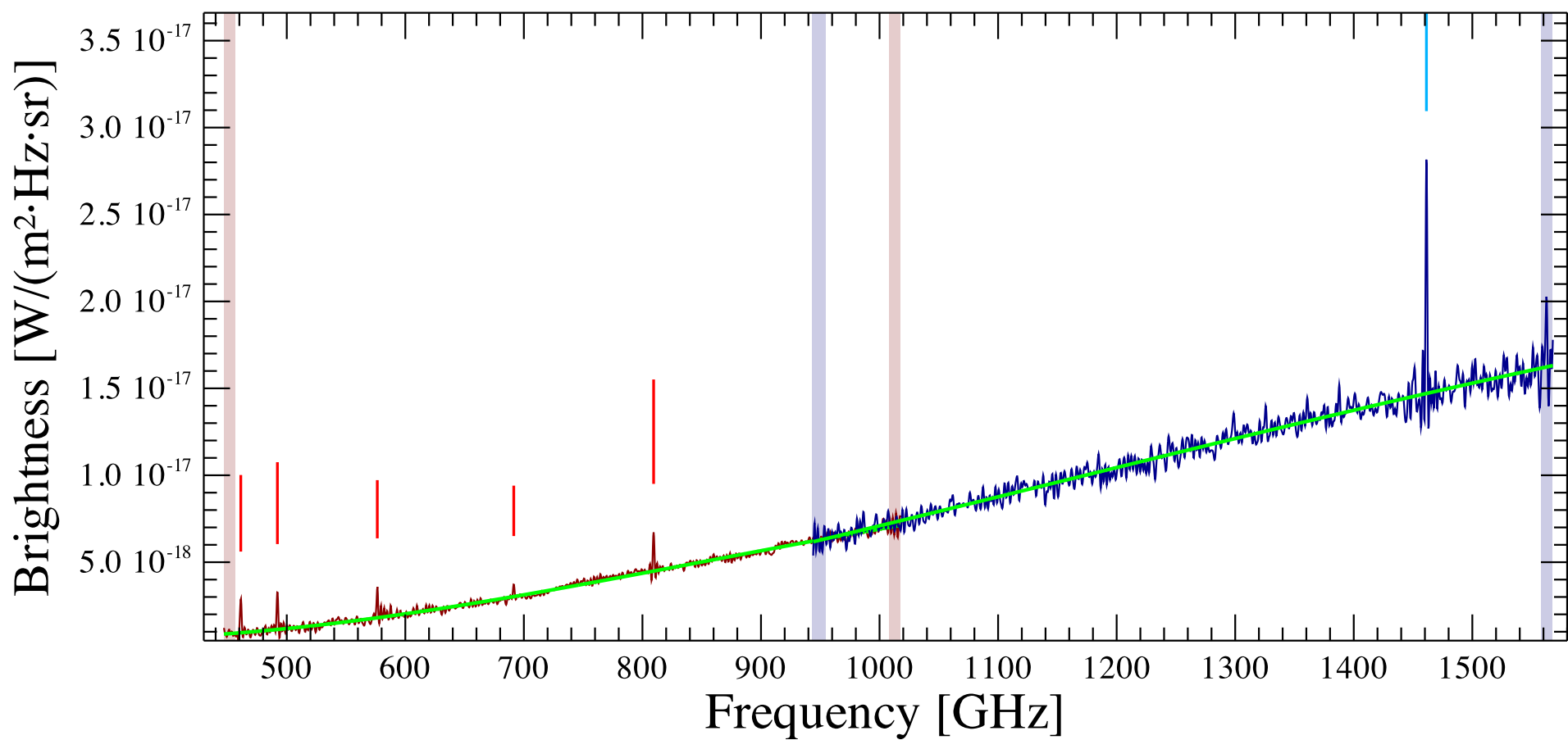
rcw120irs2 Observation ID 1342191229; (5/1)
