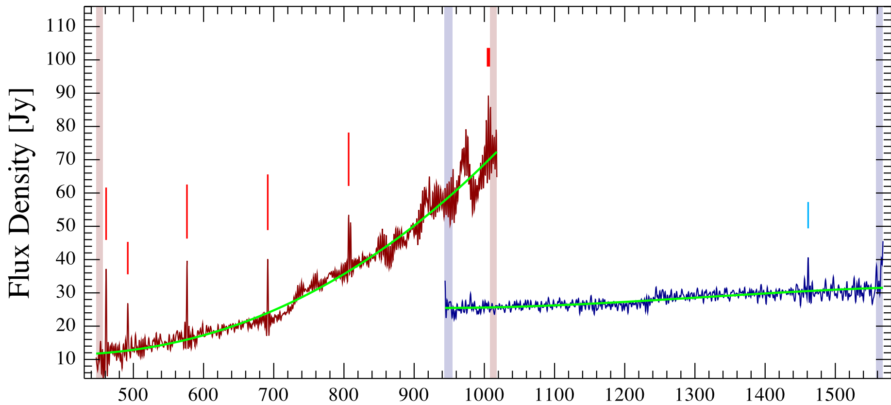
rcw120c8 Observation ID 1342191228; (8/1)
