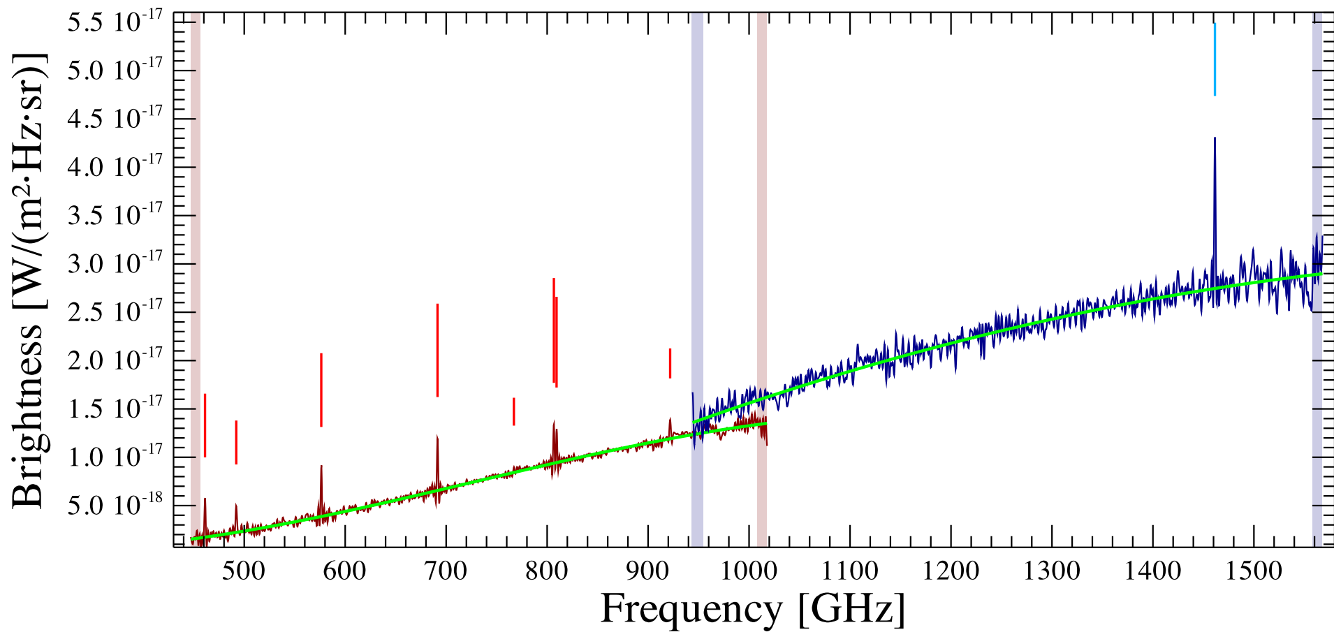
rcw120c8 Observation ID 1342191228; (8/1)
