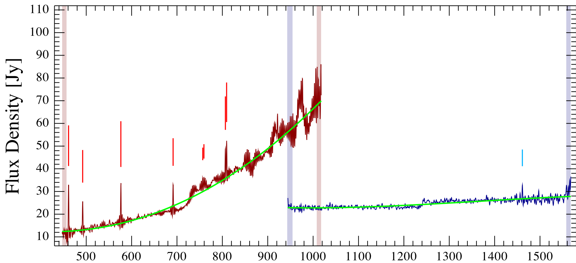
rcw120c6 Observation ID 1342191225; (10/1)
