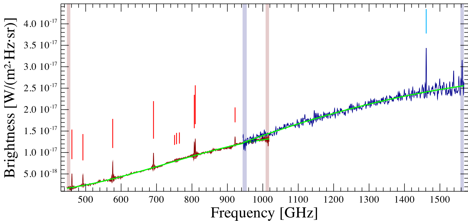
rcw120c6 Observation ID 1342191225; (10/1)
