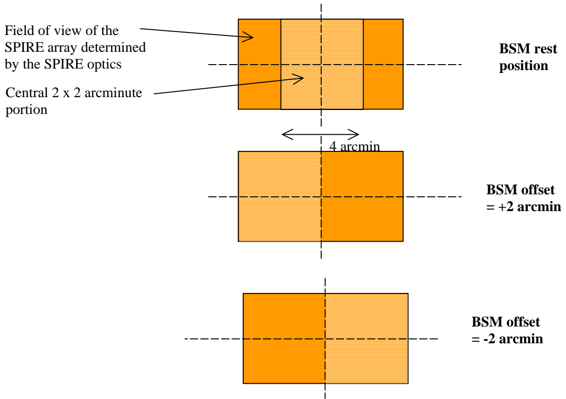
Figure 5.5: Field mapping with maximum chop throw of 4 arcminutes. The detectors in the central square 2 x 2 arcminute portion of a photometer array are deflected by \pm 2 arcminutes by the BSM, so that they are alternately chopped from one side of the available field of view to the other.
