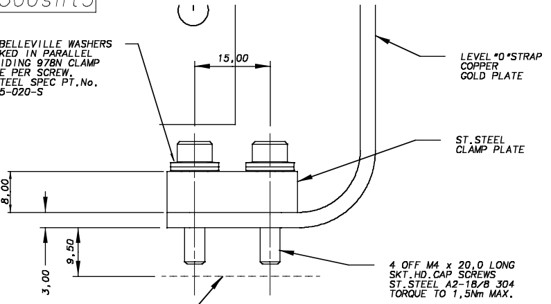
DETAIL "B" OF LEVEL "0" TO S/C INTERFACE SCALE 2:1
