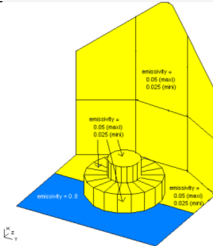
INCORPORER Figure 3.5-2/a: Thermal Interfaces (emissivities)
