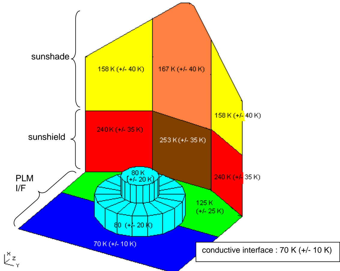
Figure 3.5-2/b: Thermal Interfaces (temperatures)
