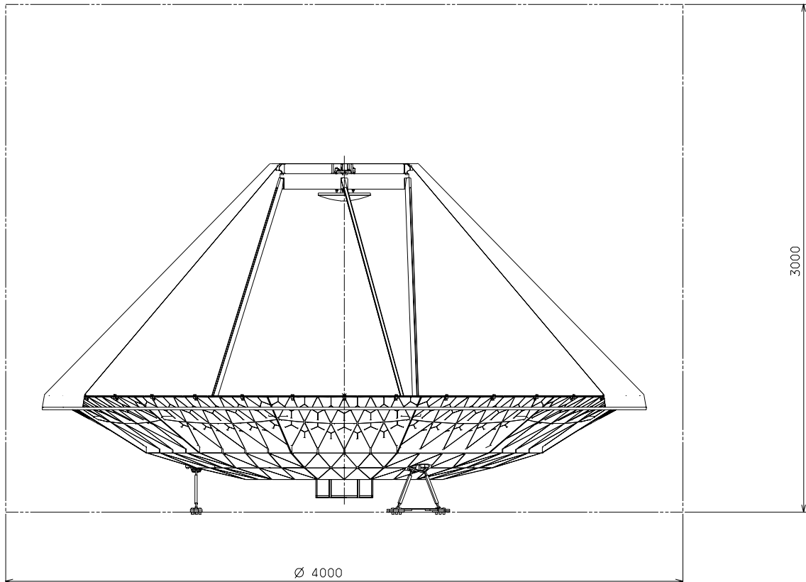
Figure 3.5-3: telescope hoisting device envelope (delimited by a cylinder \text{Ø}4000 , height 3000)
