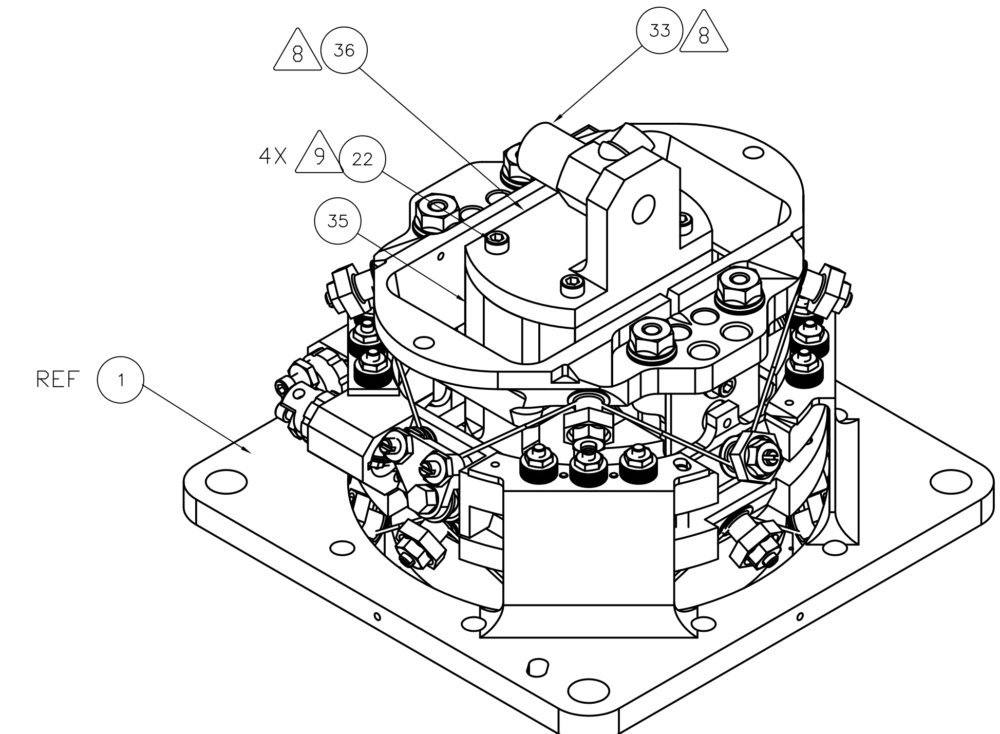
GENERAL VIEW REFERENCE ONLY SCALE: NONE -7 CONFIGURATION
