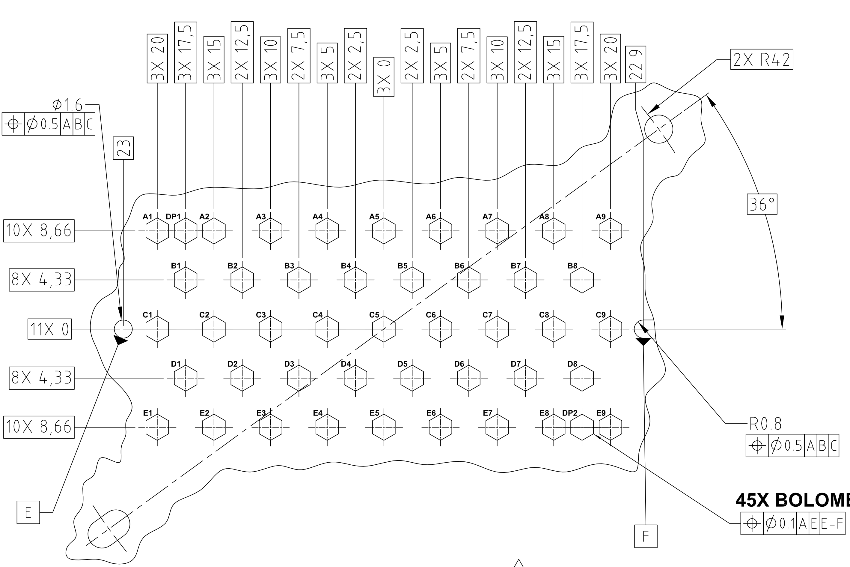
SECTION D-D PHOTOMETER LONG WAVE SCALE: 5:1
