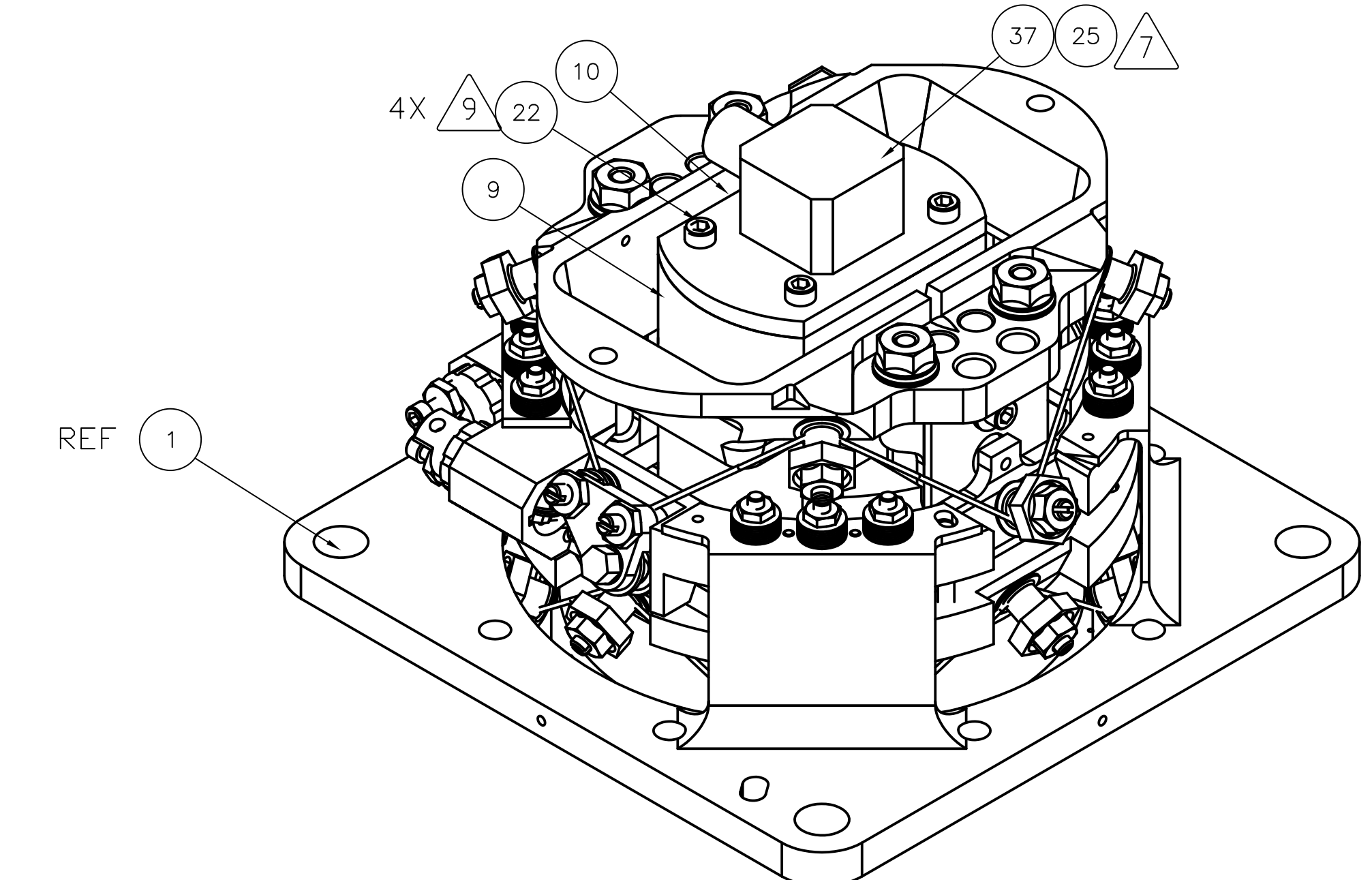
GENERAL VIEW REFERENCE ONLY SCALE: NONE -6 CONFIGURATION
