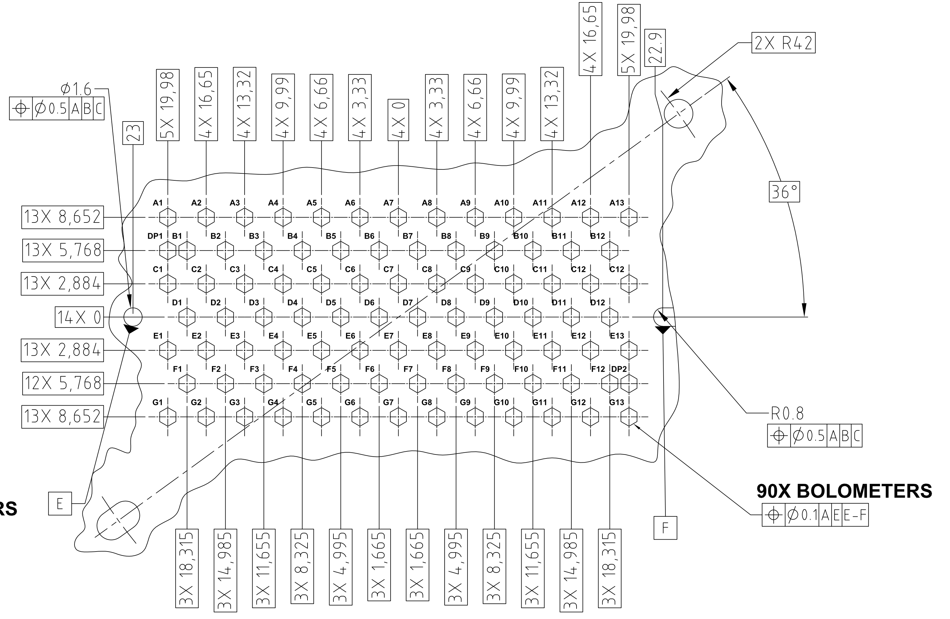
SECTION E-E PHOTOMETER MEDIUM WAVE SCALE: 5:1
