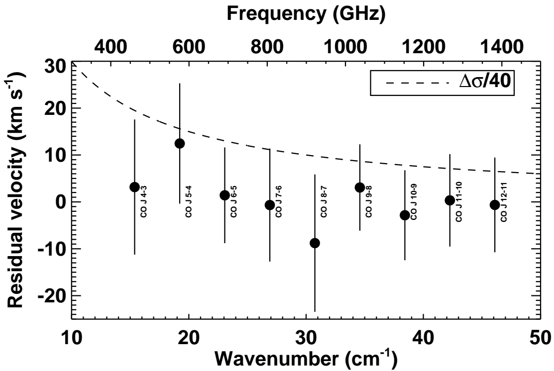
Figure 3: Residual velocity of the CO lines in the OD302 Orion observations. The dashed line shows the spectral resolution, divided by 40, converted into velocity units.
