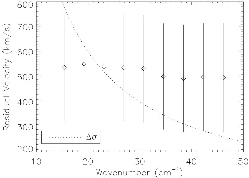
Figure 2: Residual velocity of the CO lines in the OD302 Orion observations prior to obliquity correction. The dashed line shows the spectral resolution, converted into velocity units.
