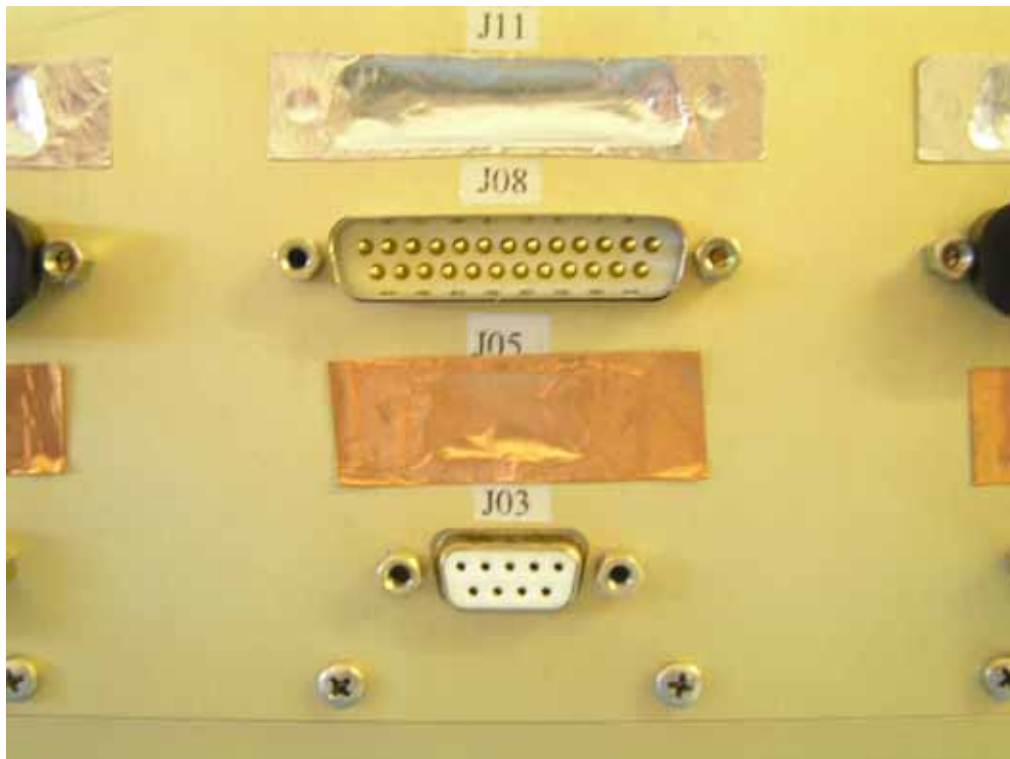
View to show connectors J11, J08, J05, J03
