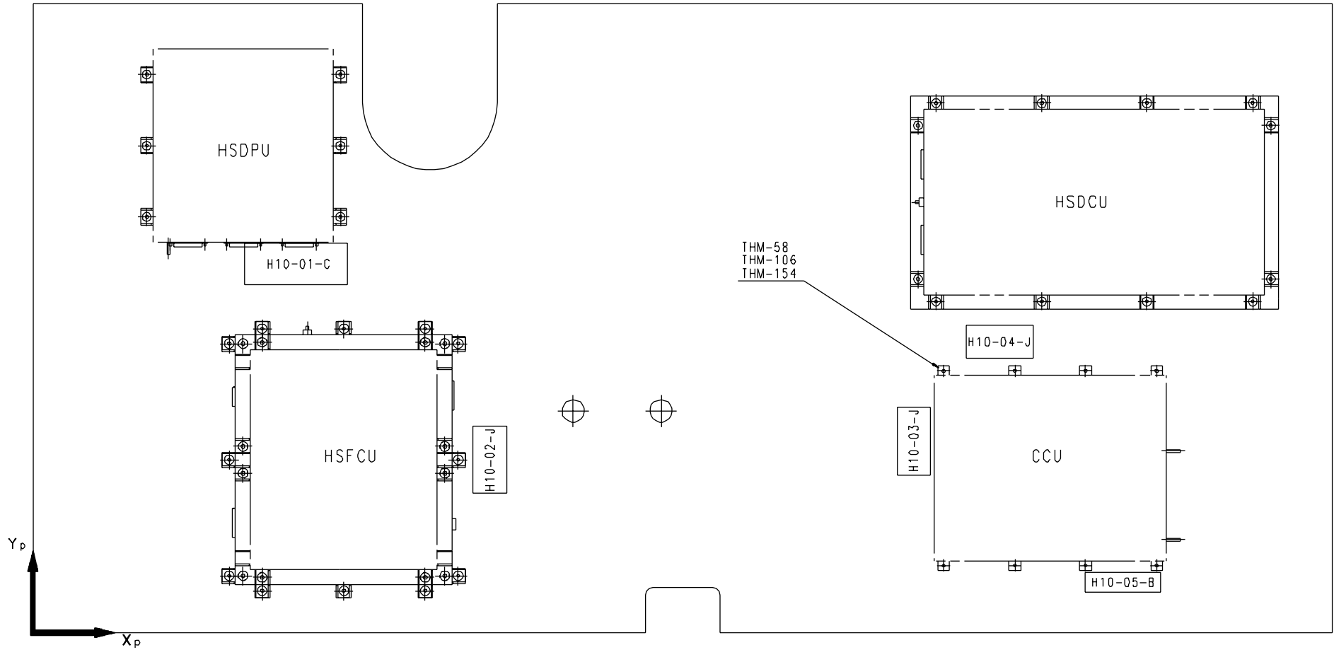
Figure 3.1.1-4 HERSCHEL –Z Panel (SPIRE)
