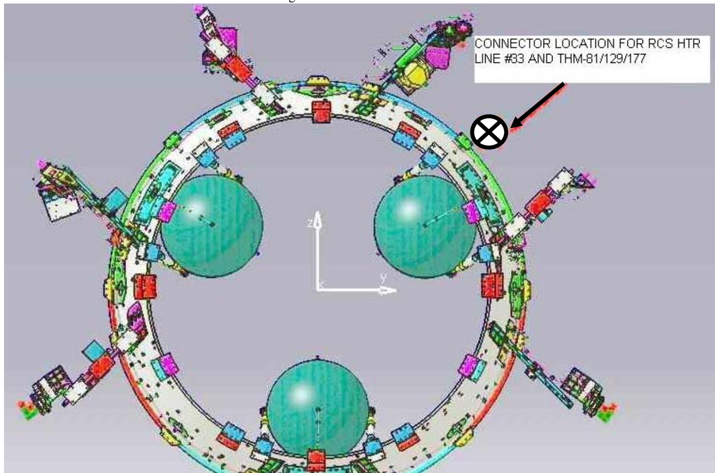
Figure 3.1.2-14b PLANCK RCS
