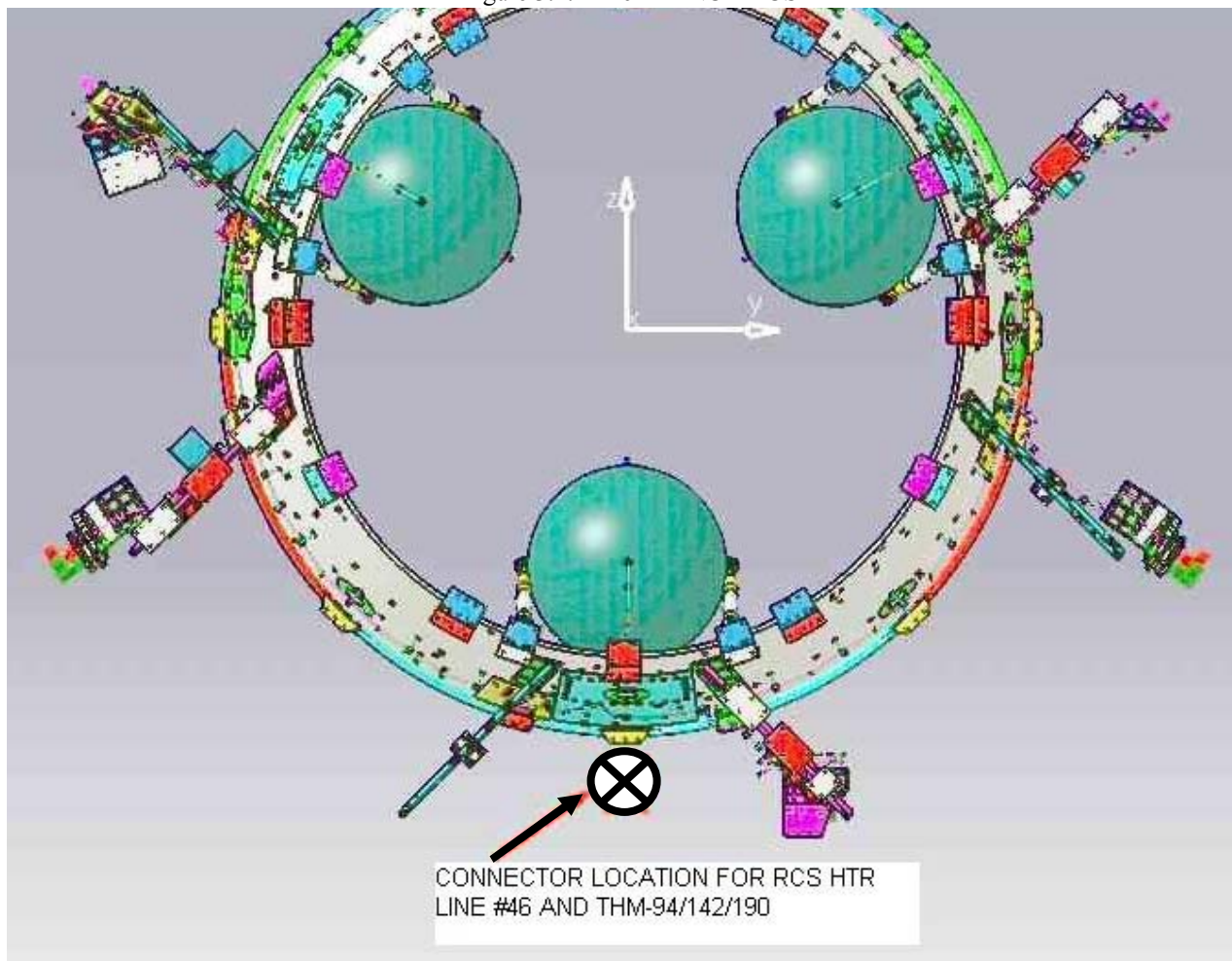
Figure 3.1.2-14c PLANCK RCS
