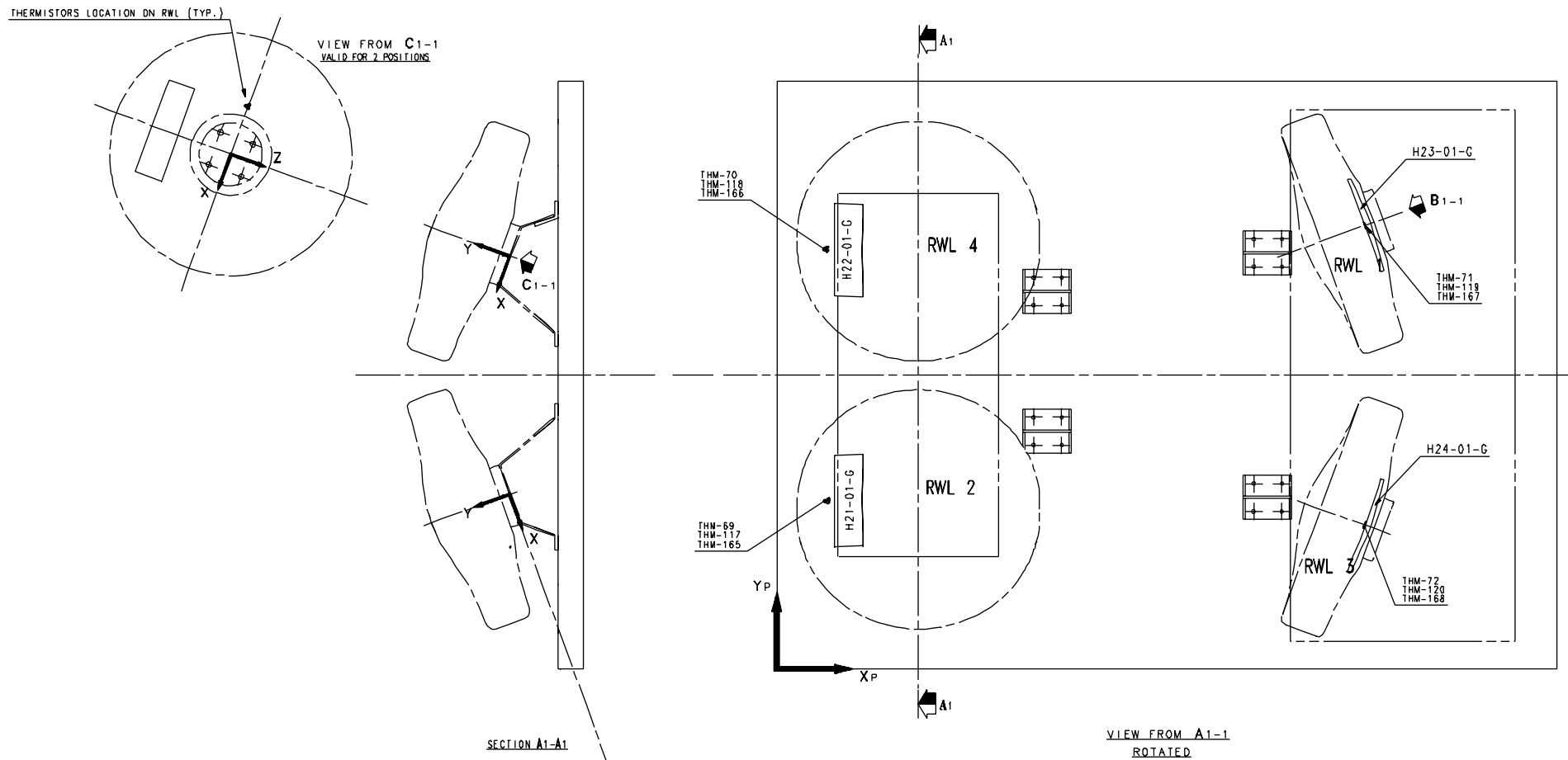
Figure 3.1.1-7 HERSCHEL -Y+Z Panel (RWL)
