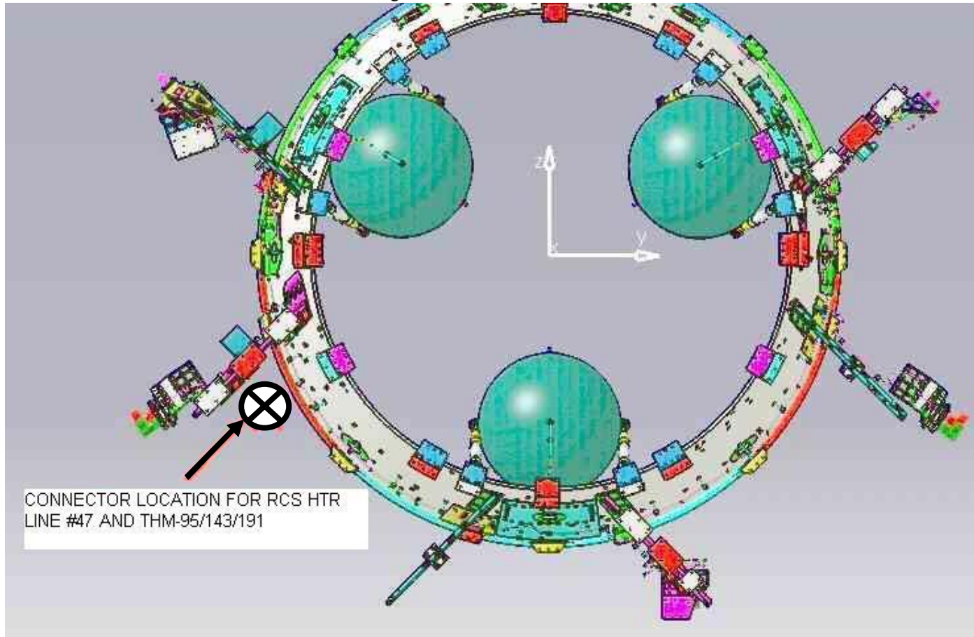
Figure 3.1.2-14d PLANCK RCS
