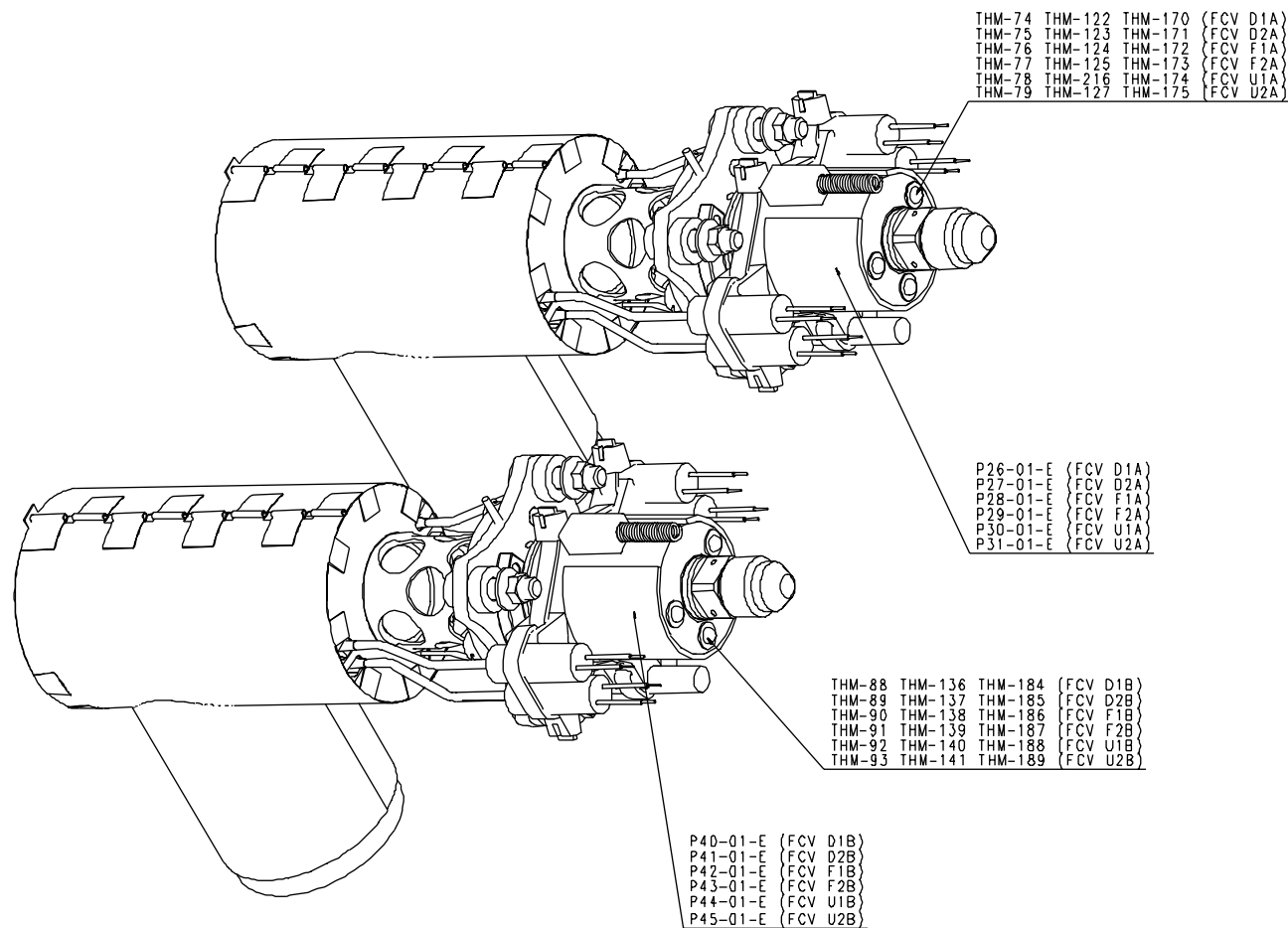
Figure 3.1.2-7a PLANCK Lower Thruster (20 N)
