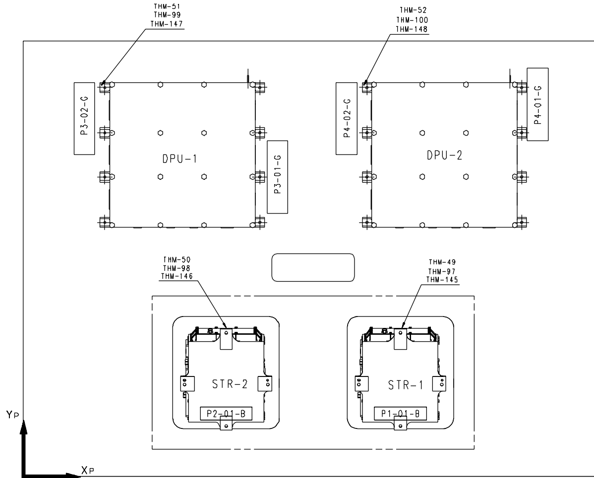
Figure 3.1.2-1 PLANCK +Z Panel
