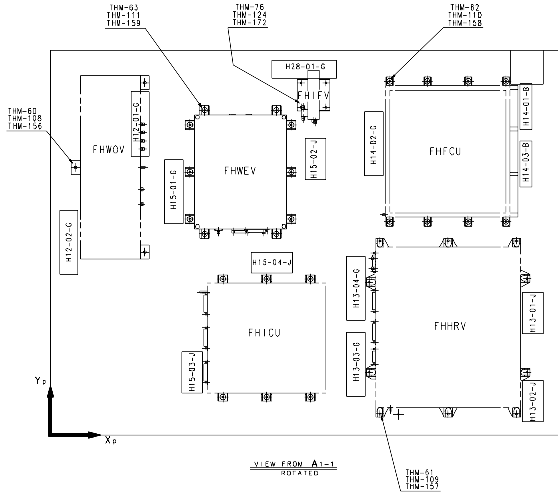
Figure 3.1.1-5 HERSCHEL -Y-Z Panel (HIFI 2)
