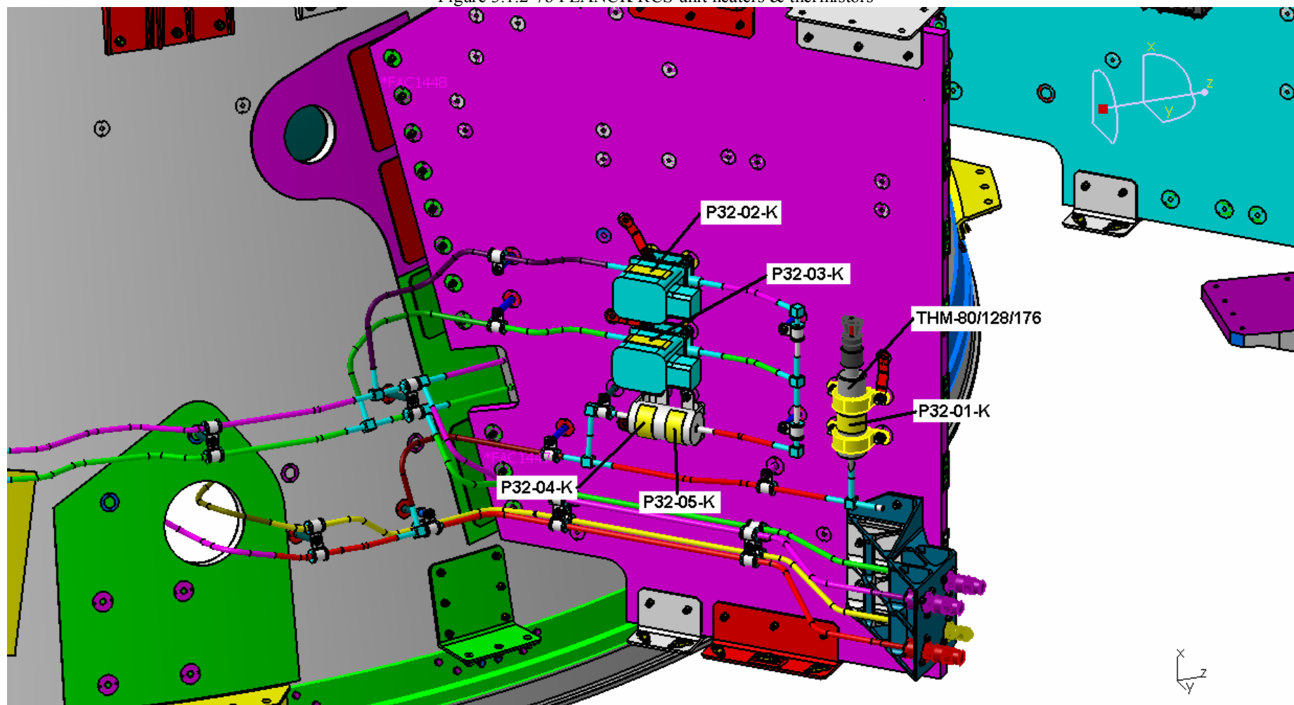
Figure 3.1.2-7b PLANCK RCS unit heaters & thermistors
