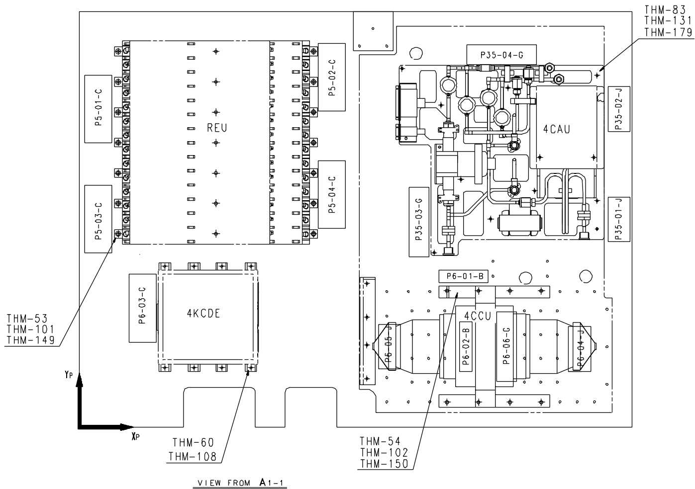
Figure 3.1.2-2 PLANCK +Y Panel
