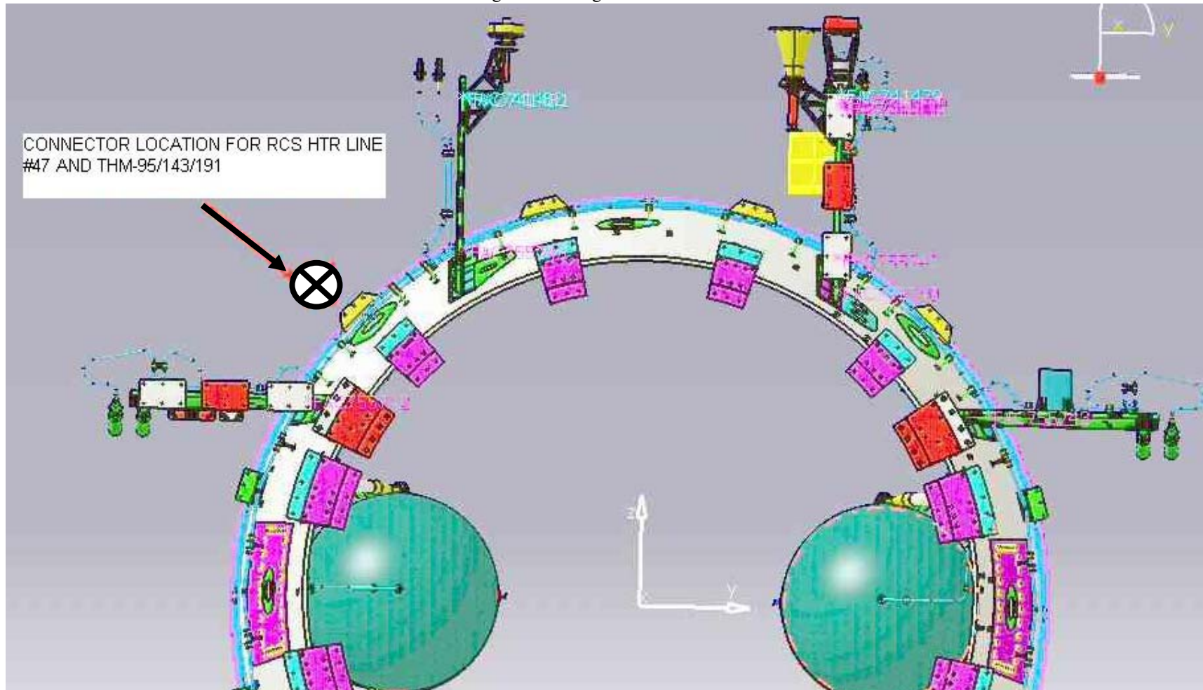
Figure 3.1.1-11g HERSCHEL RCS
