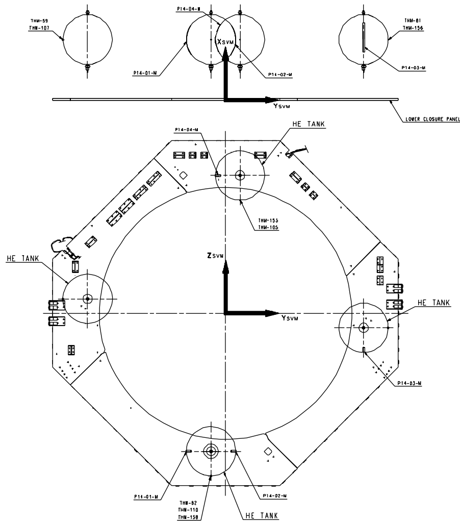
Figure 3.1.2-15 PLANCK Helium Tanks
