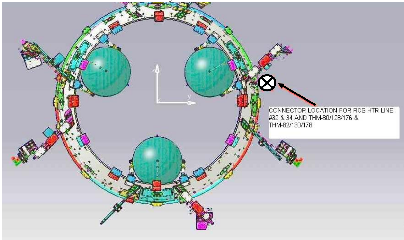
Figure 3.1.2-14a PLANCK RCS
