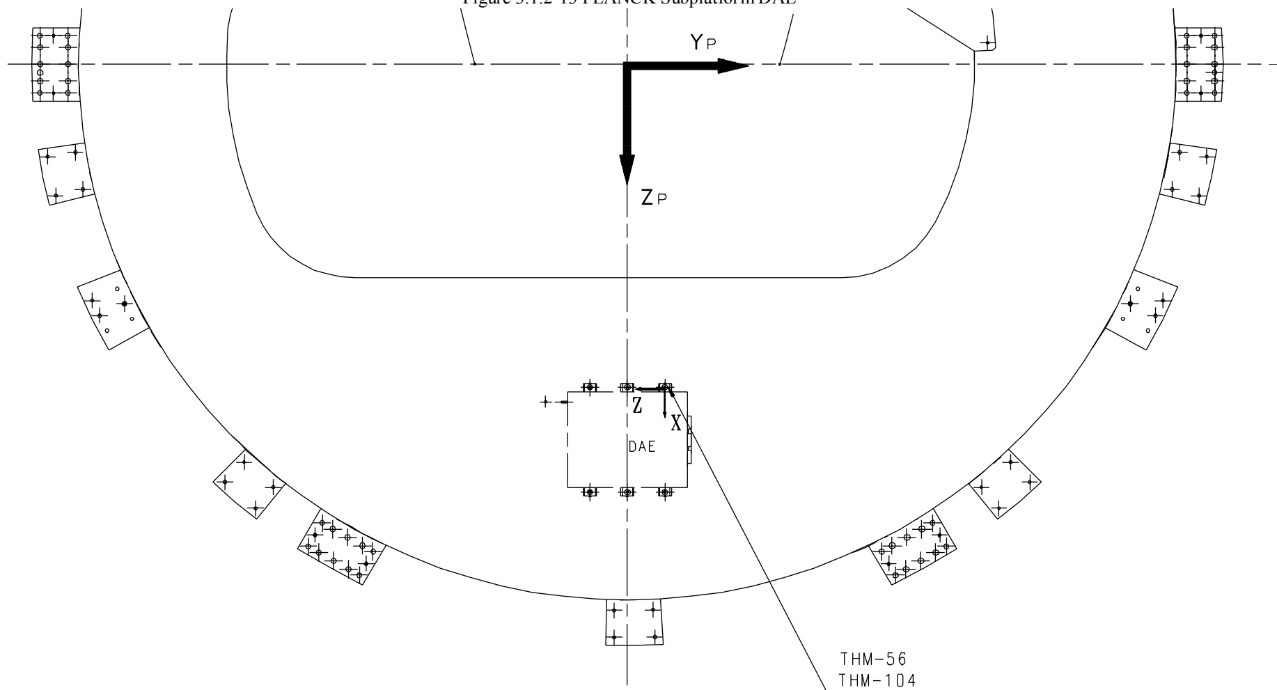
Figure 3.1.2-13 PLANCK Subplatform DAE
