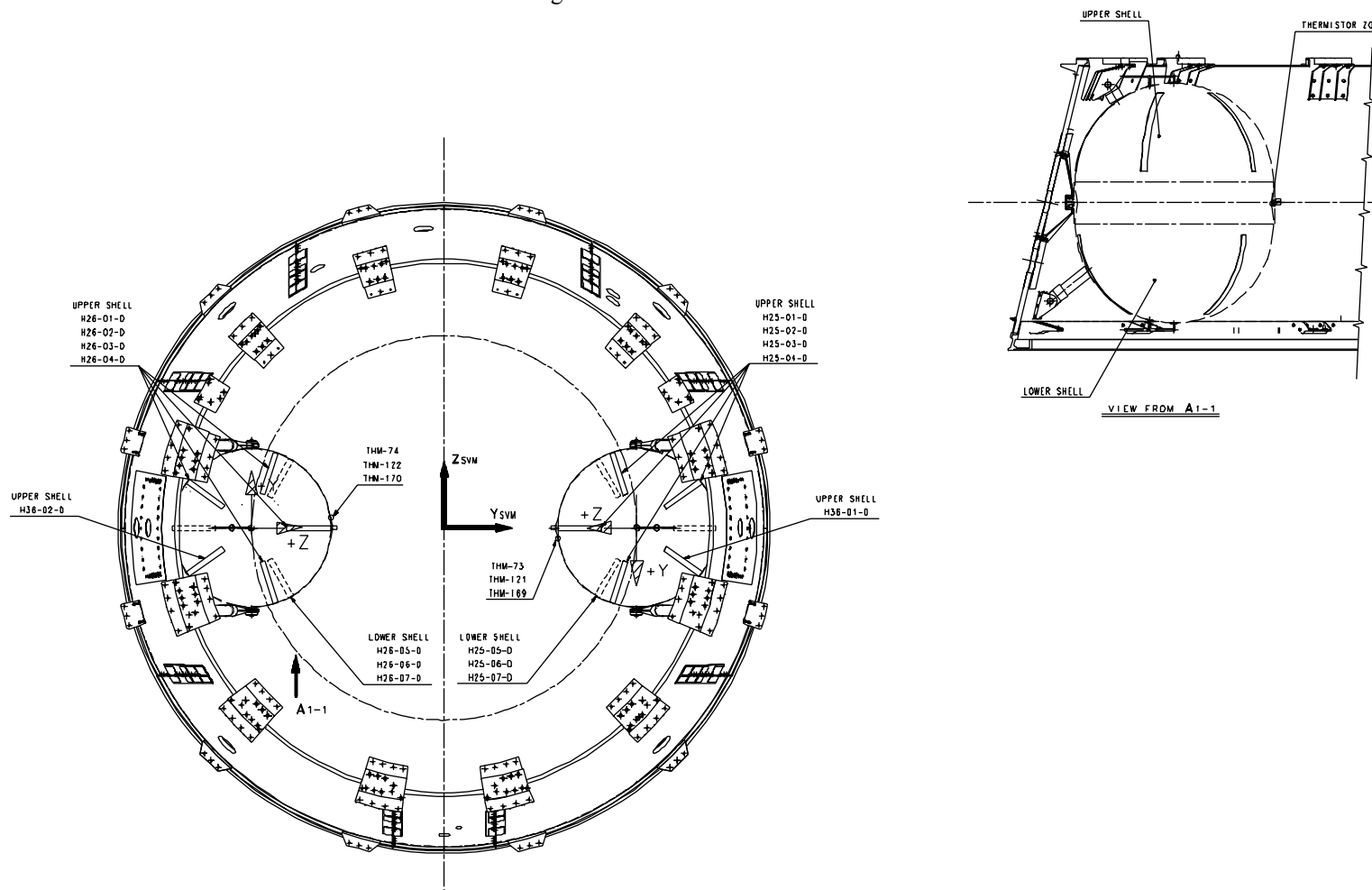
Figure 3.1.1-8 HERSCHEL Tanks
