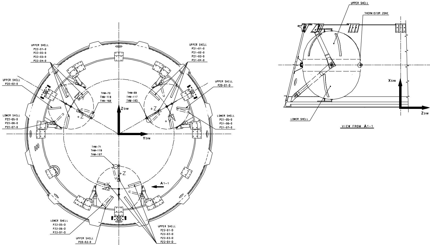
Figure 3.1.2-5 PLANCK Tanks
