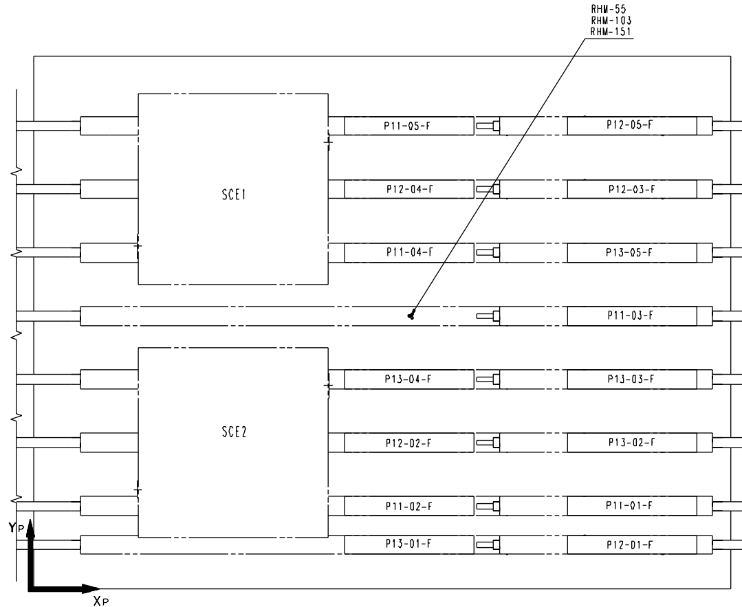
Figure 3.1.2-9 PLANCK Heat Pipes
