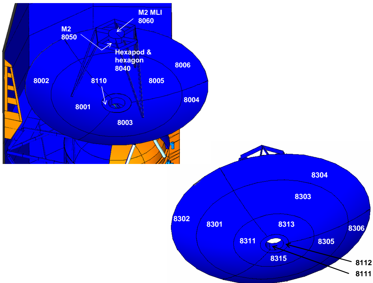
Figure 4.8-4: Telescope GMM
