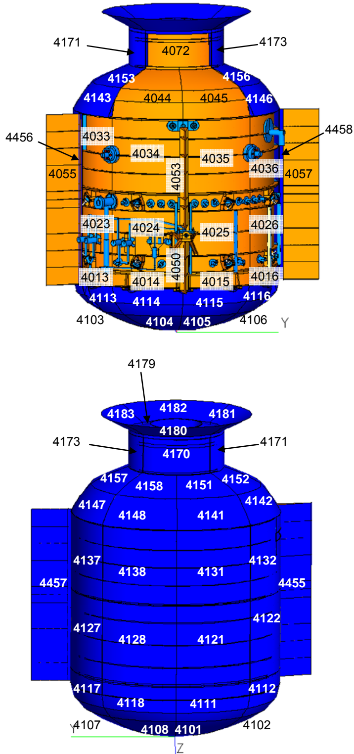
Figure 4.7-1: CVV Radiator and MLI Nodal Break-Down
