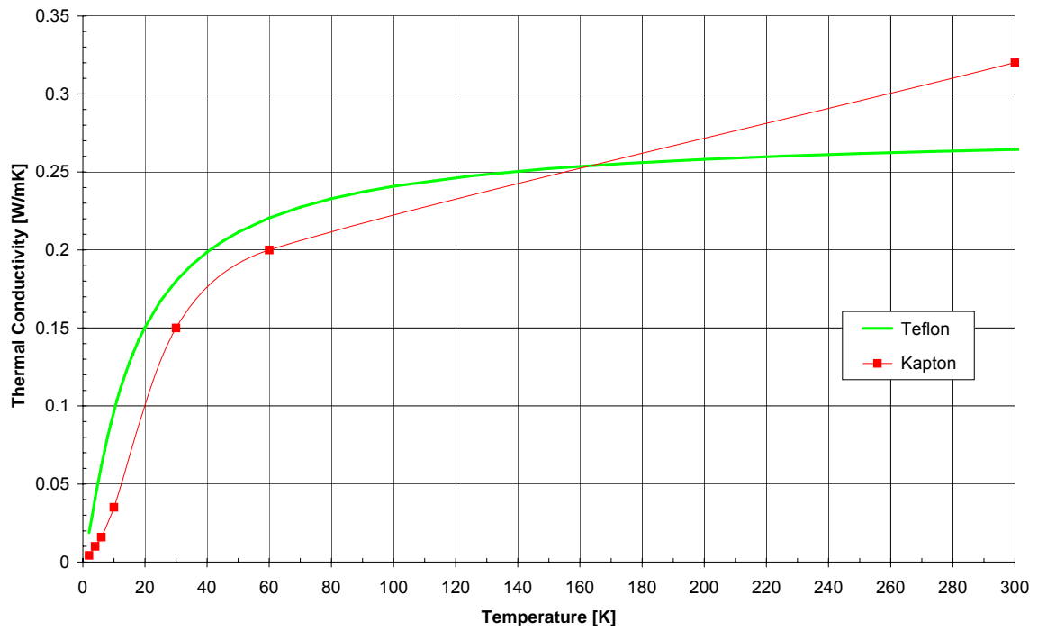
Figure 5.2-7: Thermal Conductivity of Harness Wire Insulation Materials /14/
