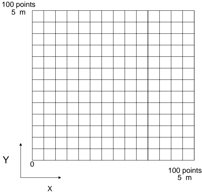
Figure 15-5 : CATR Quiet zone measurement : acquisition grid
