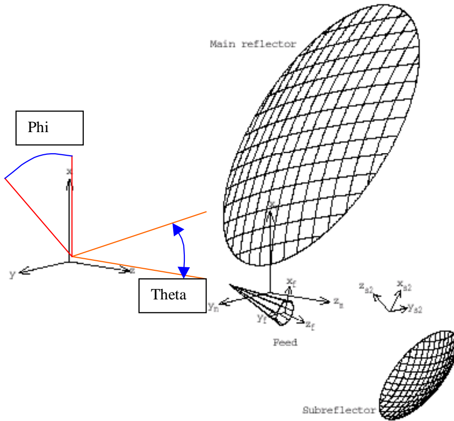
Figure 5-1 : axis convention
