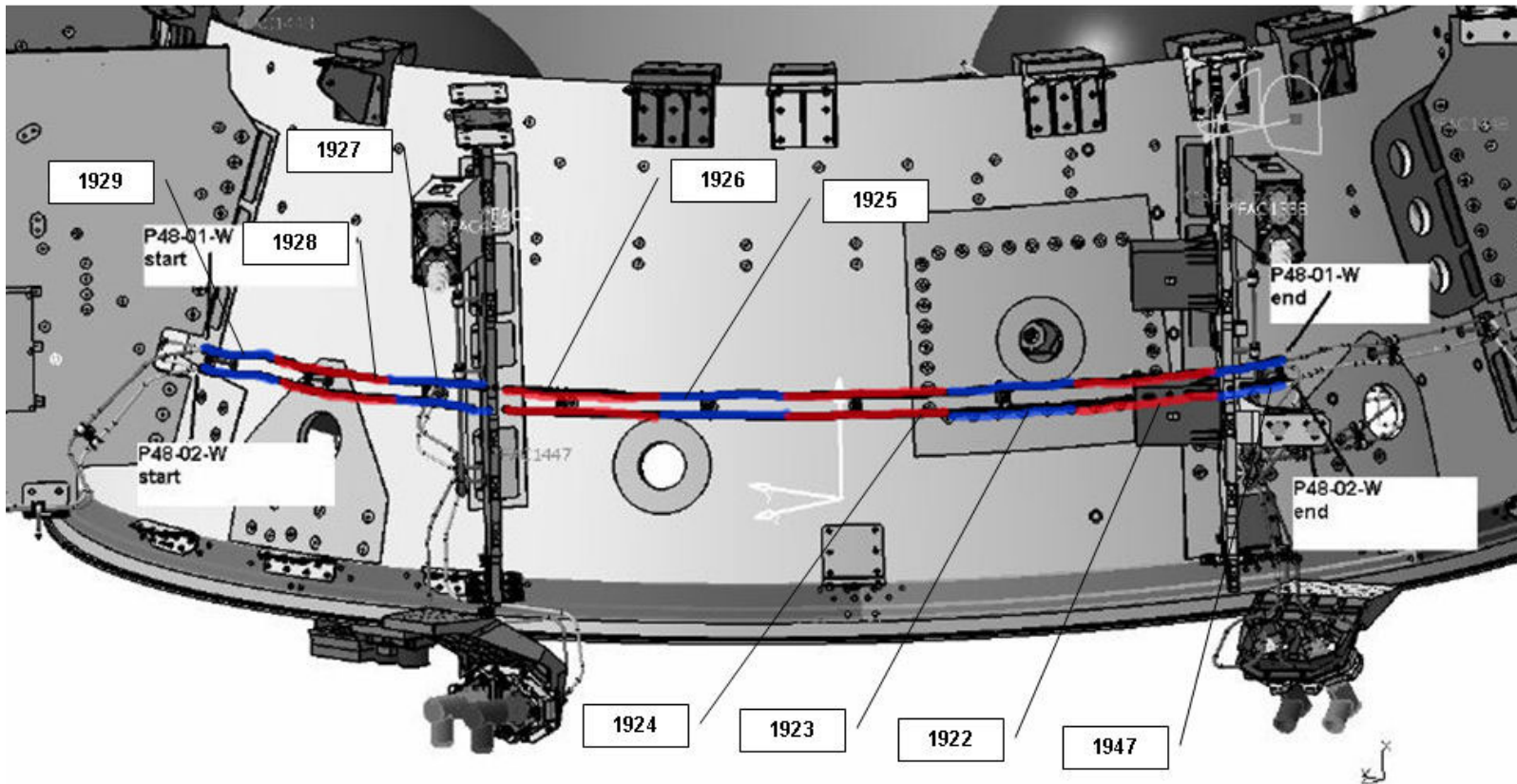
Figure 4.1.4-22 PLANCK - RCS Line #48
