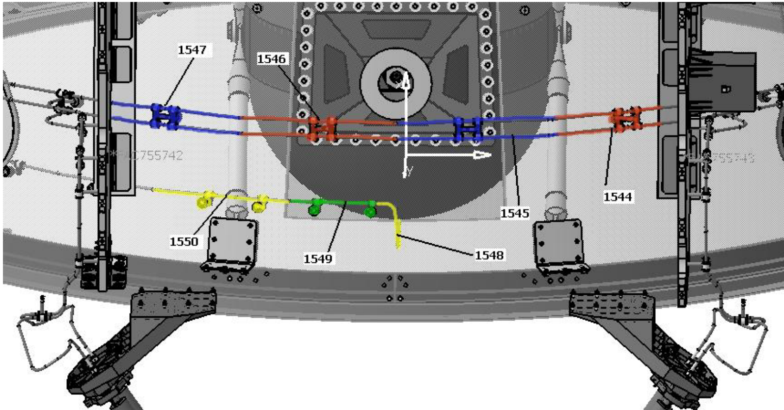
Figure 3.1.4-5 HERSHEL – RCS line11
