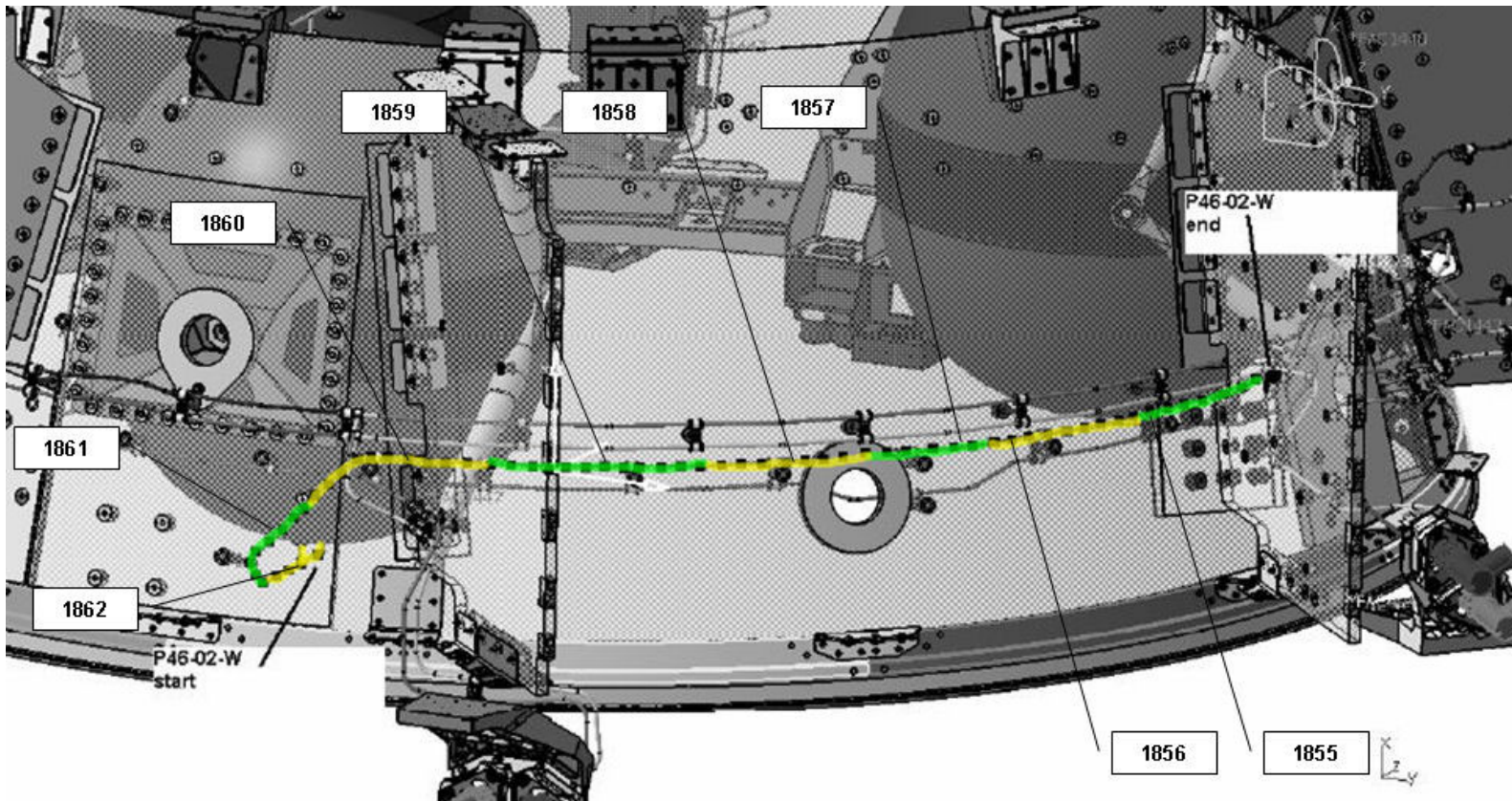
Figure 4.1.4-12 PLANCK - RCS Line #46
