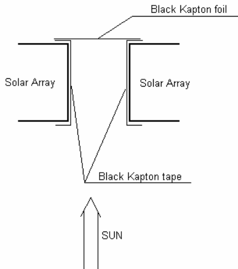
Figure 8.5.4.5-1 PLANCK – Sun trapping
