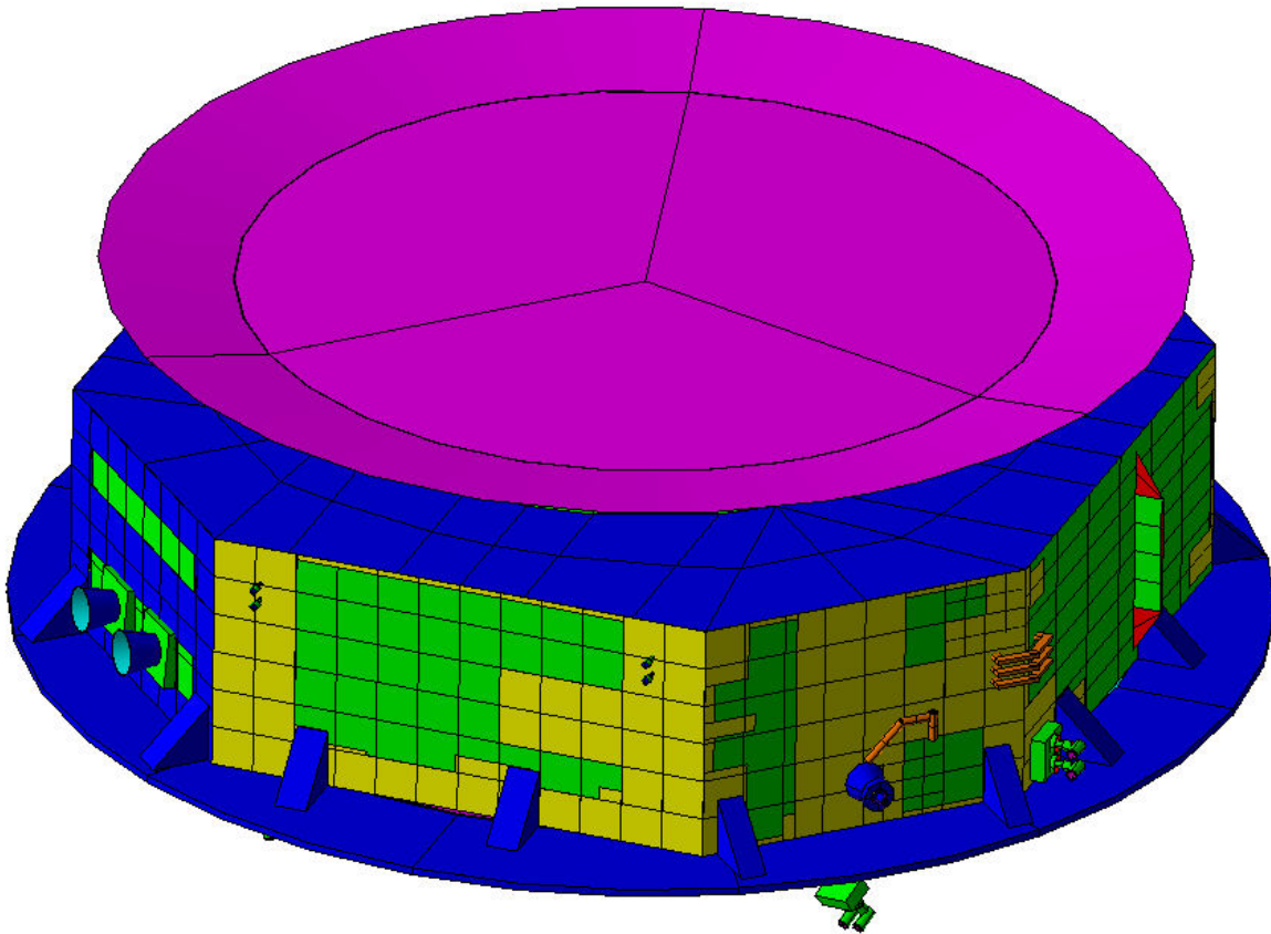
Figure 4-1 PLANCK - Overall view
