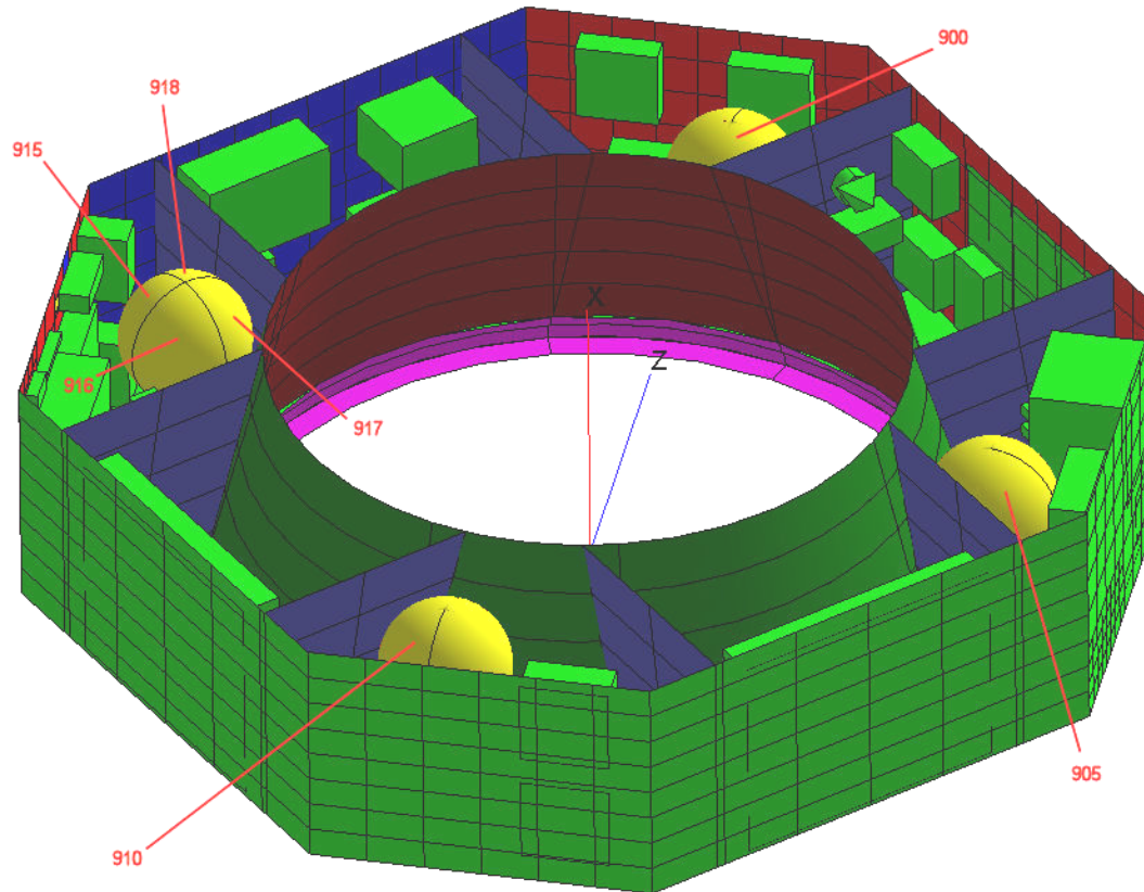
Figure 4.1.2-2 PLANCK He Tanks
