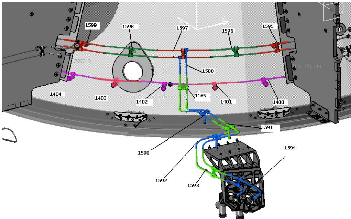
Figure 3.1.4-8 HERSCHEL – RCS line37-45
