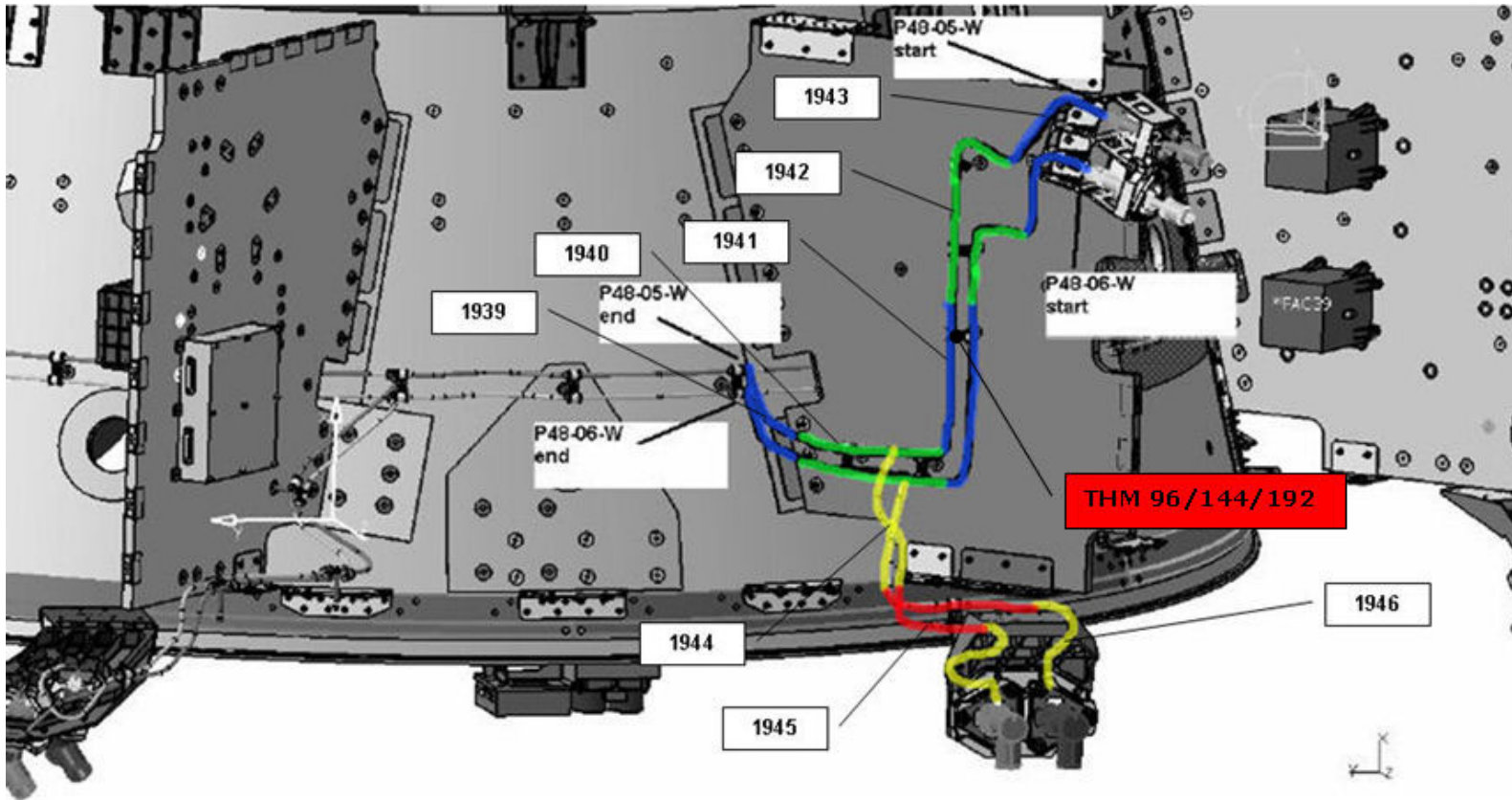
Figure 4.1.4-25 PLANCK - RCS Line #48
