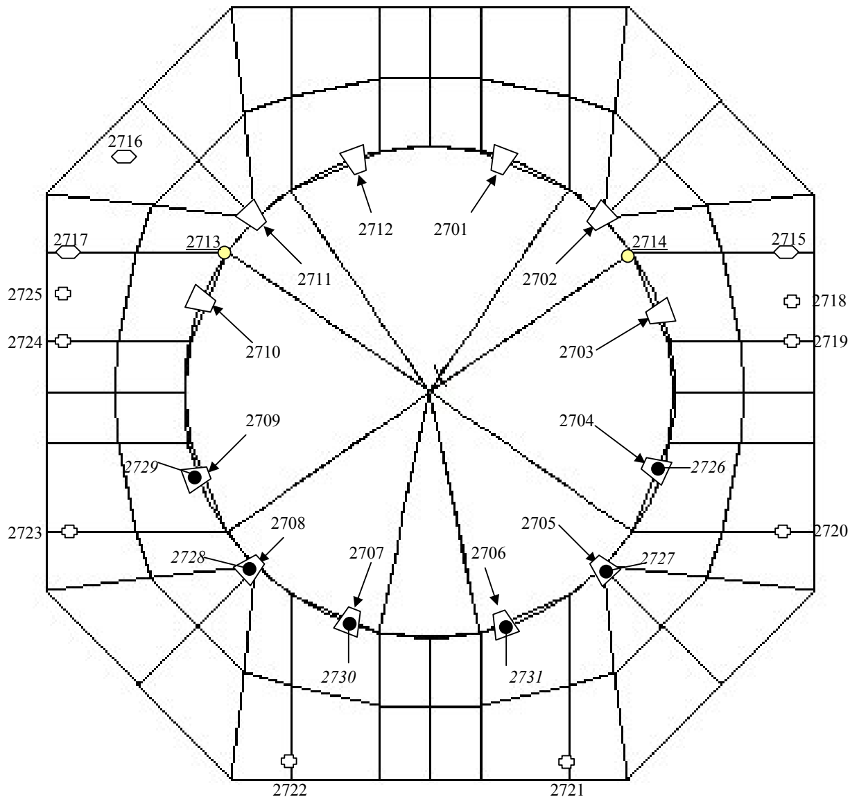
Figure 3.1.7-1 HERSCHEL – I/F points with PLM
