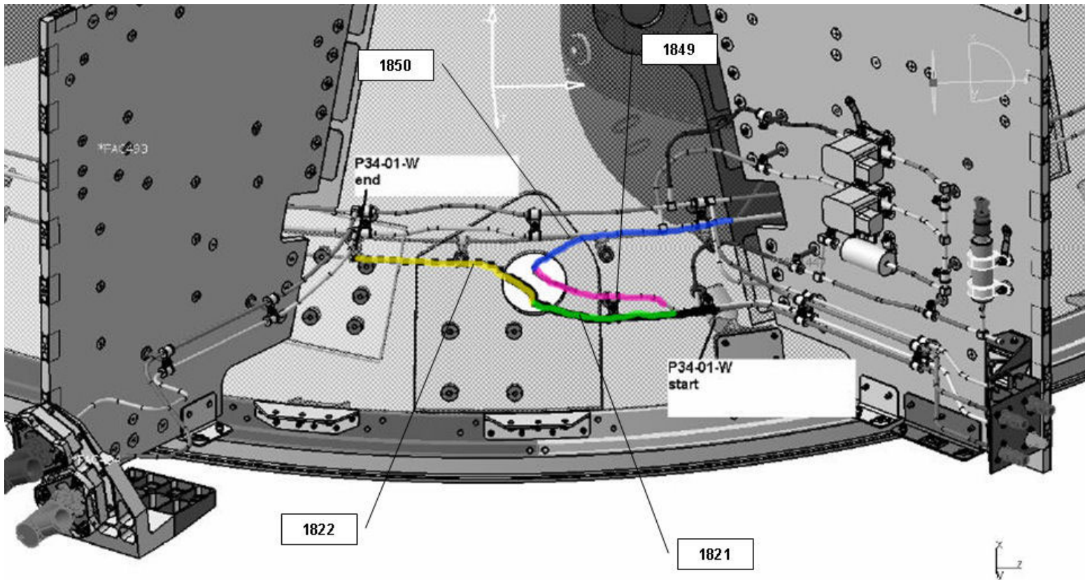
Figure 4.1.4-6 PLANCK - RCS Line #34
