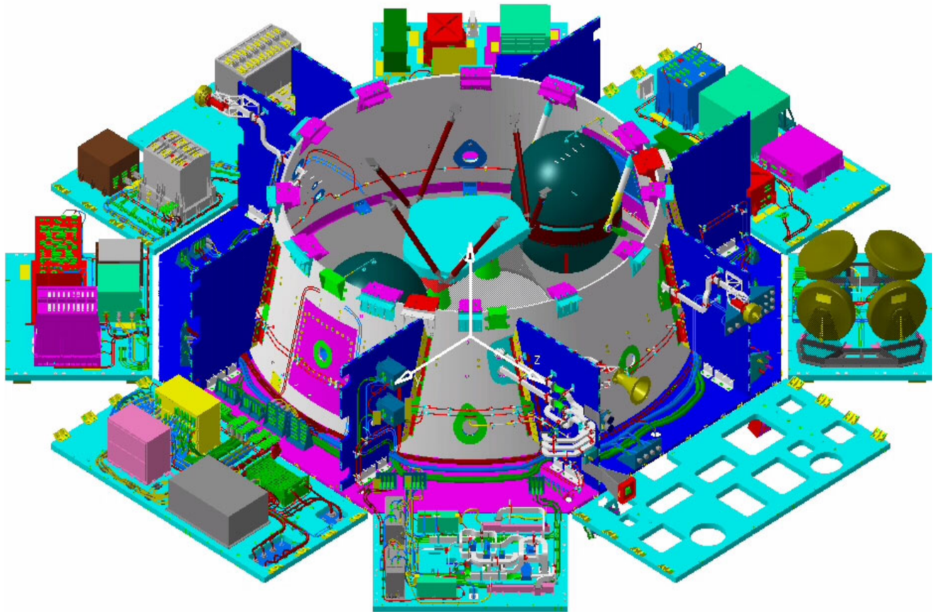
Figure 3-3 HERSCHEL – Internal overall View
