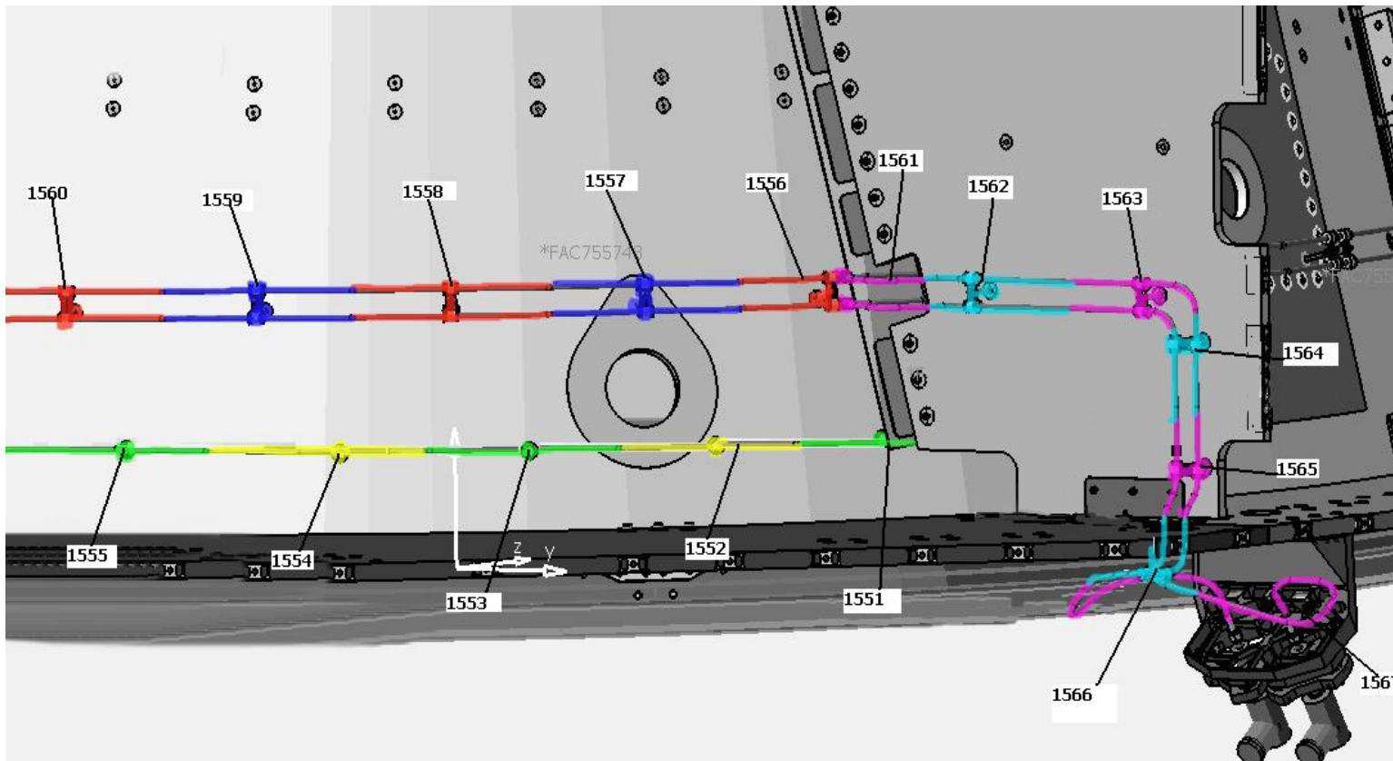
Figure 3.1.4-6 HERSHEL – RCS line35
