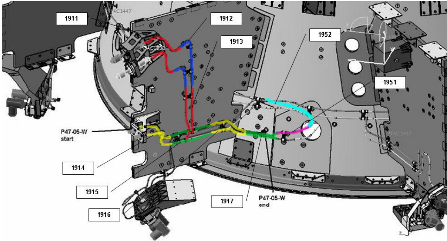
Figure 4.1.4-20 PLANCK - RCS Line #47
