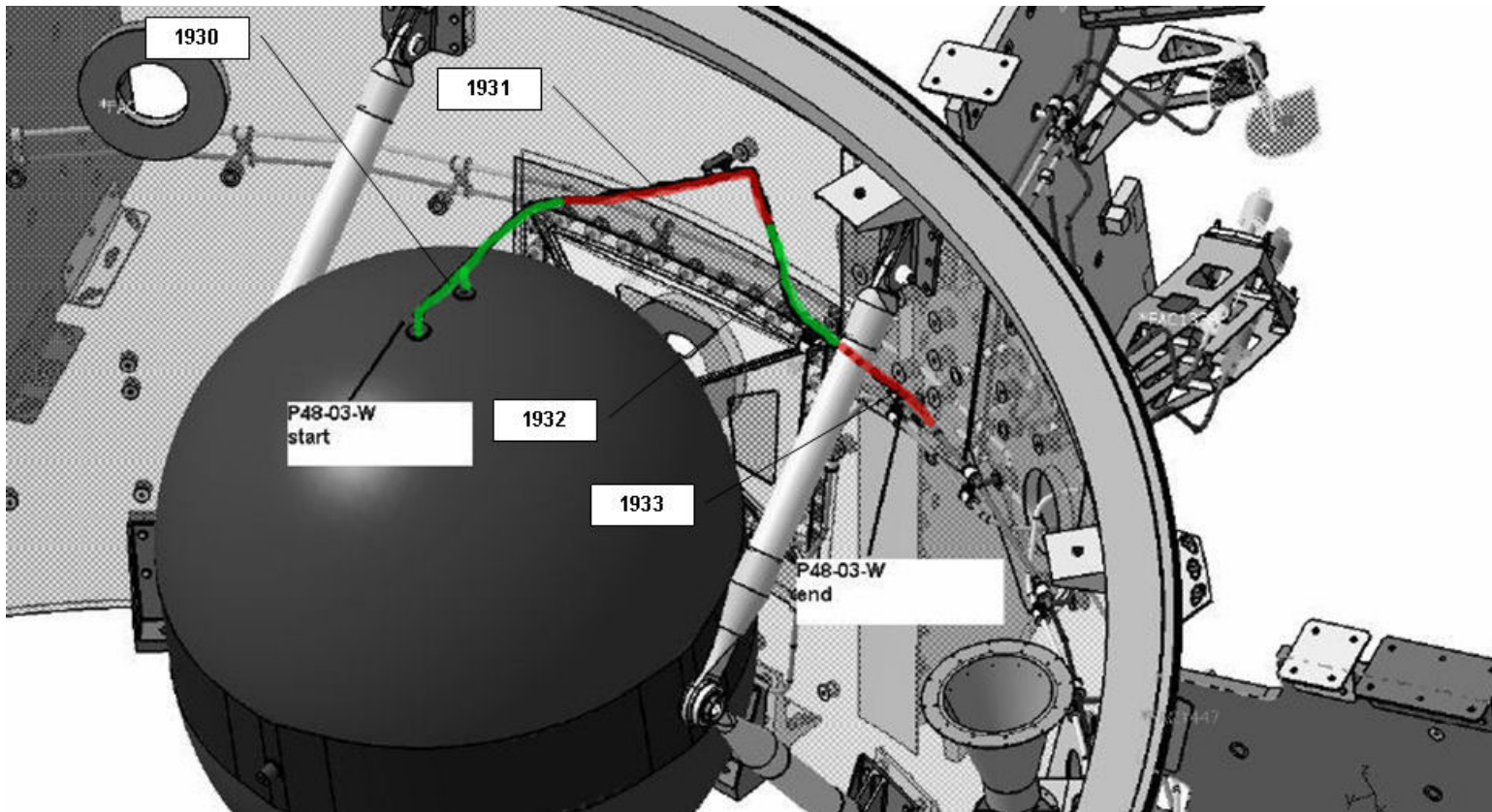
Figure 4.1.4-23 PLANCK - RCS Line #48
