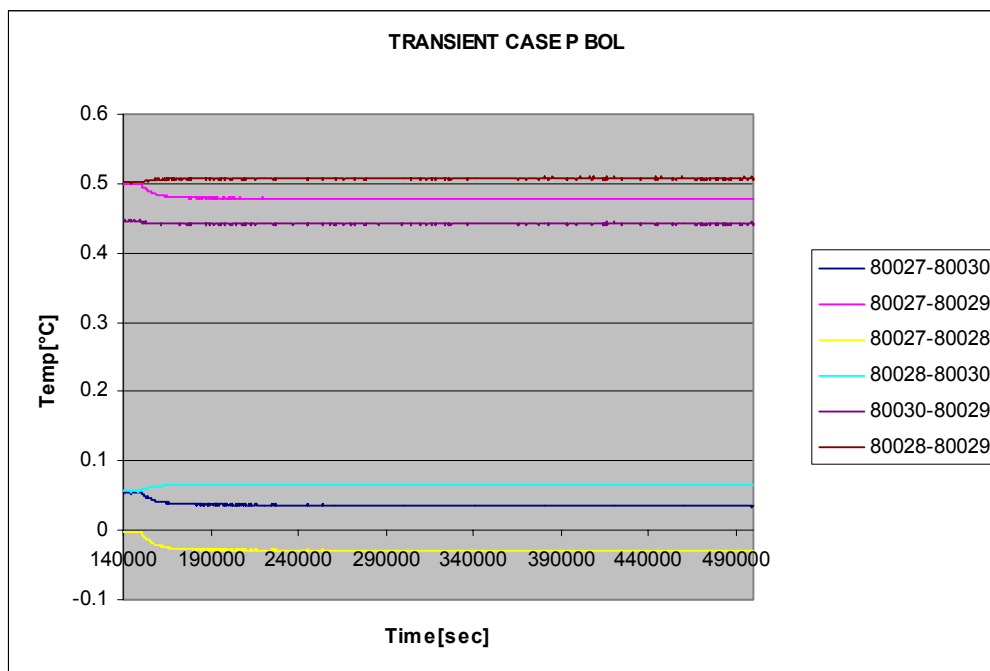
Figure 7.1-1 HERSCHEL STR feet temperature gradient (COLD CASE P)
