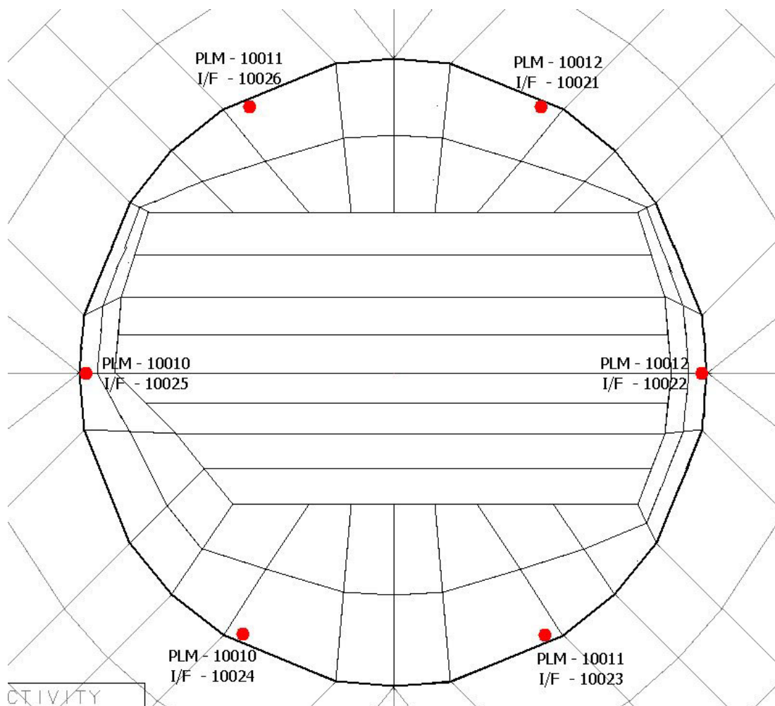
Figure 4.1.7-1 PLANCK - PLM I/F attachment points
