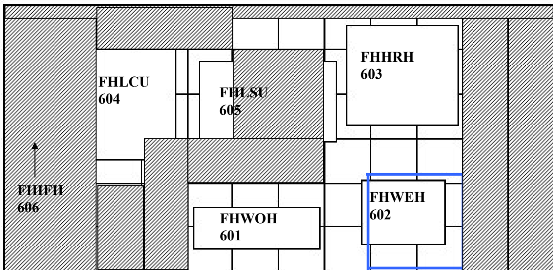
Figure 3.1.1-2f HERSHEL - -Y MLI Lateral Panel & Units Internal View
