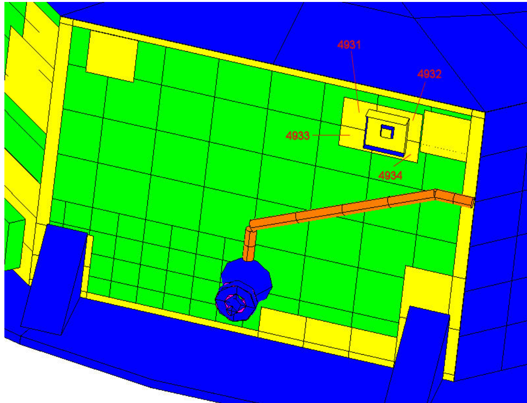
Figure 4.1.1-6 PLANCK +Y external panel new GMM nodes
