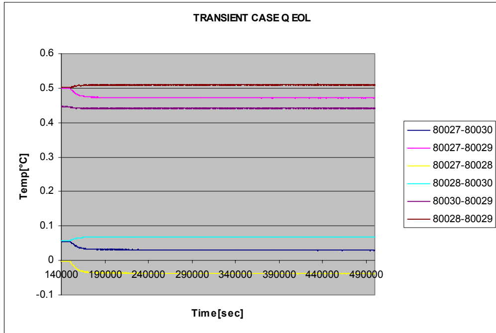
Figure 7.1-2 HERSCHEL STR feet temperature gradient (HOT CASE Q)
