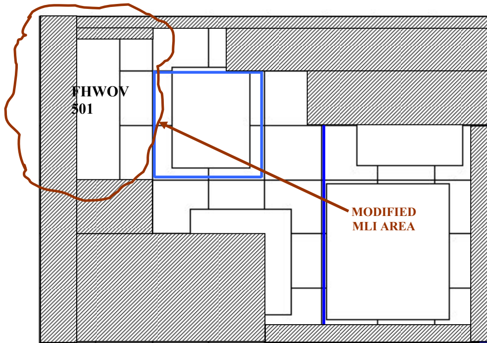
Figure 3.1.1-: HERSHEL - -Y -Z MLI Lateral Panel & Units Internal View according to [AD31]
