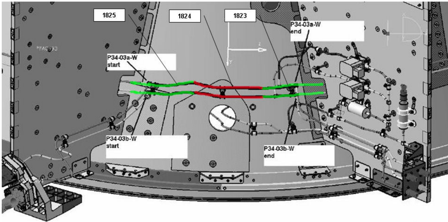
Figure 4.1.4-7 PLANCK - RCS Line #34
