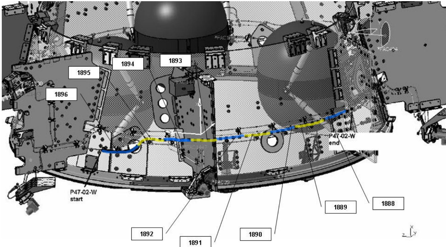
Figure 4.1.4-17 PLANCK - RCS Line #47
