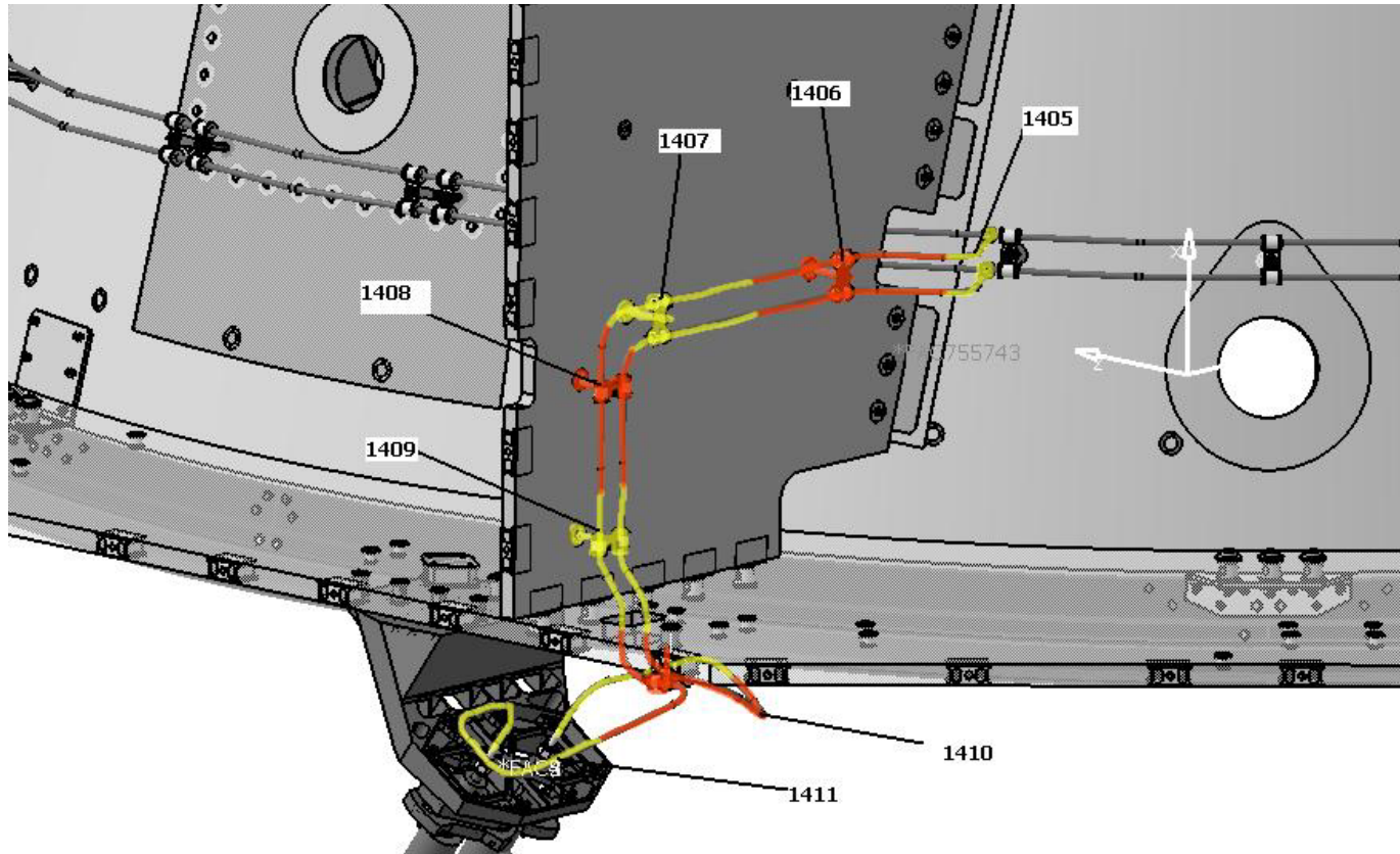
Figure 3.1.4-9 HERSCHEL – RCS line45
