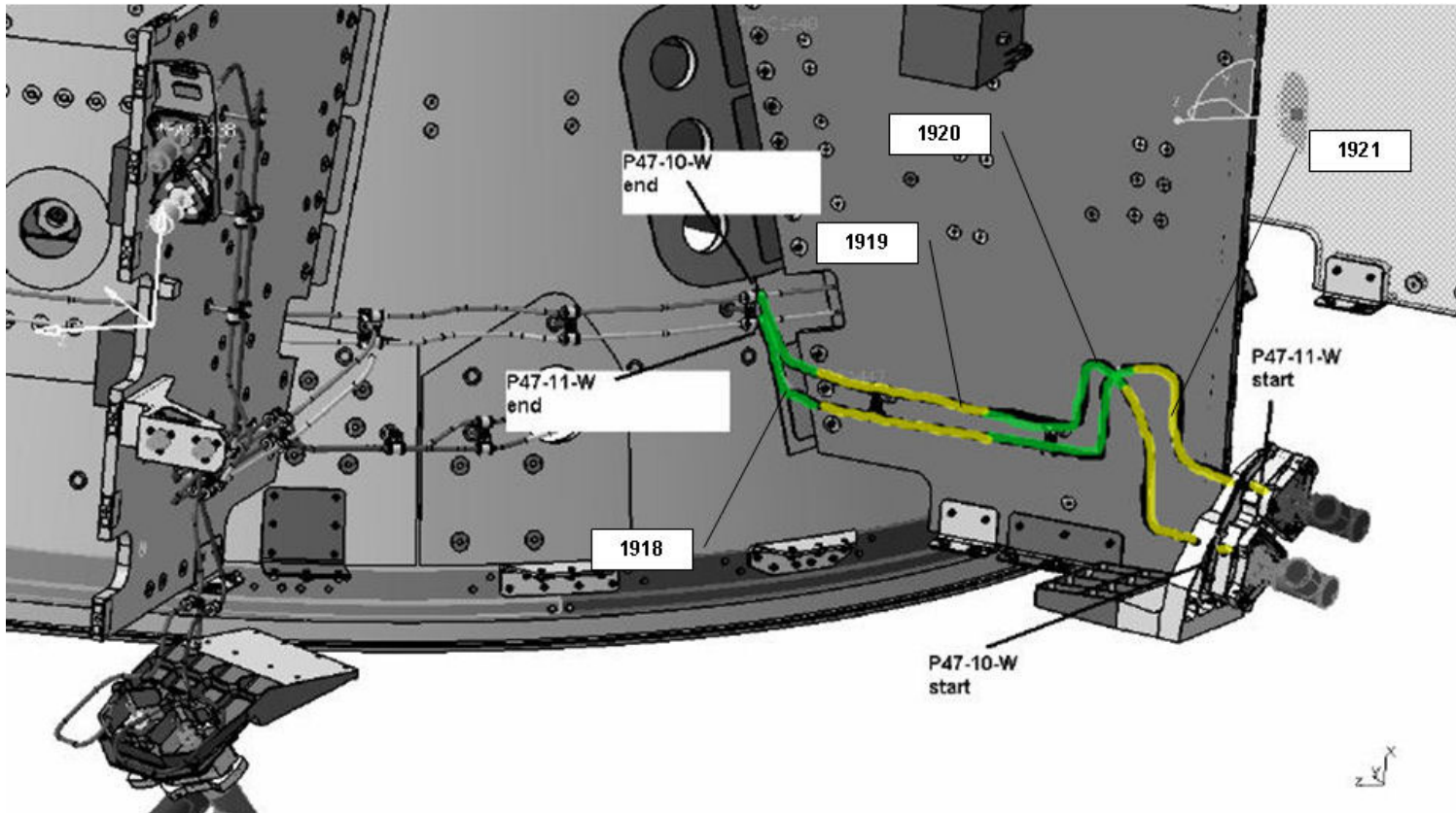
Figure 4.1.4-21 PLANCK - RCS Line #47
