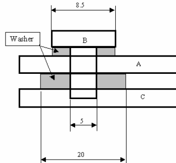
Figure 5.7-1 PLANCK – Connection via screw
