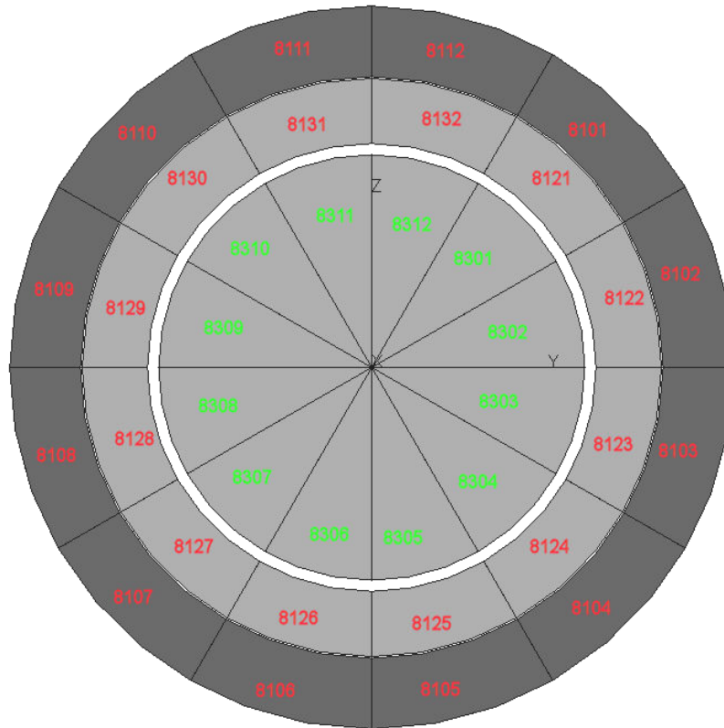
Figure 4.1.1-8 PLANCK Solar Arrays, -X side
