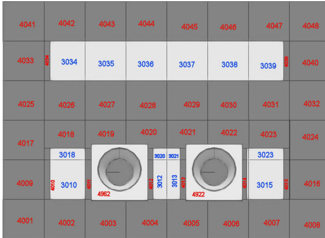
Figure 4.1.1-4 PLANCK DPU +Z external panel
