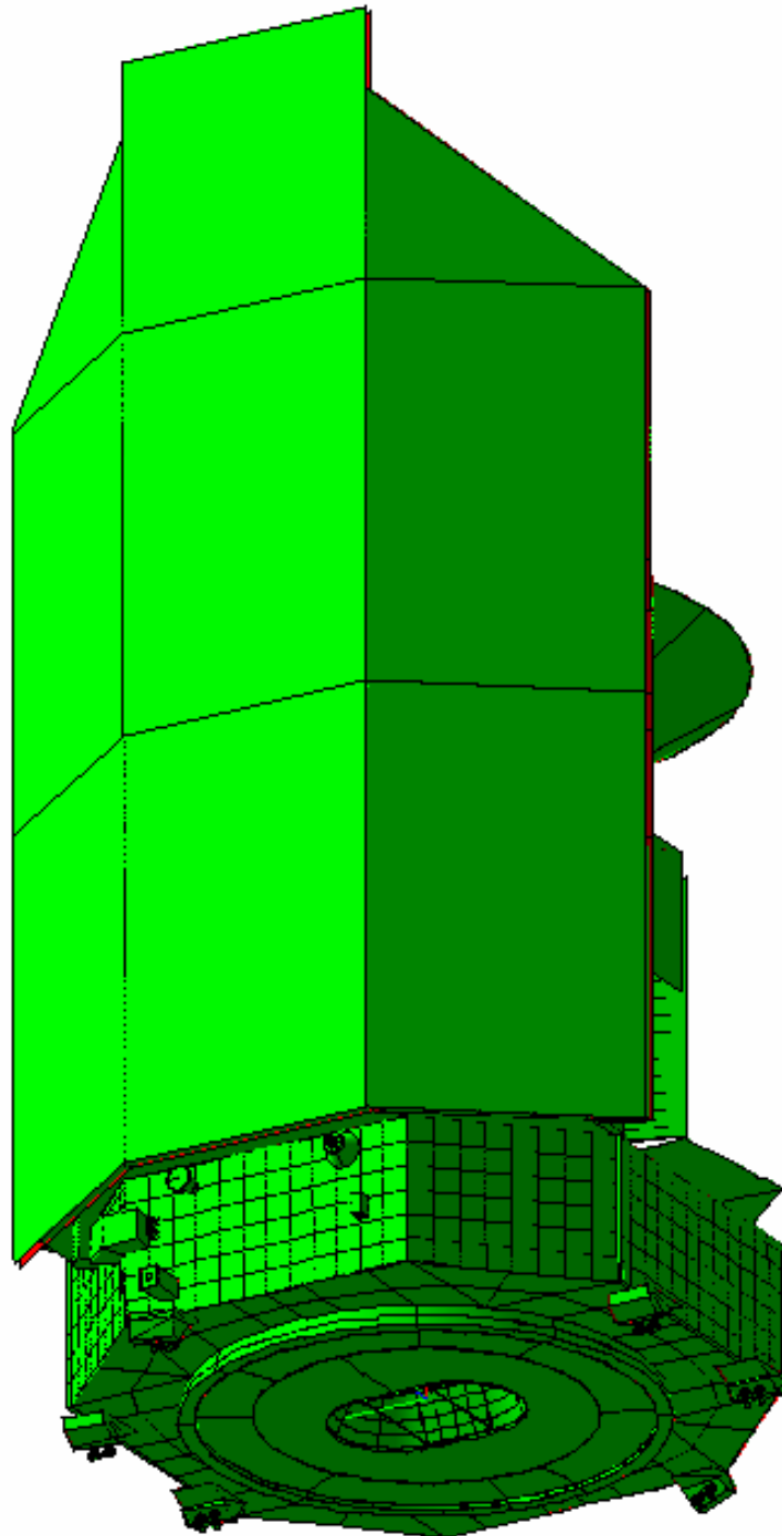
Figure 3-1 HERSCHEL – Overall view +Z
