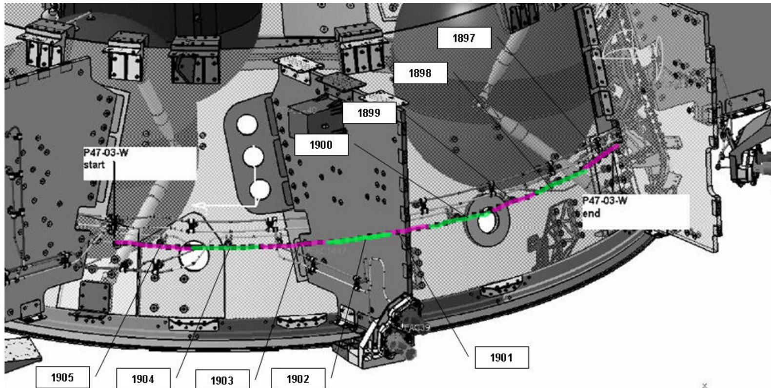
Figure 4.1.4-18 PLANCK - RCS Line #47
