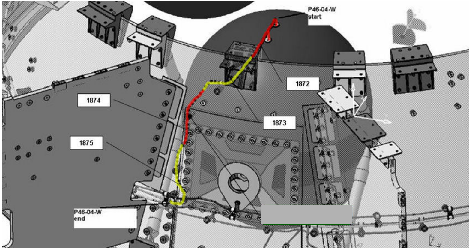
Figure 4.1.4-14 PLANCK - RCS Line #46
