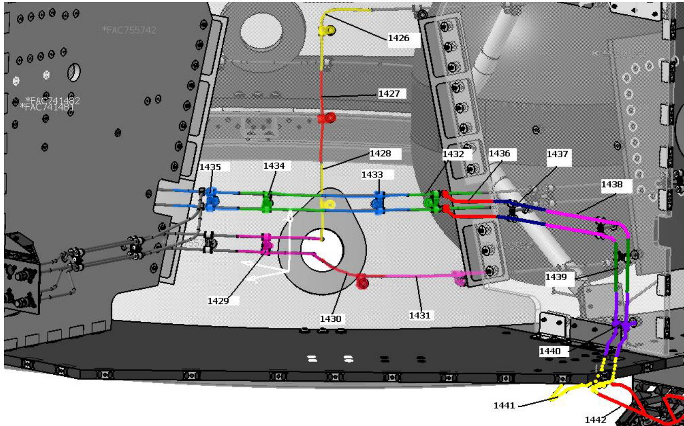
Figure 3.1.4-11 HERSHEL – RCS line47
