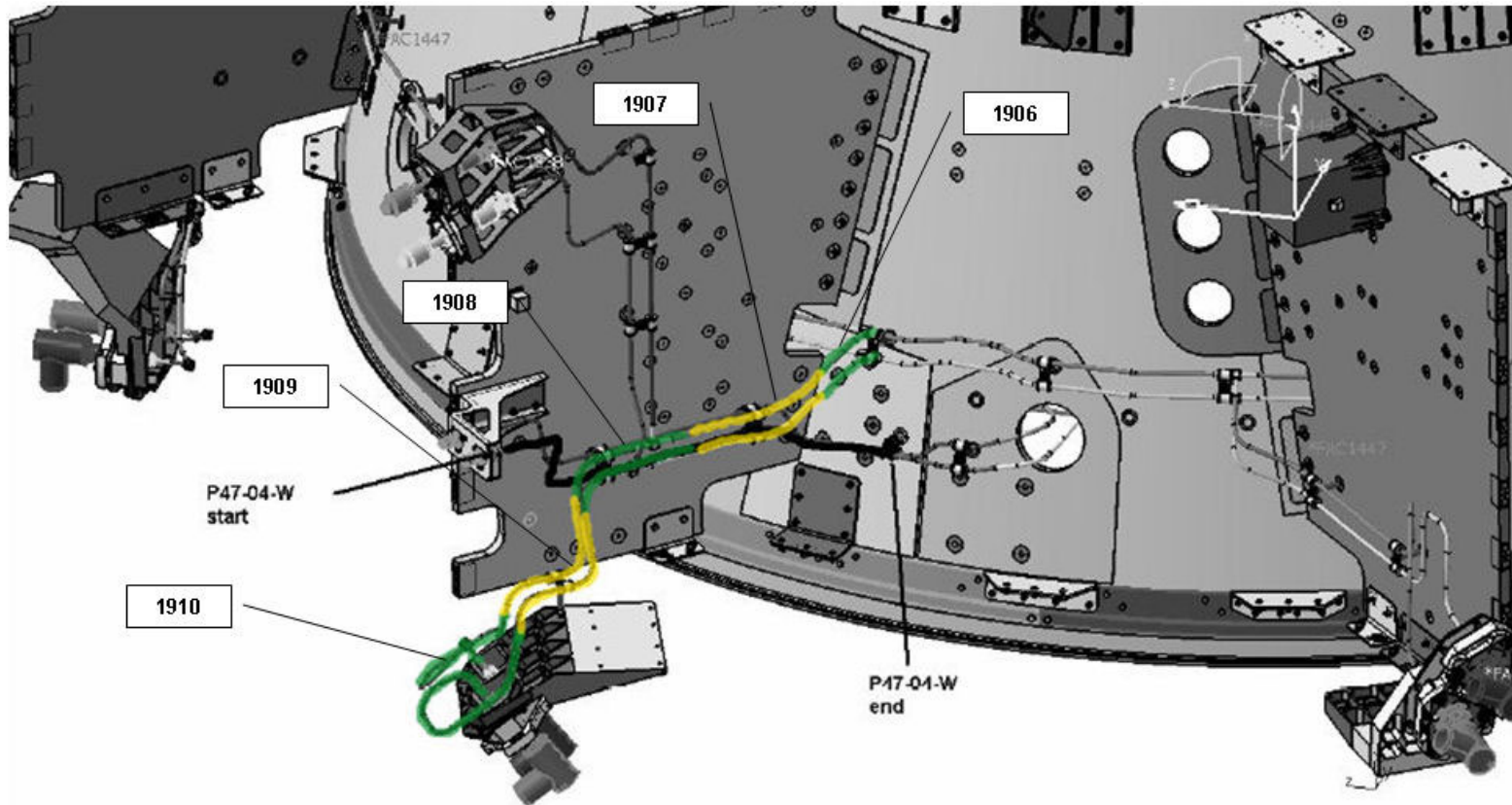
Figure 4.1.4-19 PLANCK - RCS Line #47
