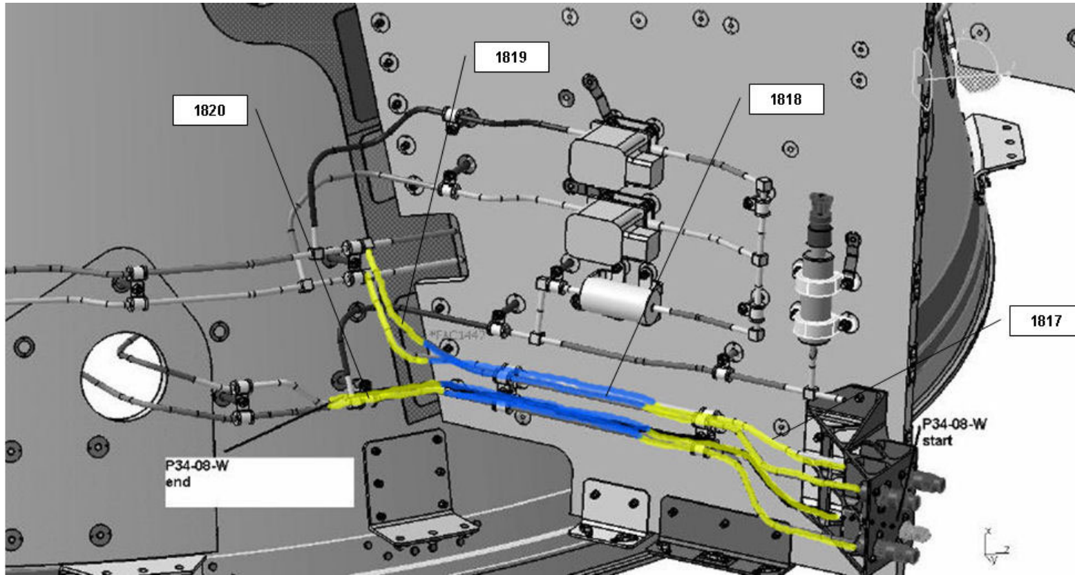
Figure 4.1.4-5 PLANCK - RCS Line #34
