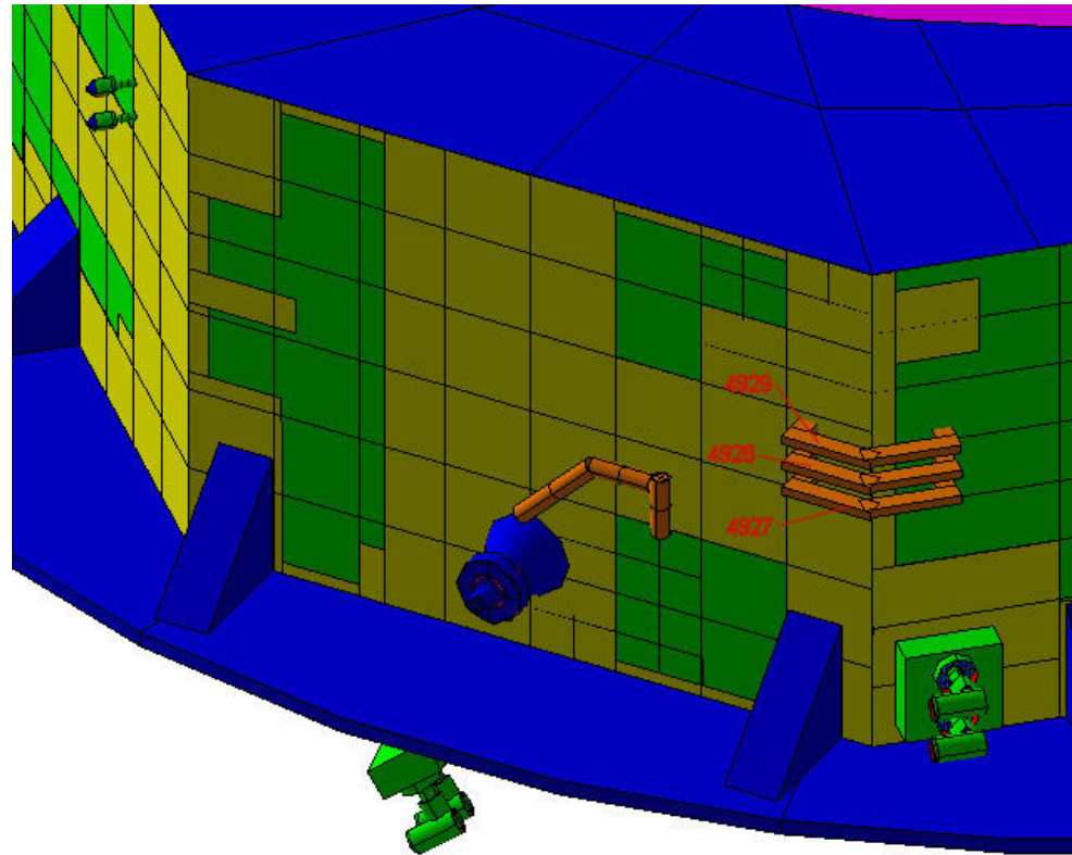
Figure 4.1.1-3 PLANCK TT&C -Y external panel: WG GMM
