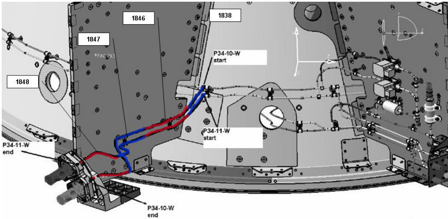
Figure 4.1.4-10 PLANCK - RCS Line #34
