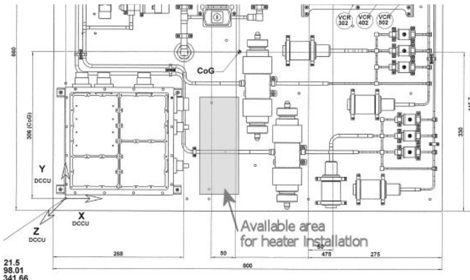
Figure 4.1.8-1 DCE possible heater location.
