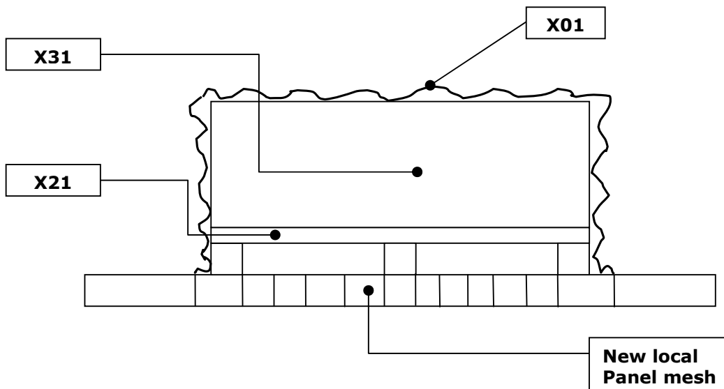
Figure 3.1.2-4 HERSCHEL – FHWOV/FHWOH new model
