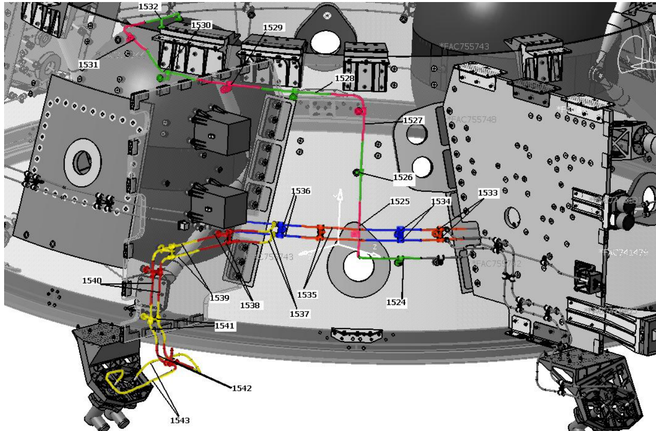
Figure 3.1.4-4 HERSHEL – RCS line11
