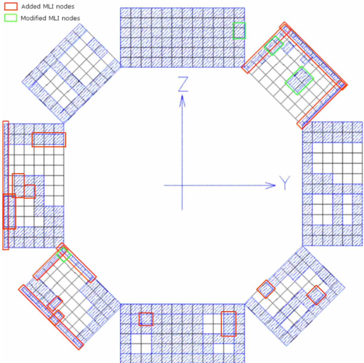
Figure 3.1.1-1 HERSHEL – SVM external panels radiators layout
