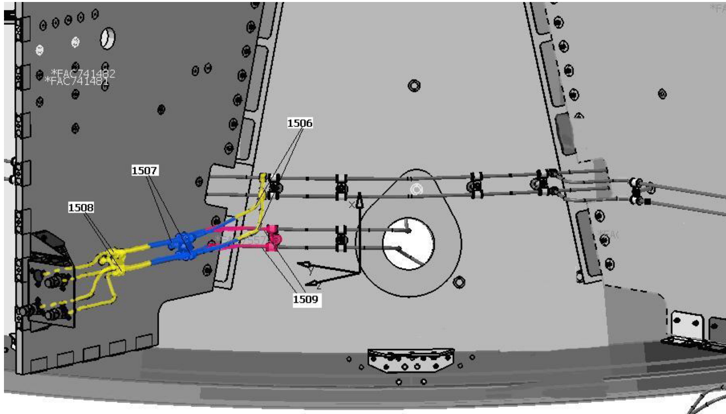
Figure 3.1.4-2 HERSCHEL – RCS line9
