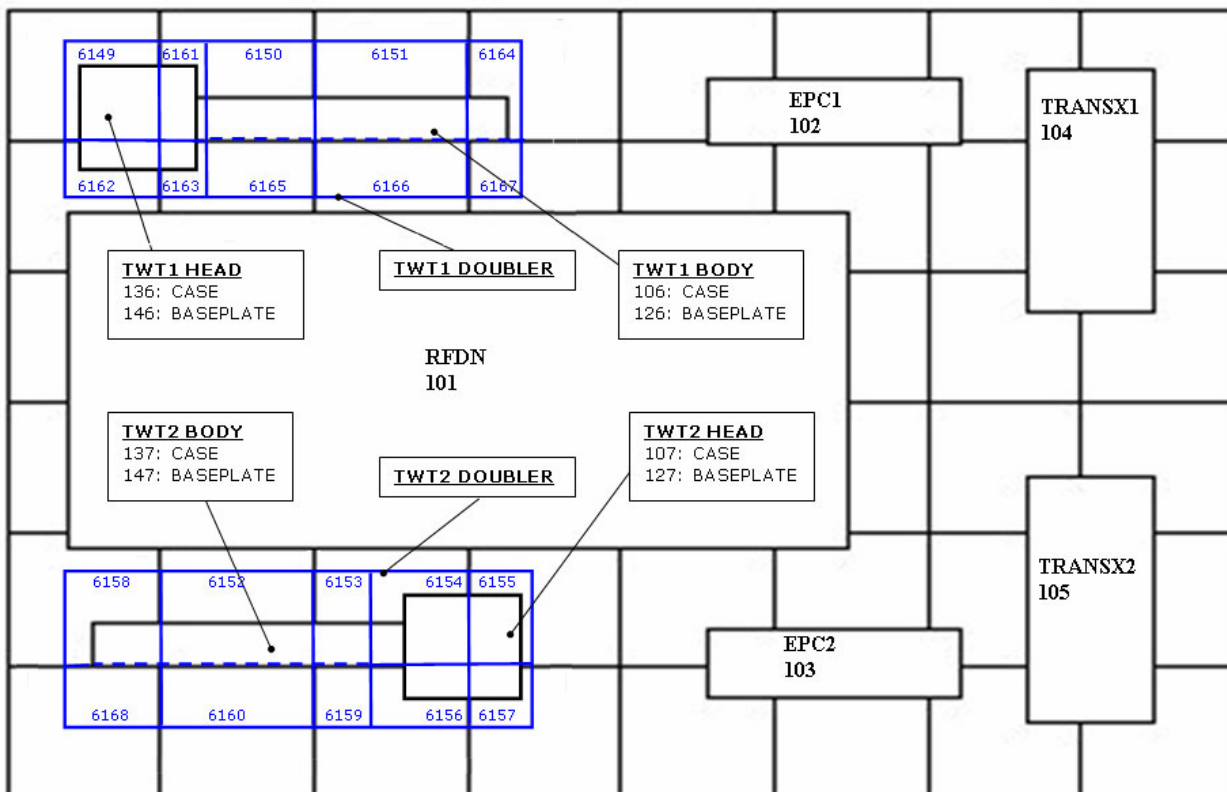
Figure 3.1.2-5 HERSHEL – TT&C doublers new local mesh
