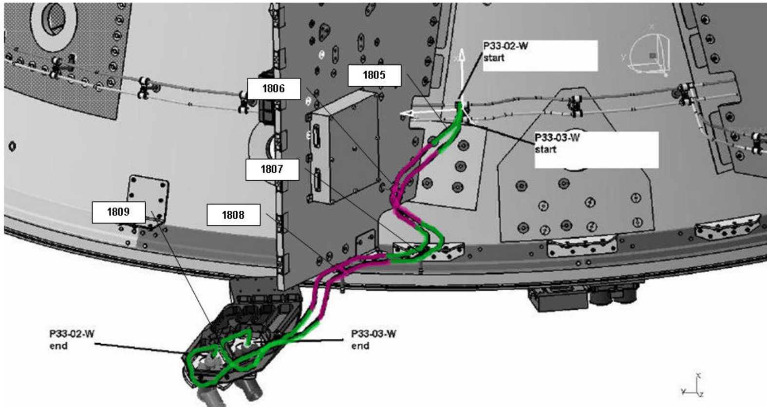
Figure 4.1.4-2 PLANCK - RCS Line #33
