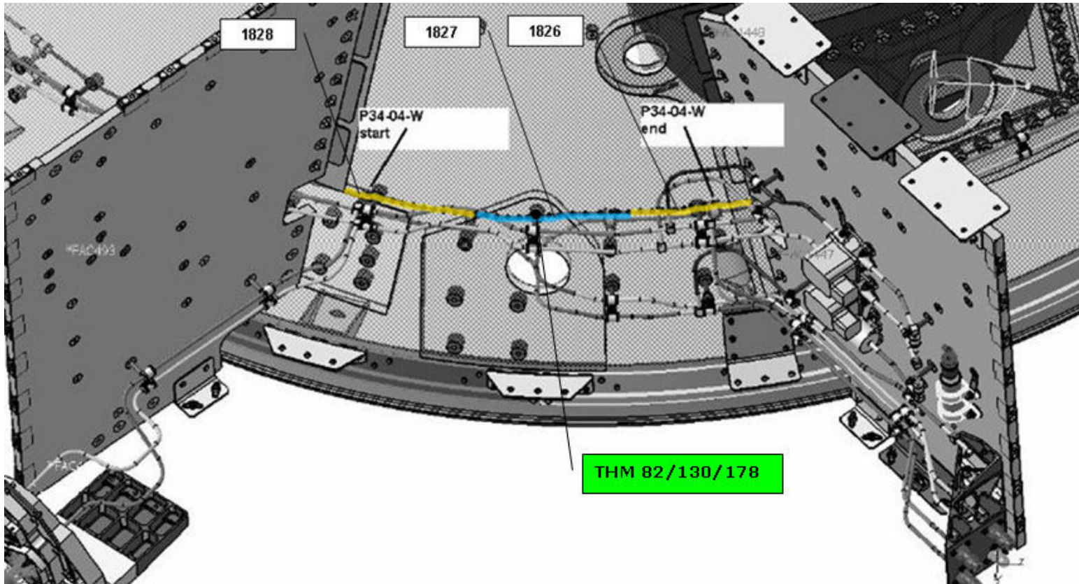
Figure 4.1.4-8 PLANCK - RCS Line #34
