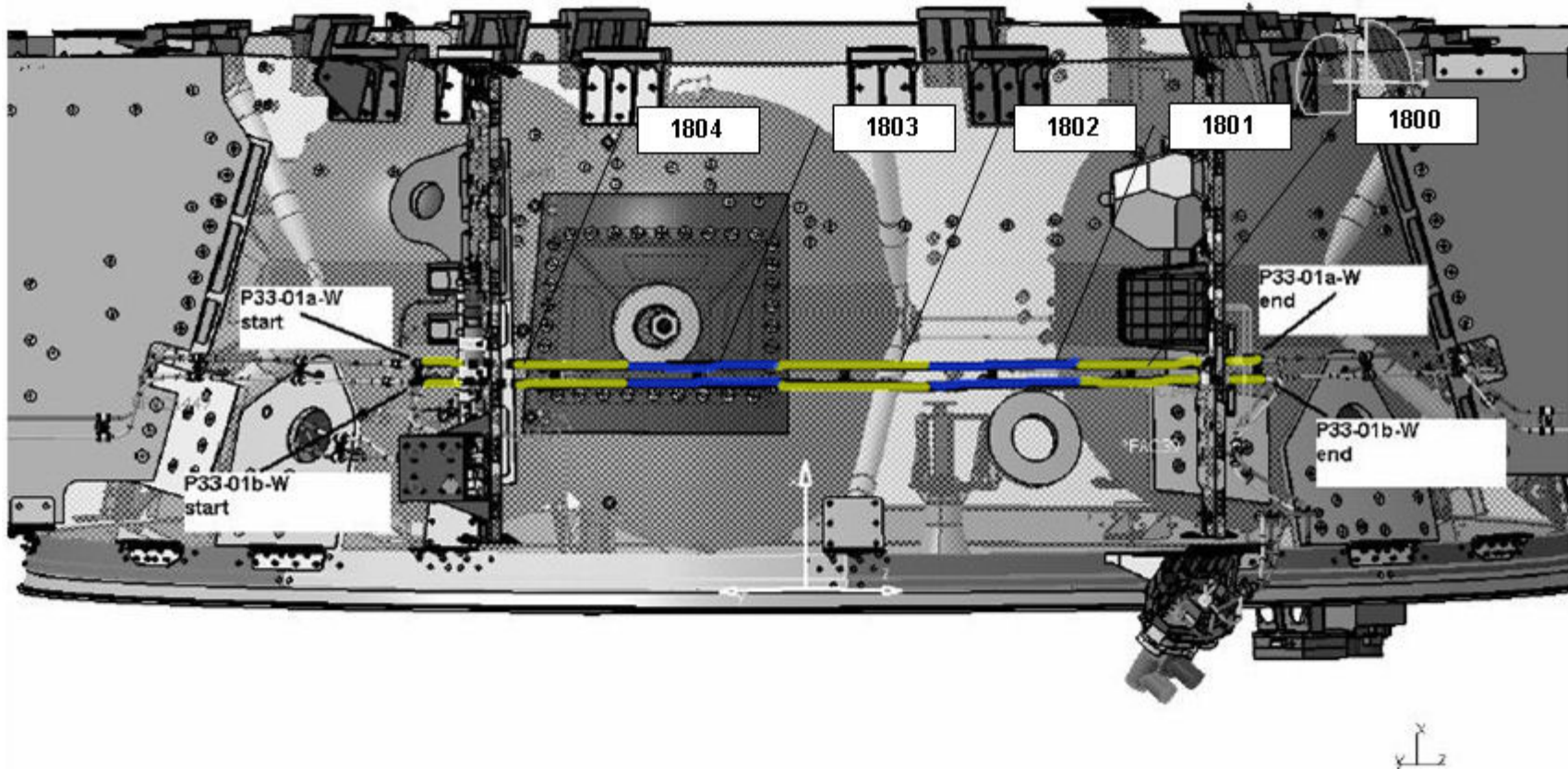
Figure 4.1.4-1 PLANCK - RCS Line #33
