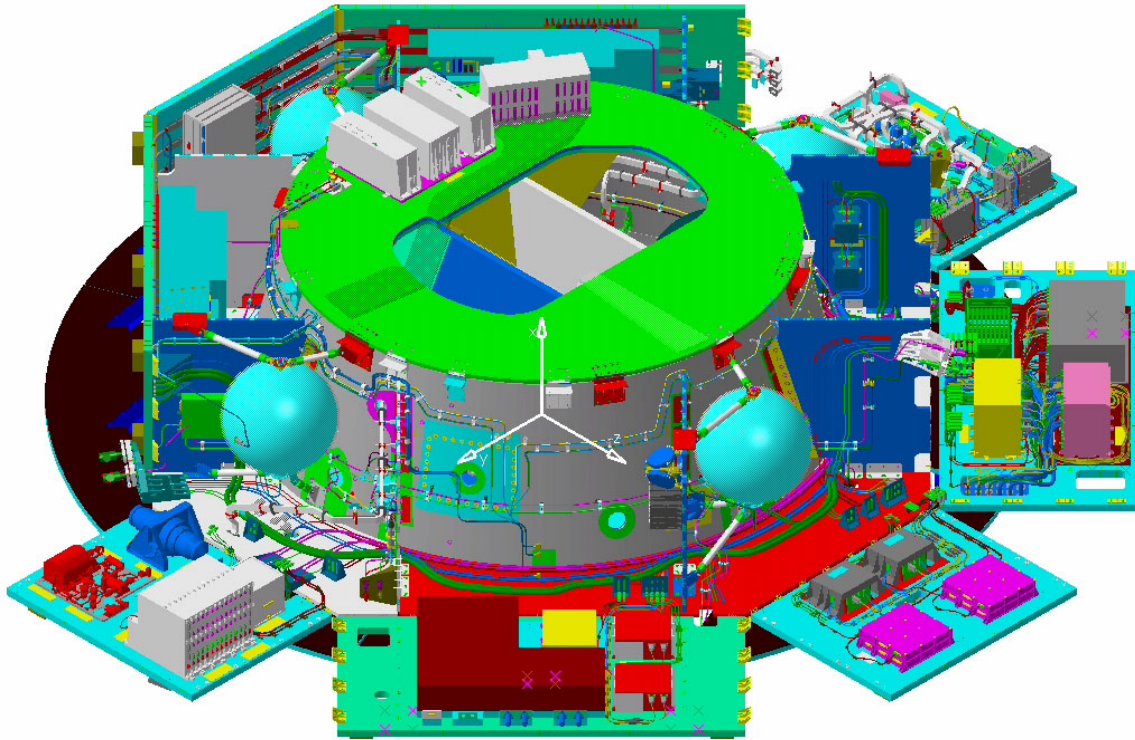
Figure 4-5 PLANCK – Internal overall View
