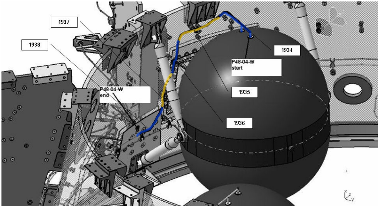
Figure 4.1.4-24 PLANCK - RCS Line #48
