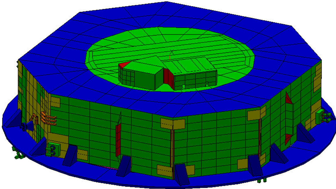
Figure 4-4 PLANCK - Overall view (Groove shield not plotted)
