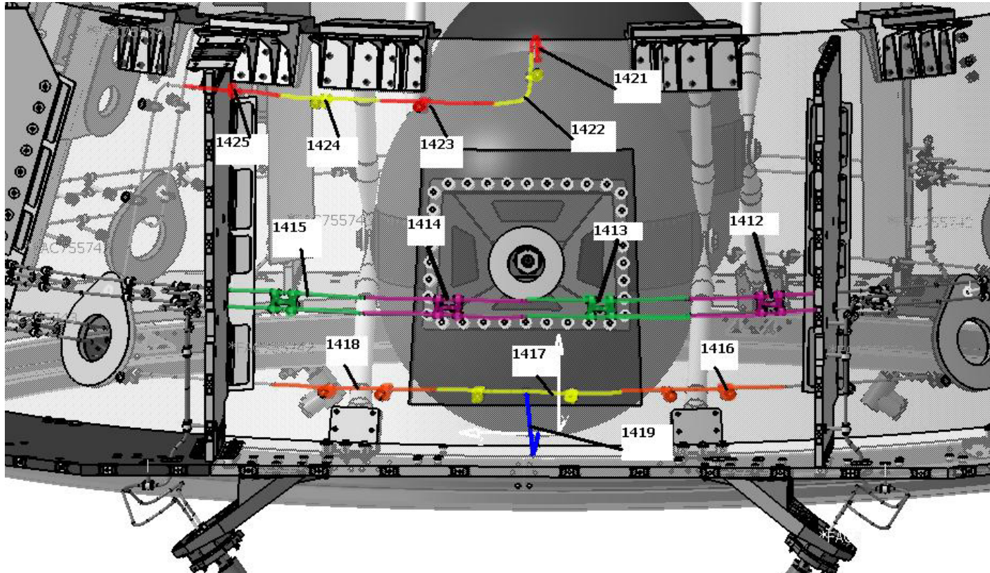
Figure 3.1.4-10 HERSHEL – RCS line46
