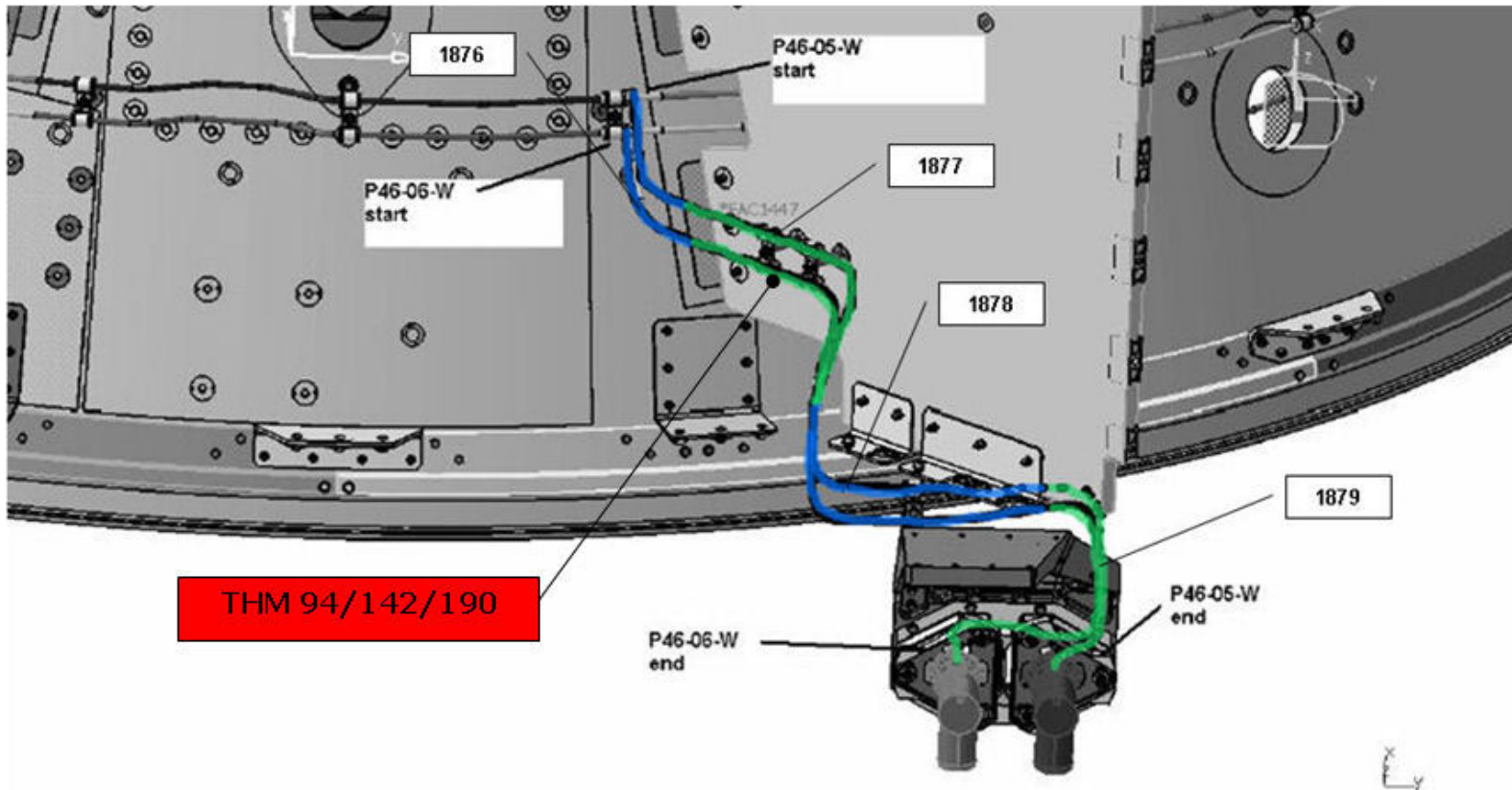
Figure 4.1.4-15 PLANCK - RCS Line #46
