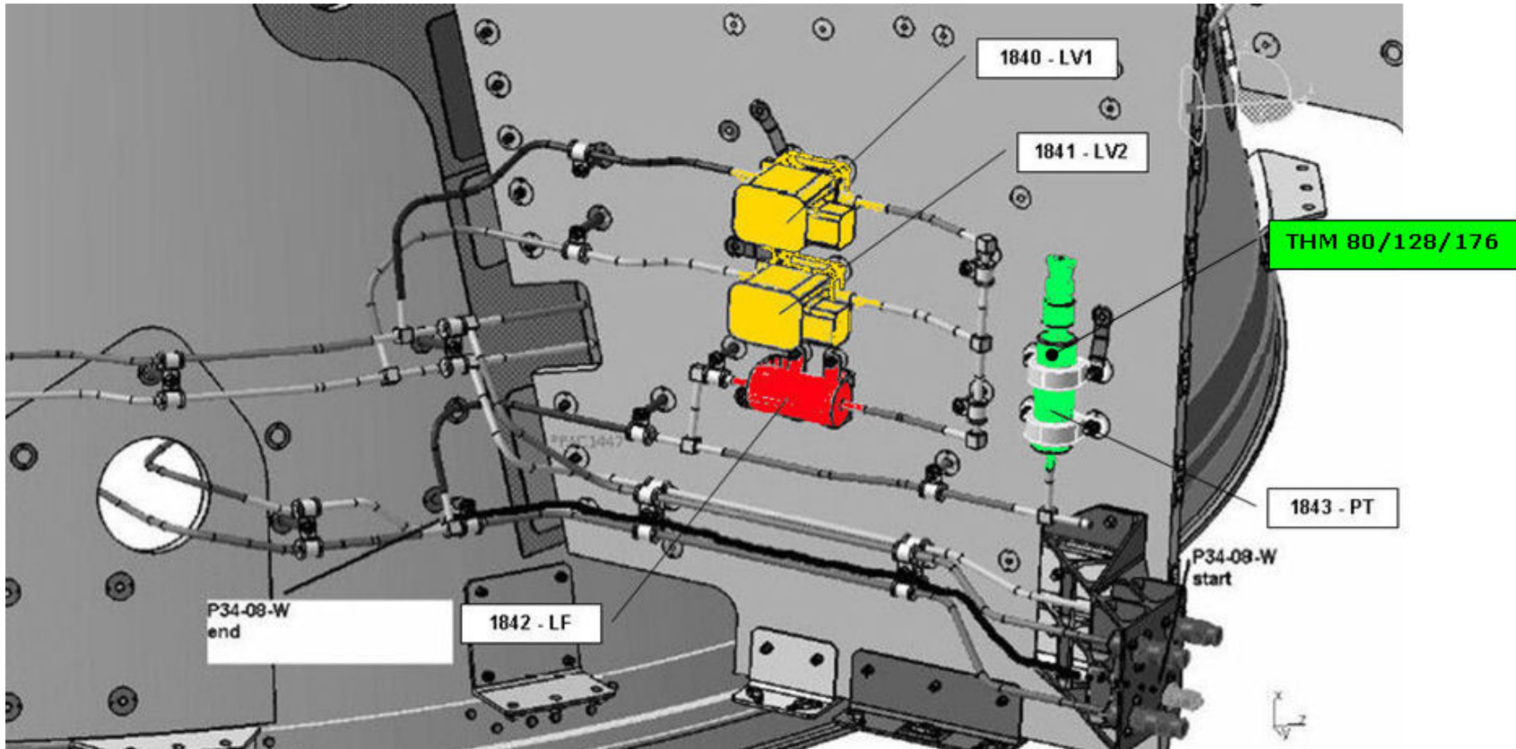
Figure 4.1.4-26 PLANCK - RCS Line #32 (RCS Units)
