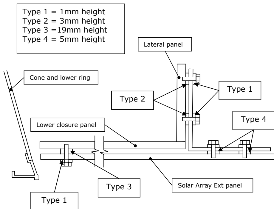
Figure 5.7-2 PLANCK – Connection Solar Array-Lateral panel
