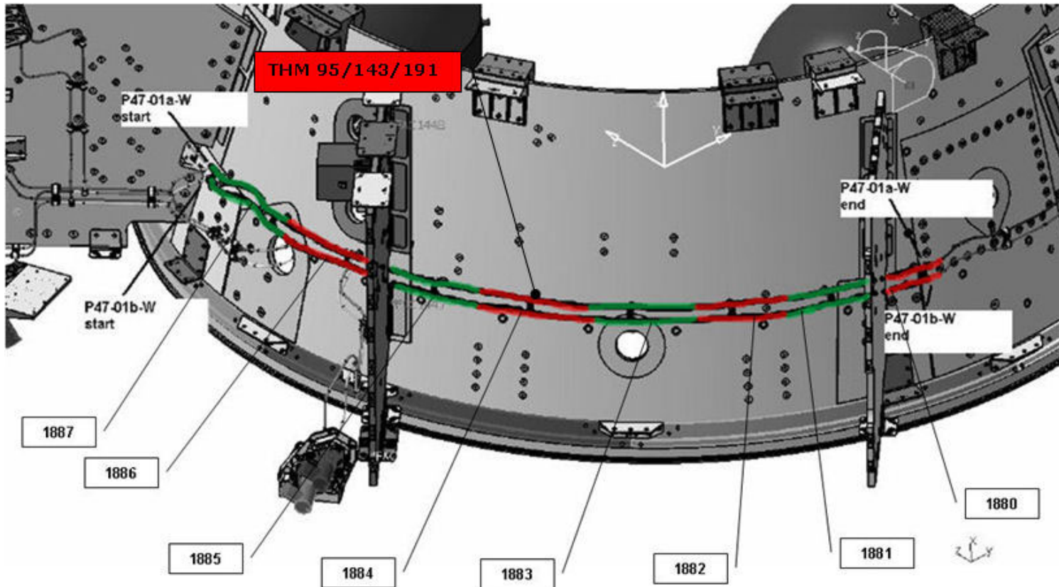
Figure 4.1.4-16 PLANCK - RCS Line #47
