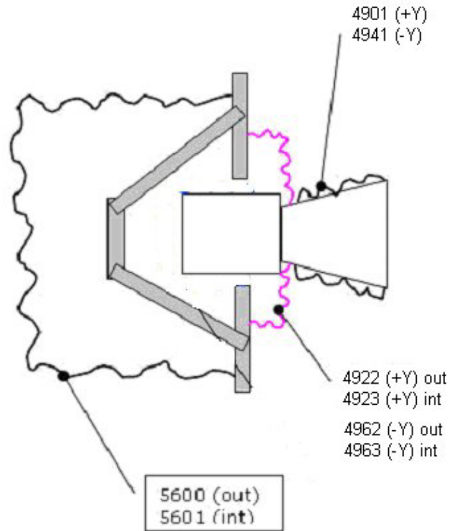
Figure 4.1.2-3 PLANCK Star Trackers MLI
