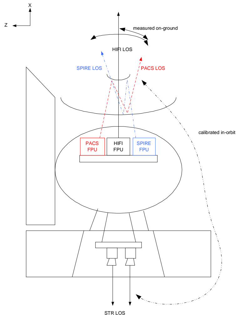
Figure 2-3 instruments LOS schematic projection on the sky
