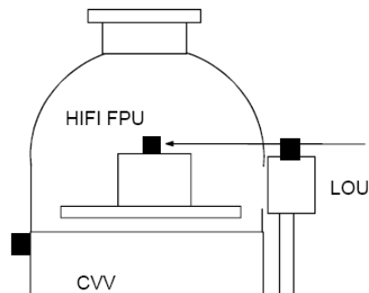
Figure 2-4 LOU to HIFI FPU coalignment - schematic
