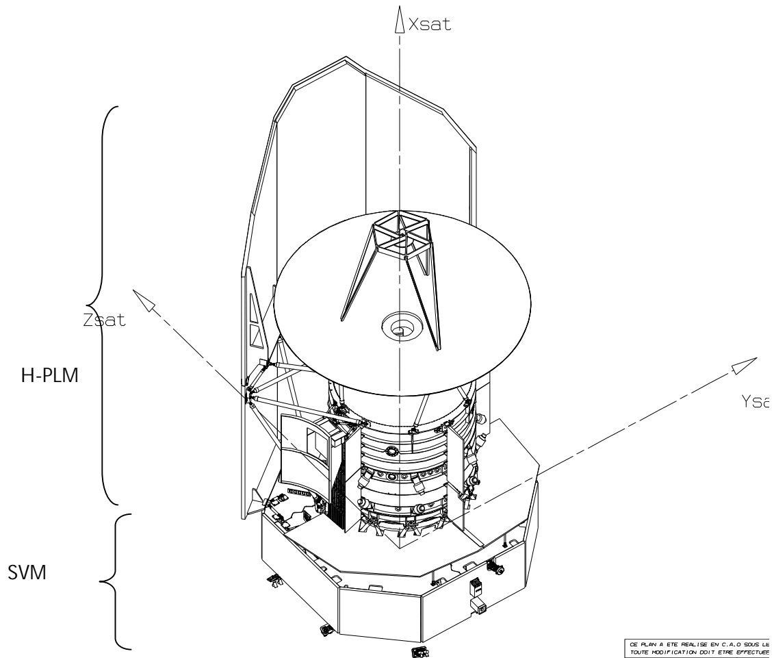
Figure 2-1 Herschel S/C axis
