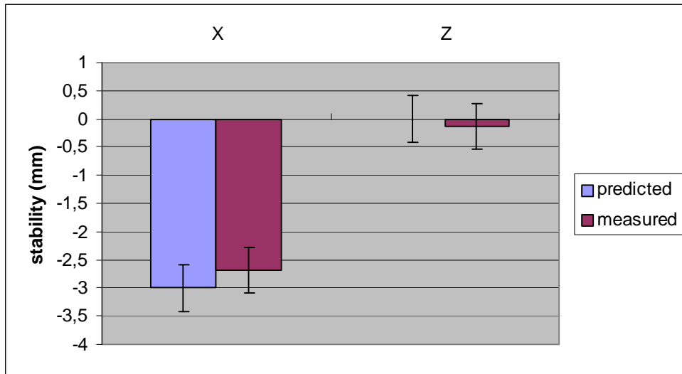
Figure 4-3 FEM correlates well the LOU to FPU stability from warm/warm conditions to cold/cold conditions
