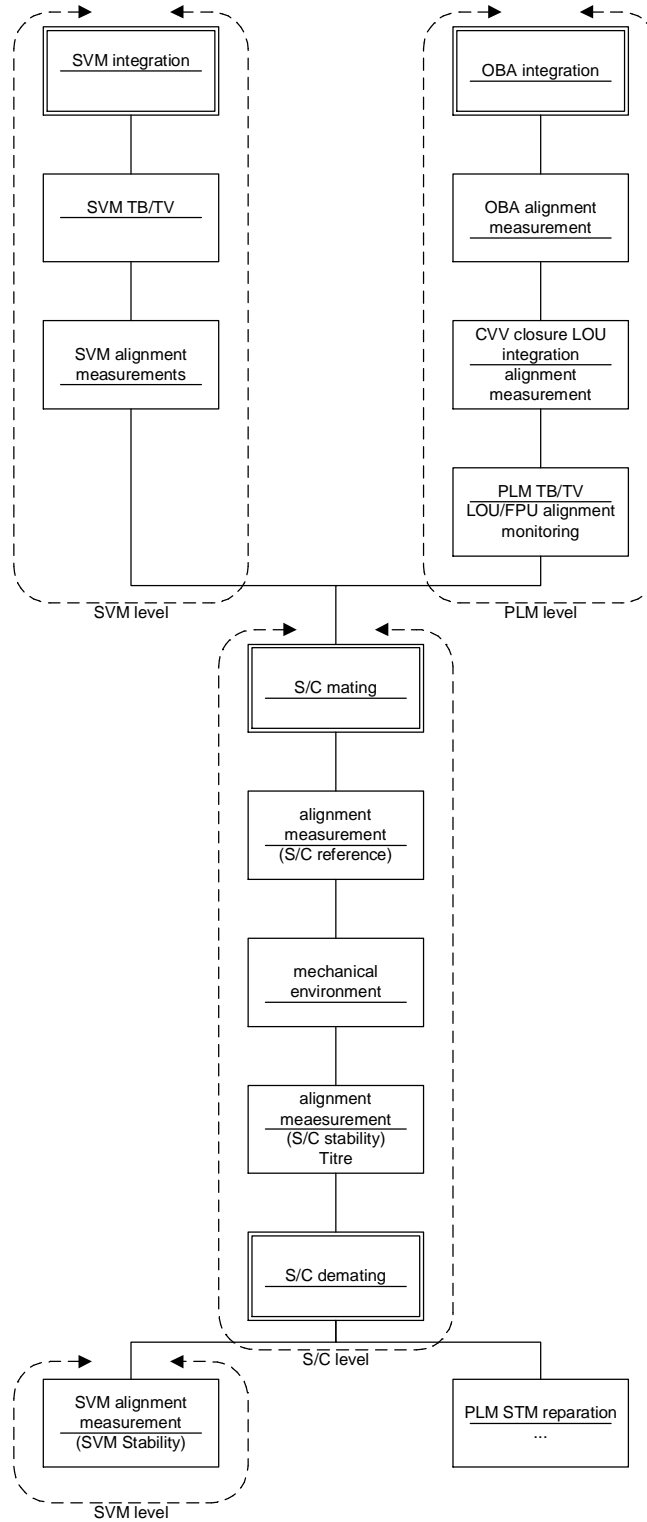
Figure 4-1 STM alignment activities sequence
