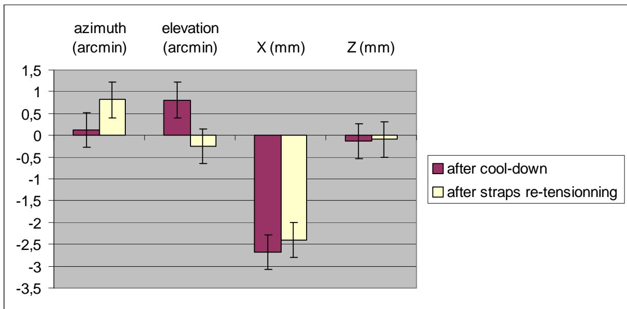
Figure 4-2 stability of FPU wrt LOU during PLM integration -> main effect is cool-down along X
