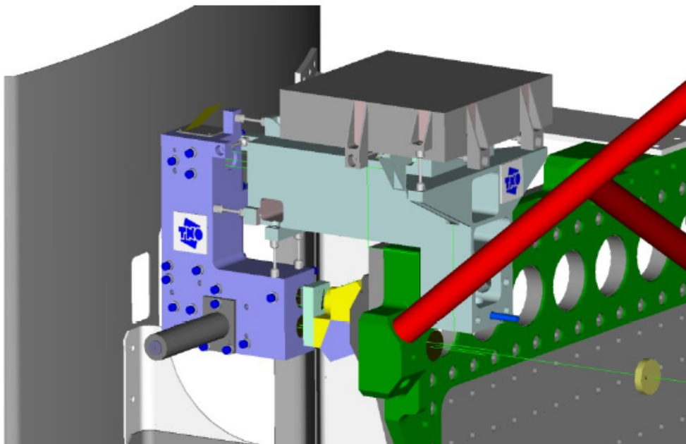
Figure 5-2 one camera HACS integrated on -Z side of LOU
