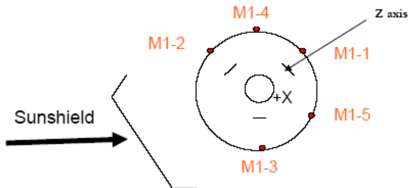
Figure 5-5 M1 Corner cube accommodation
