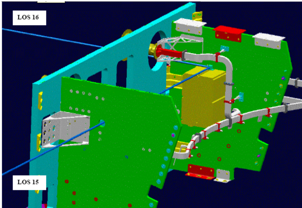
LoS 16 is accessible with all panel closed, LOS 15 is only accessible with panel-Y+Z dismounted
