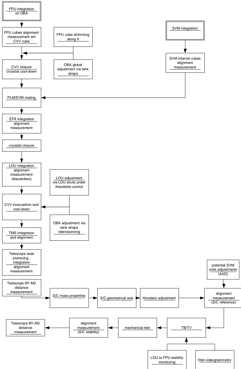
Figure 5-1 FM alignment flow
