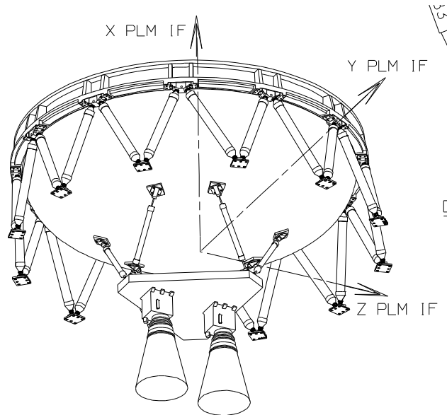
Figure 2-2 for stability reason, star trackers are interfaced to PLM , not SVM Note that, despite this accommodation, STR are functionally part of SVM
