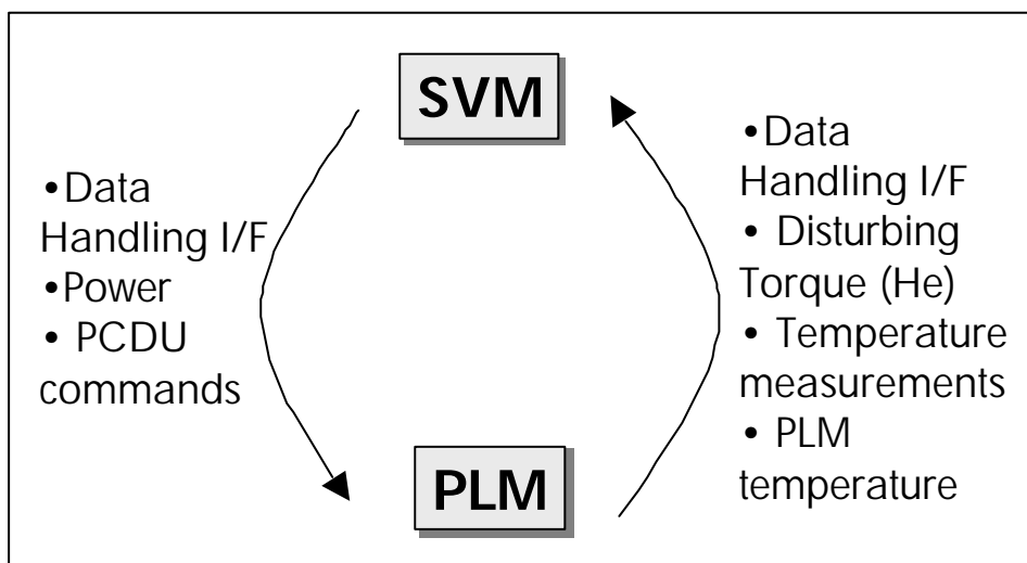
Figure 1.8.2 : System internal data interfaces -SVM / PLM (relevant for FDIR analysis)
