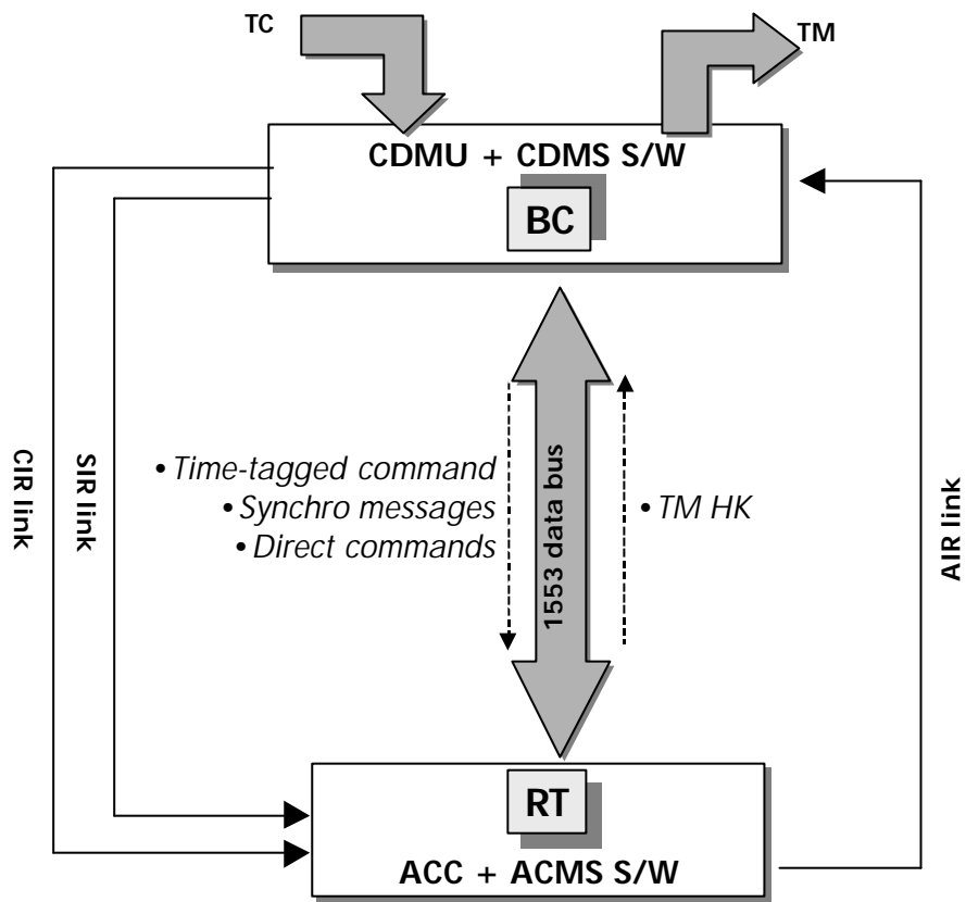
Figure 3.4.2 : CDMS/ACMS Communication
