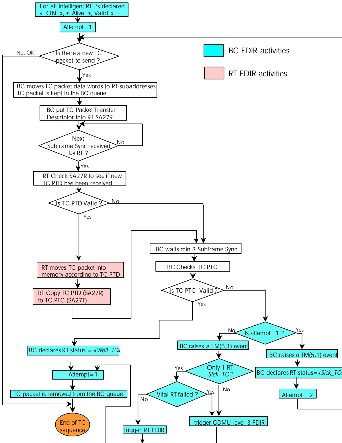
Figure 3.3-1 : TFL TC protocol flow chart & FDIR
