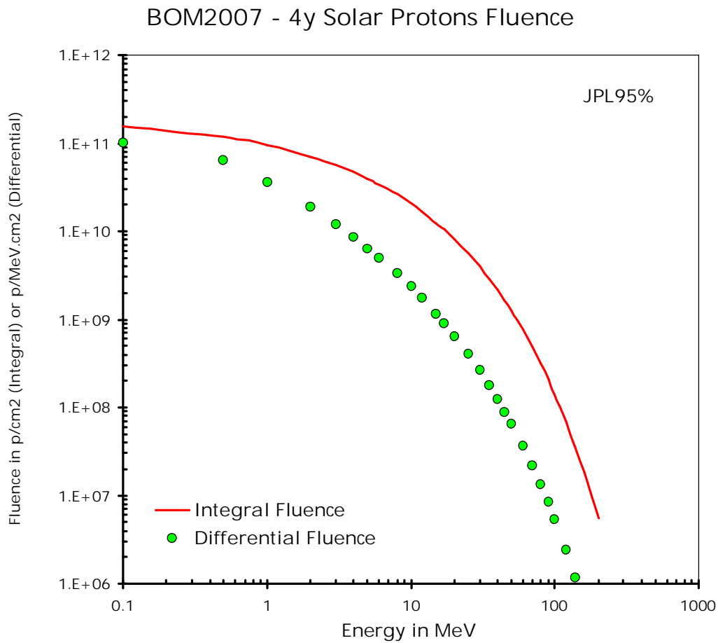
Figure 3-20: Solar Protons Fluence for the 4 years mission BOM 2007
