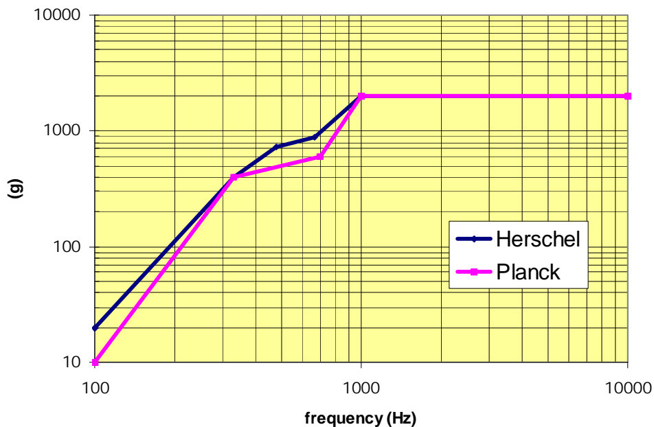
Figure 3-5: Shock Spectrum at launcher interface
