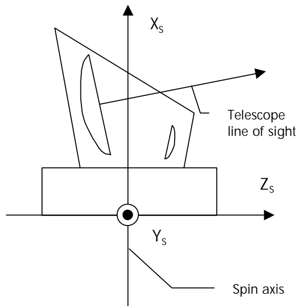
Figure 3-3: PLANCK Spacecraft Axis
