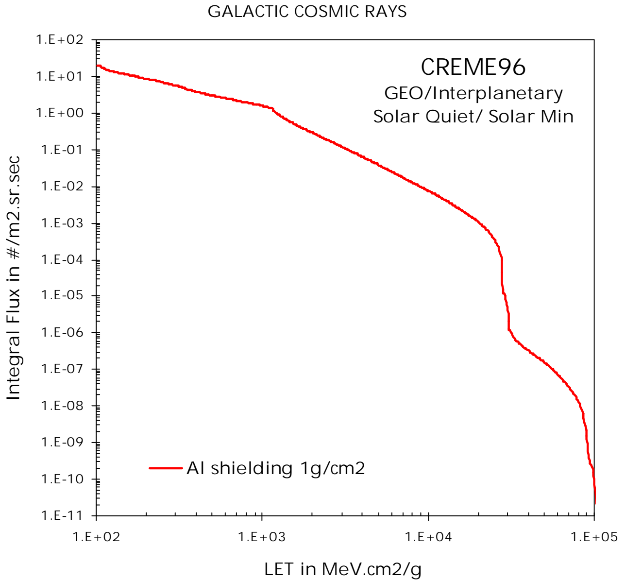
Figure 3-24: Galactic Cosmic Rays LET spectrum
