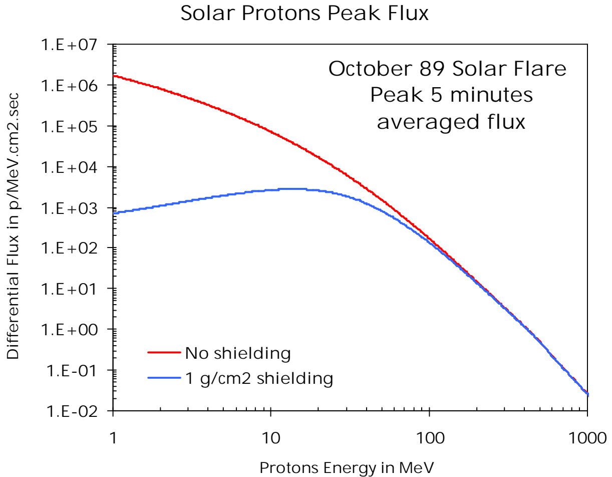
Figure 3-22: Solar Protons Peak Fluxes
