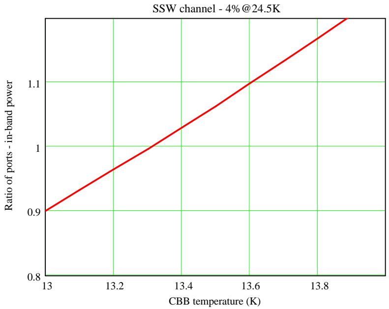
Figure 6 Example output from photometric model showing the ratio of in-band power at each spectrometer port as a function of CBB temperature, for a certain source temperature.
