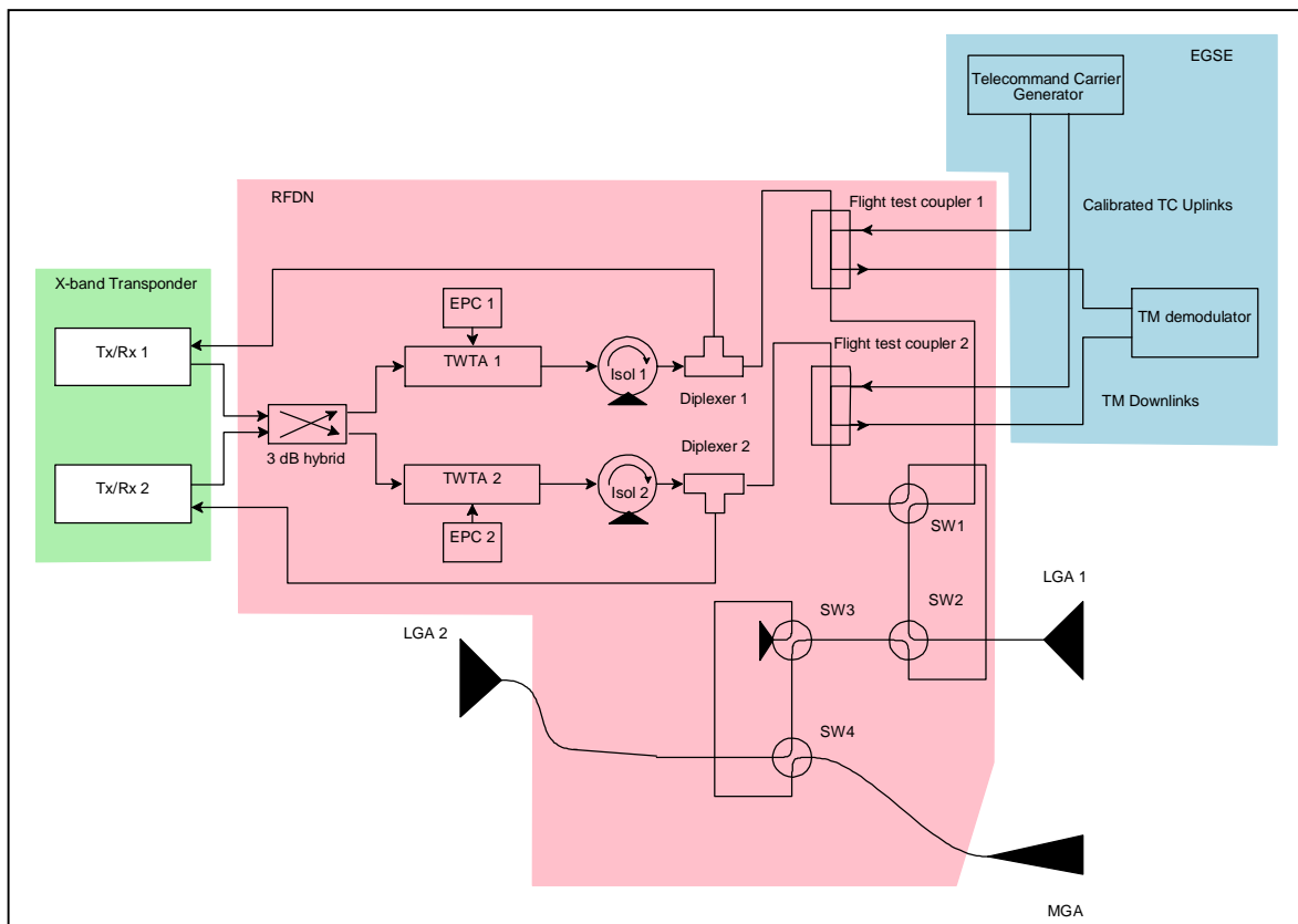
Figure 7-1 RF-EGSE and TTC Subsystem interconnection
