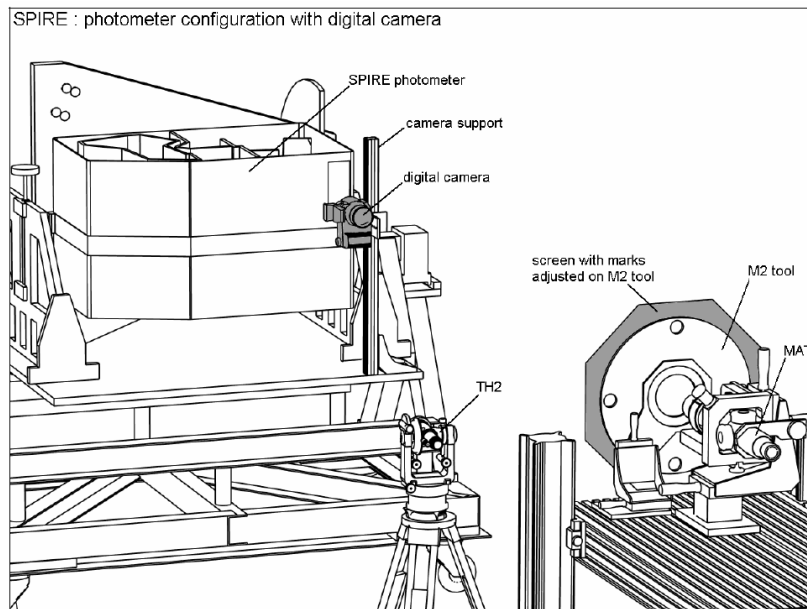
Figure 2: Set-up configuration for ambient pupil alignment verification on AM, CQM, PFM and FS (from RD1)
