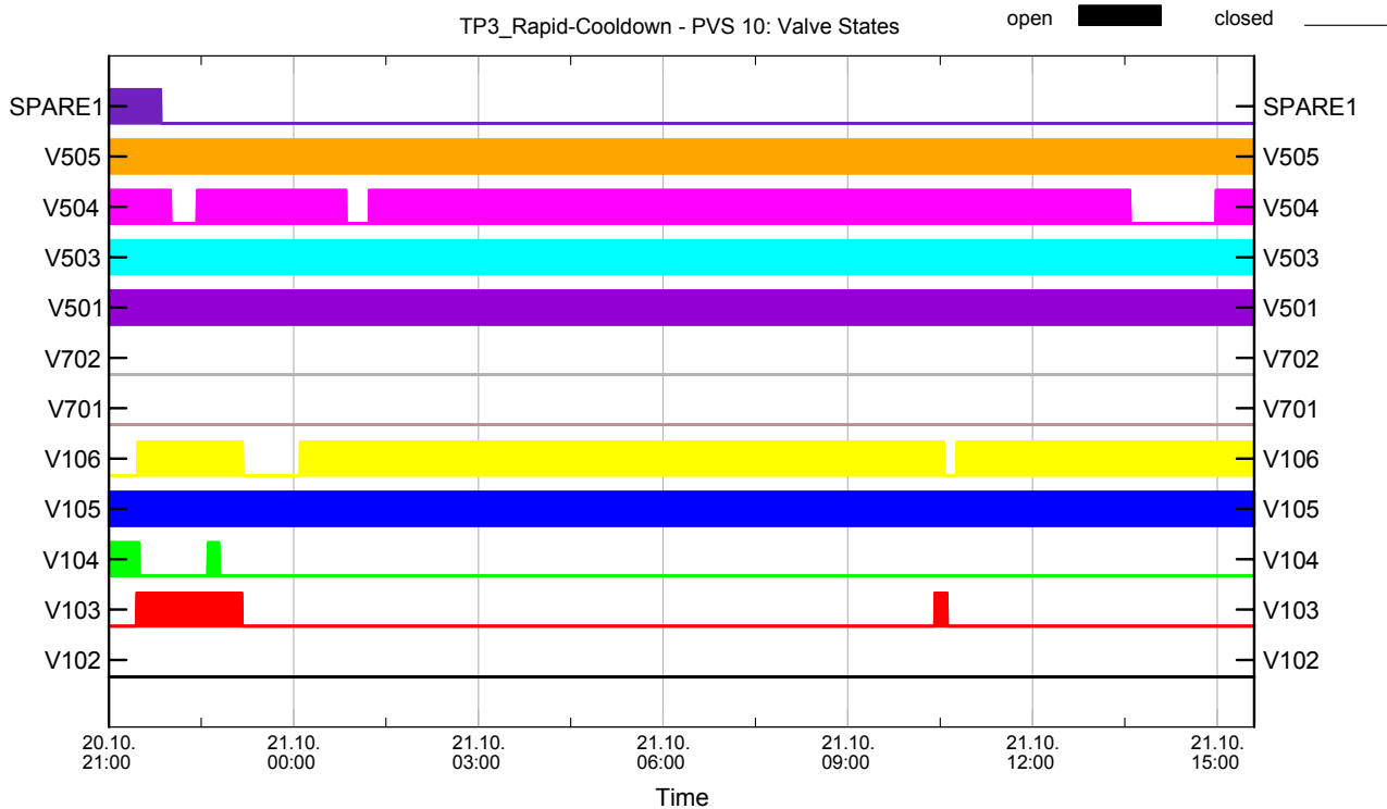
Figure 7.1-5: Valve states at end of TP3 (PVS 10)
