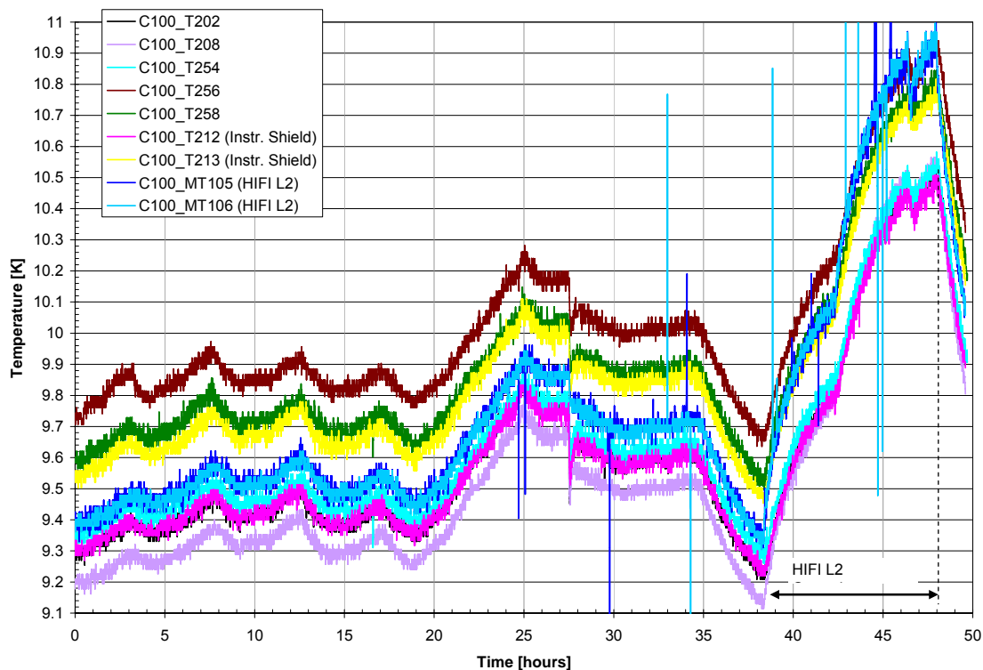
Figure 3.3-7: OBP Temperature Evolution during TP6
