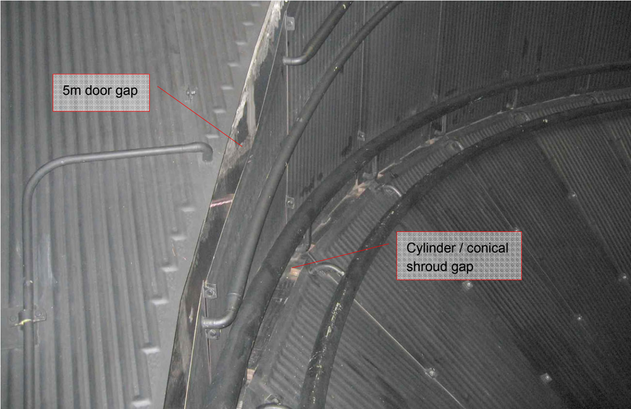
Figure 6.4-9: Circumf. gaps around 5m door connection and between conical and cylindrical shroud
