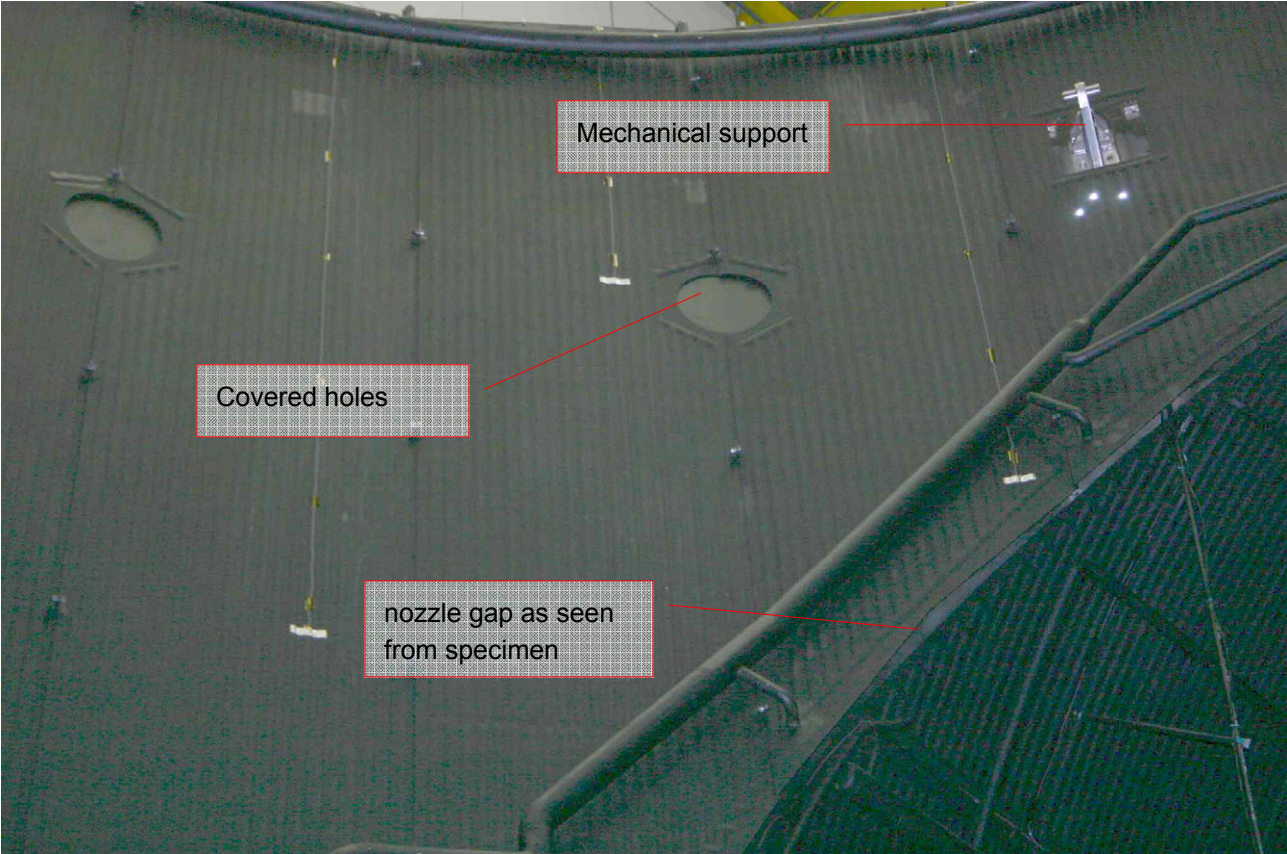
Figure 6.4-7: Mechanical support and nozzle gap
