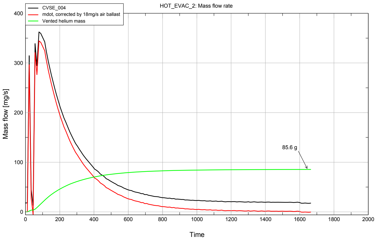
Figure 7.3-12: Vented helium mass during HOT evacuation test 2
