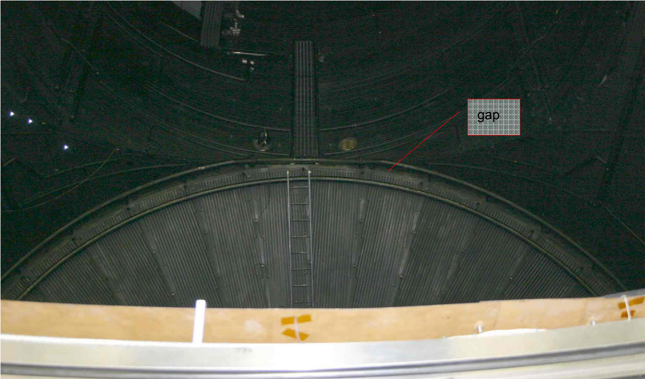
Figure 6.4-8: Circumferential gap between conical and cylindrical shroud
