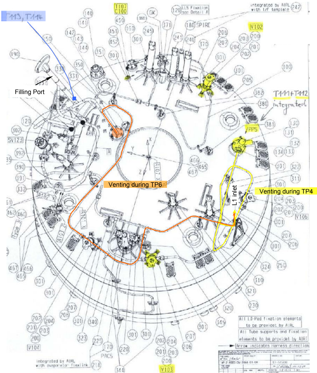
Figure 3.4-3: Helium Venting Path during TP4 and TP6
