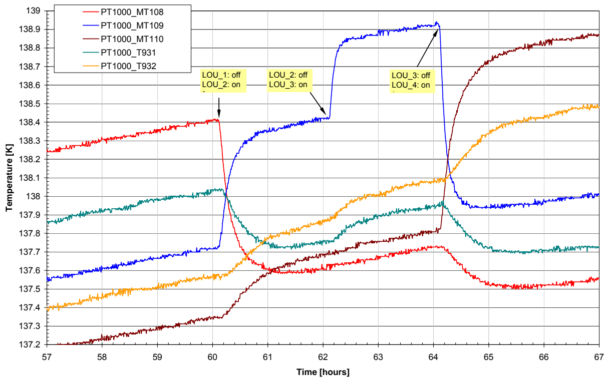
Figure 4.4-5: LOU Temperature Evolution during Switch of MTD Heaters (TB2)
