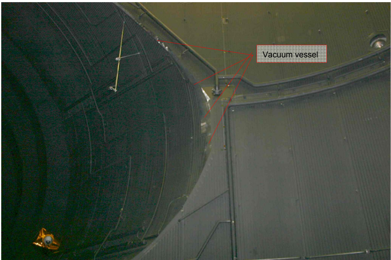
Figure 6.4-4: Shroud gaps in nozzle connection to cylinder
