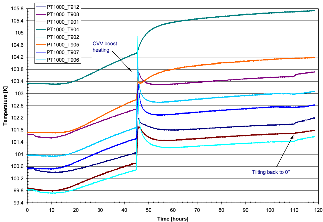
Figure 4.2-6: CVV Temperature Evolution during TB2 Test Phase (TP7)
