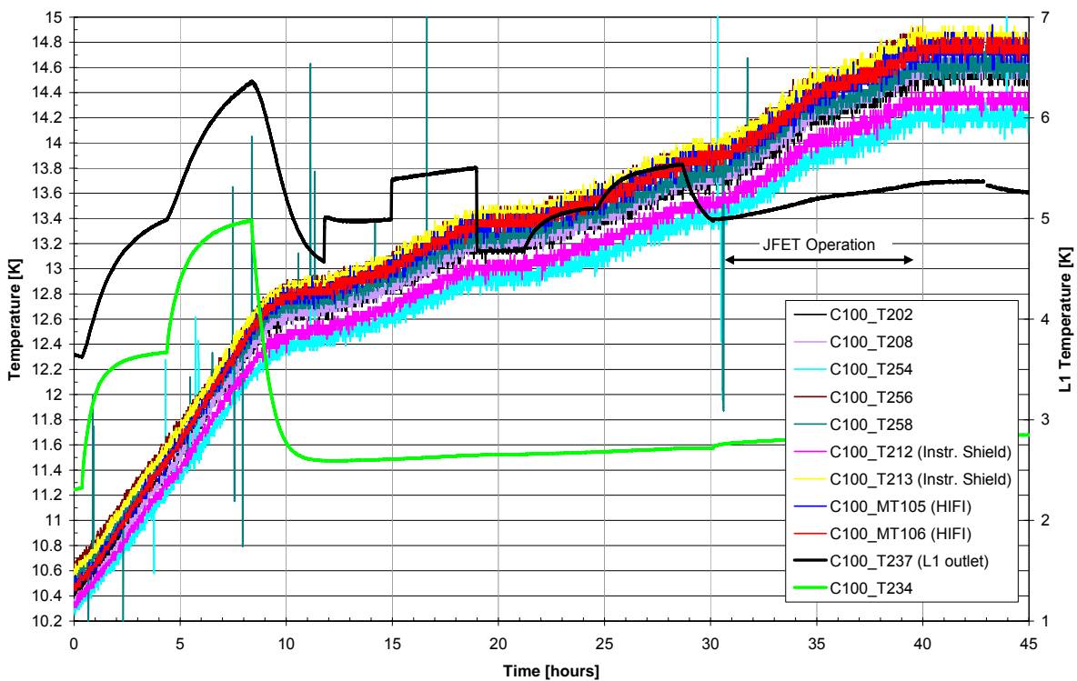
Figure 3.3-1: OBP Temperature Evolution during TP4
