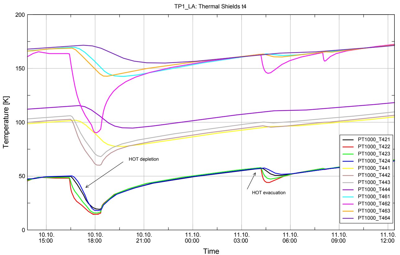
Figure 7.3-20: Thermal shields temperatures during HQT evacuation test 3
