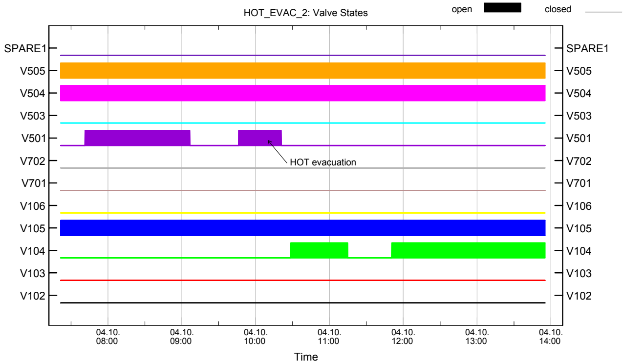
Figure 7.3-13: Electromagnetic valve states for HOT evacuation test 2
