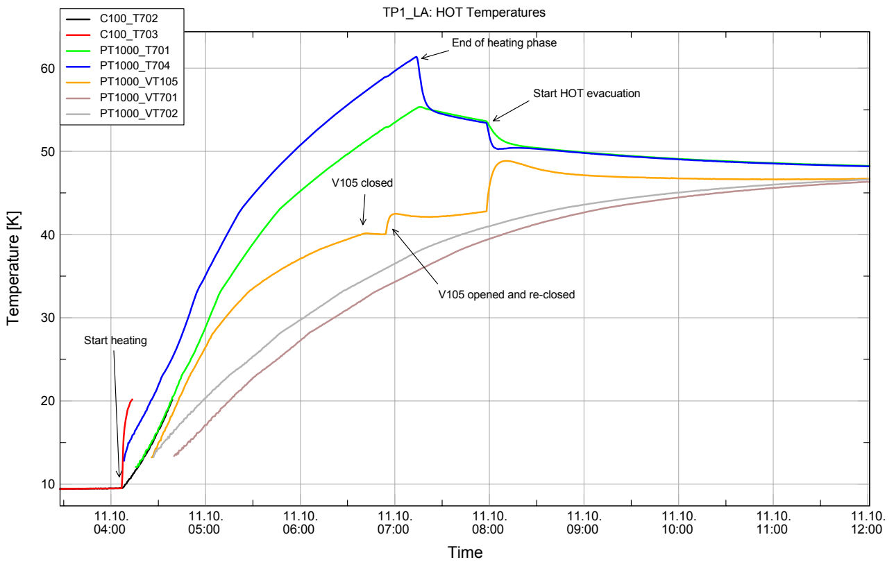
Figure 7.3-19: HQT and valves temperatures during HQT evacuation test 3
