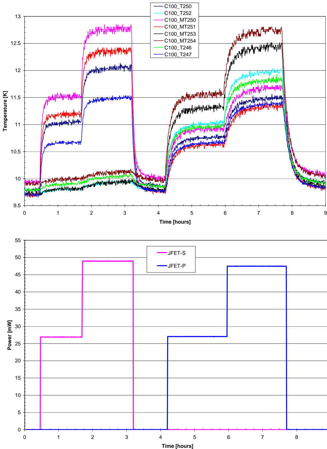
Figure 5.5-1: SPIRE JFET Power and Temperature Evolution during Operation (TP6)
