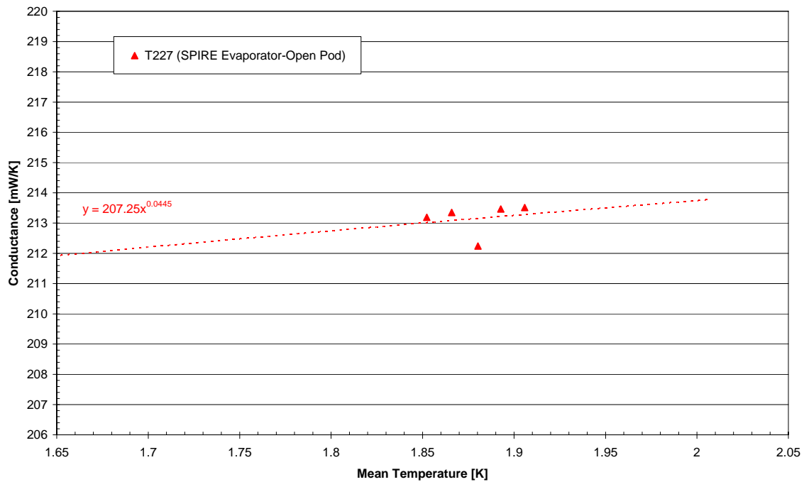
Figure 3.5-13: Thermal Conductance versus Mean Temperature for SPIRE L0 I/F to Helium
