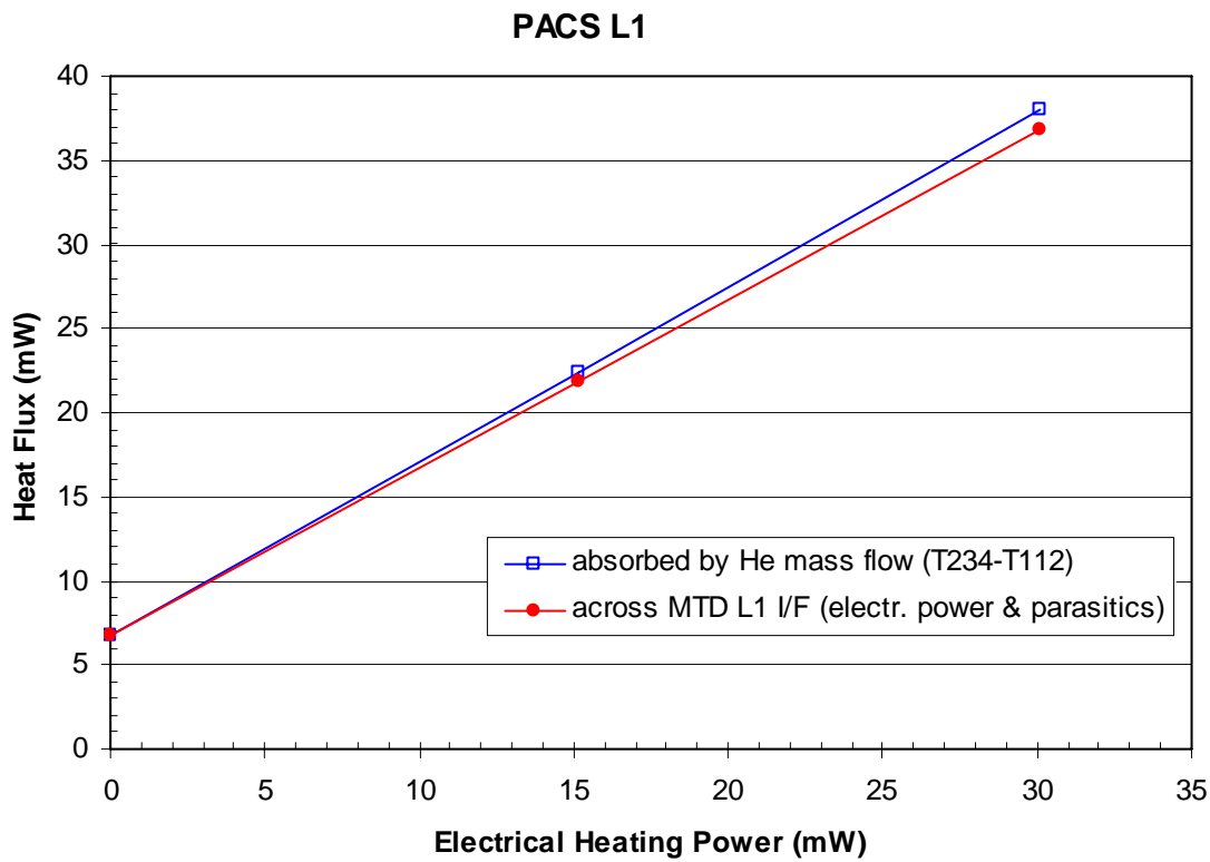
Figure 4.2-4: PACS L1 Interface Heat Flows (TP4)
