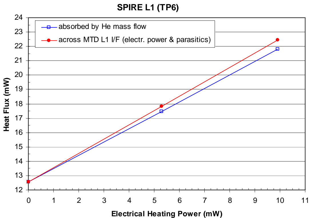
Figure 4.6-4: SPIRE L1 Interface Heat Flows (TP6)
