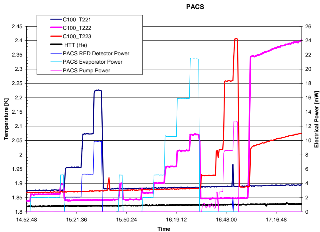
Figure 3.5-4: Power and Temperature Evolution of PACS L0 Interfaces
