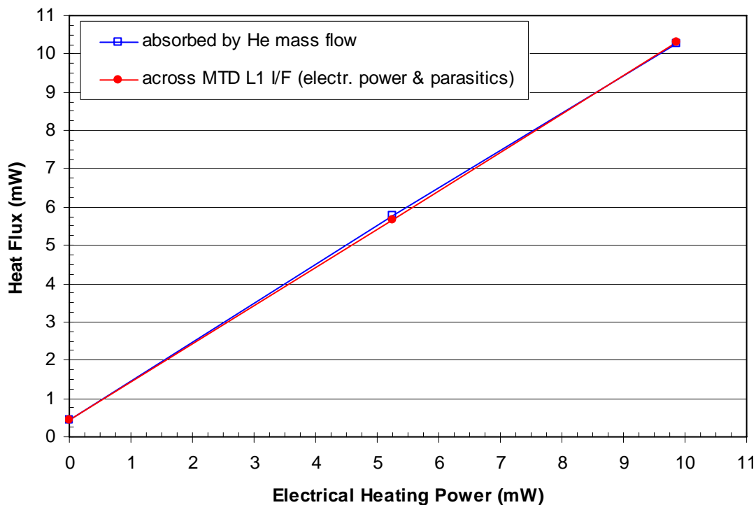
Figure 4.4-5: HIFI L1 Interface Heat Flows (TP4)
