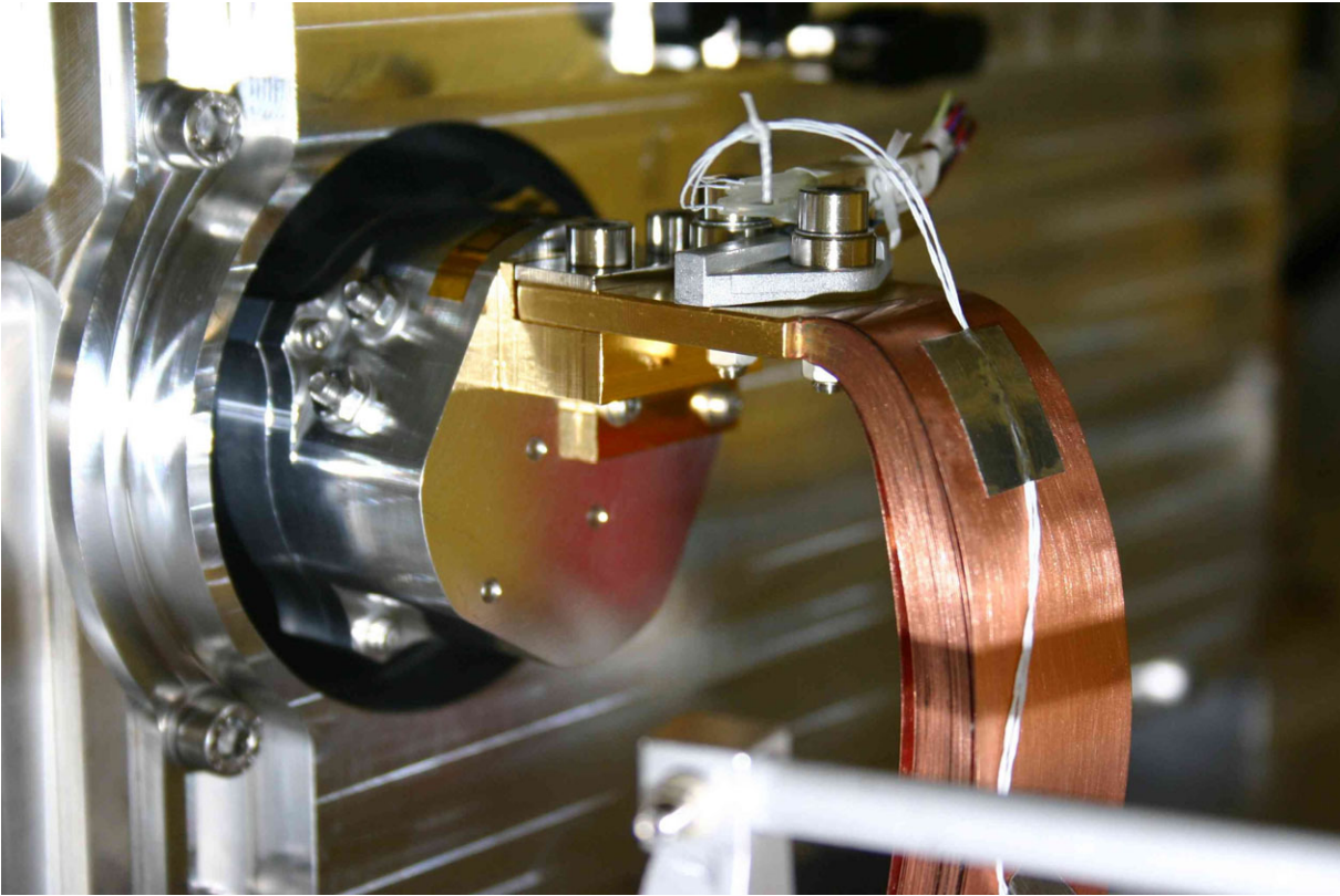
Figure 3.2-2: Temperature Sensor T224 – PACS Blue Detector FPU I/F
