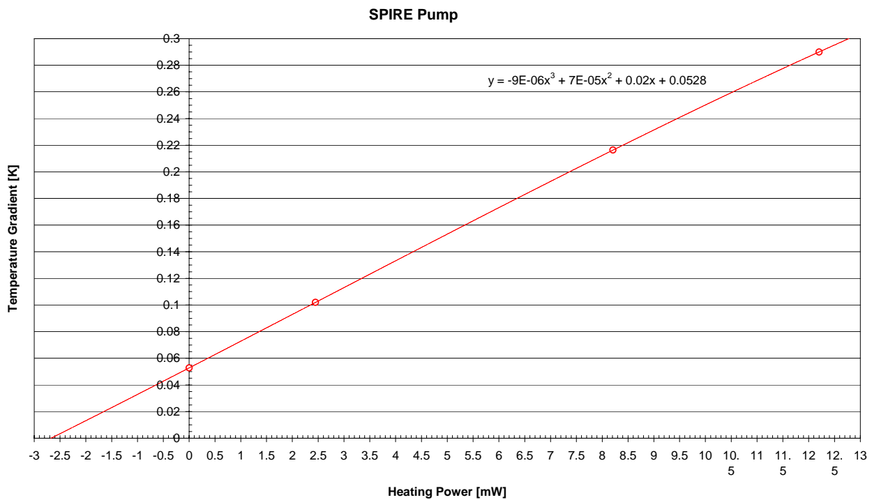
Figure 3.5-11: Temperature Gradient versus Electr. Heating Power at SPIRE Pump I/F
