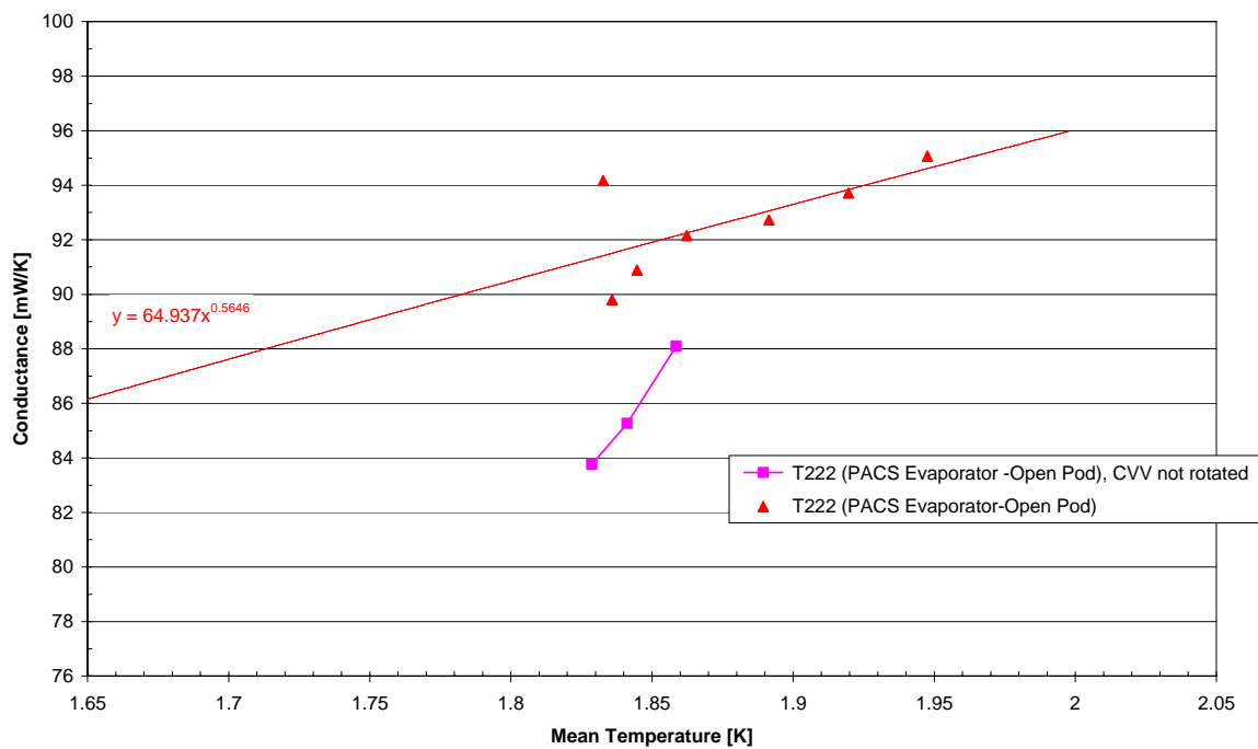
Figure 3.5-7: Thermal Conductance versus Mean Temperature for PACS L0 I/F to Helium
