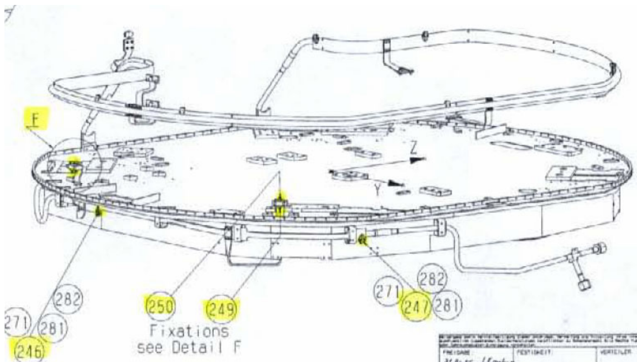
Figure 5.4-2: Distribution of Temperature Sensors on the L3 Ventline and L3 Interfaces
