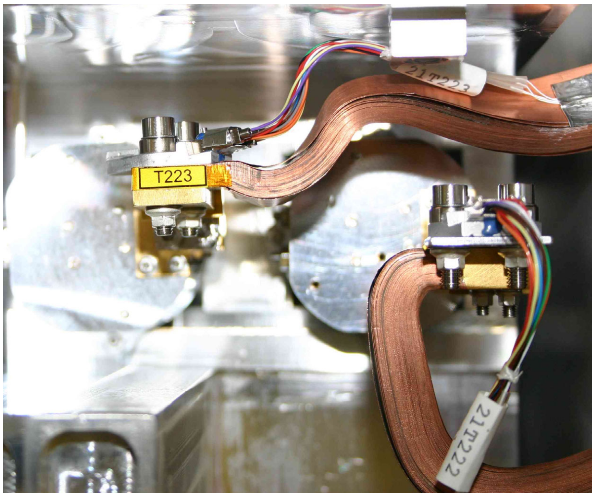
Figure 3.2-3: Temperature Sensors T222 and T223 – PACS Evaporator and Pump FPU I/F
