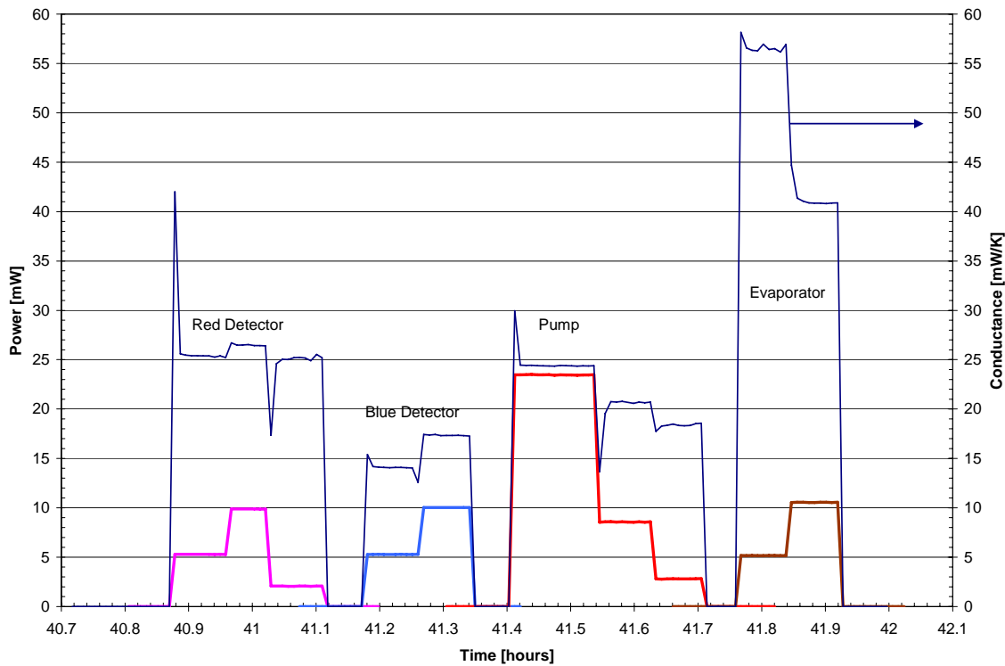
Figure 3.2-5: Electrical Heating Power and Thermal Conductance at PACS L0 Interfaces
