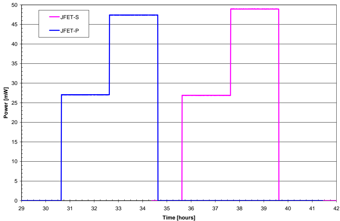
Figure 5.4-6: SPIRE JFET Power and Temperature Evolution during Operation (TP4)
