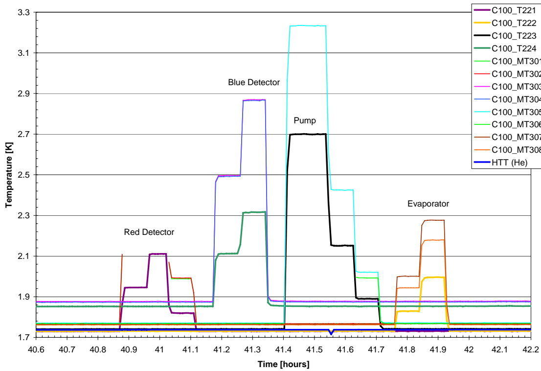
Figure 3.2-4: Temperature Evolution of PACS L0 Interfaces
