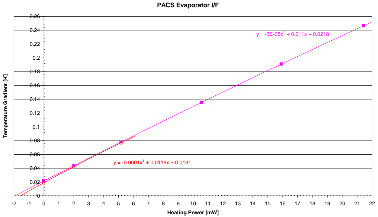
Figure 3.5-5: Temperature Gradient versus Electr. Heating Power at PACS Evaporator I/F (Open Pod)
