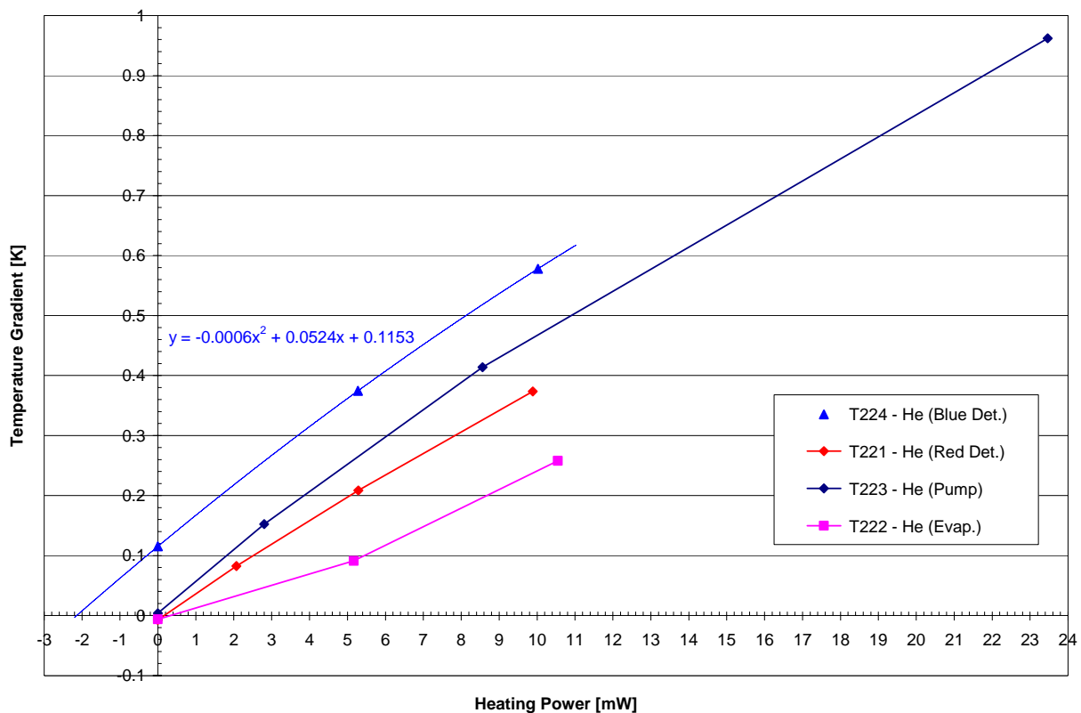
Figure 3.2-6: PACS L0 Temperature Gradients versus Electrical Heating Power
