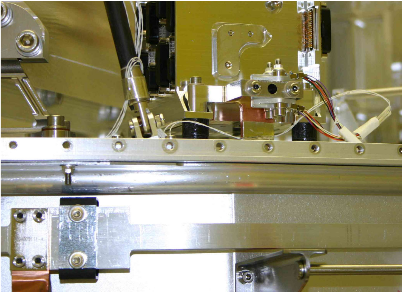
Figure 5.4-5: Temperature Sensor T244 – SPIRE L3 JFET-S
