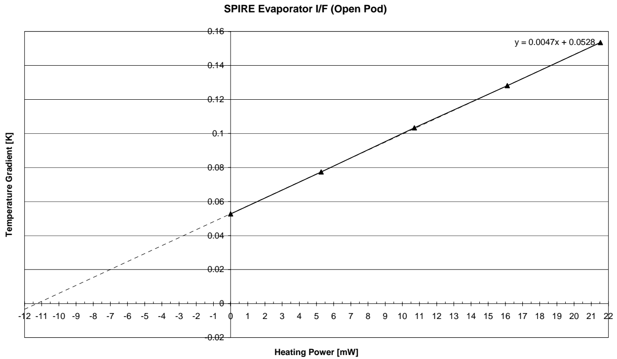
Figure 3.5-10: Temperature Gradient versus Electr. Heating Power at SPIRE Evaporator I/F (Open Pod)
