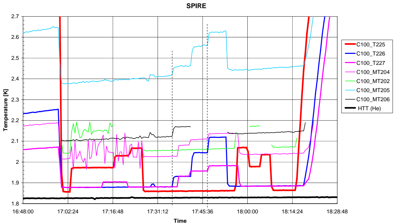
Figure 3.5-9: Temperature Evolution of SPIRE L0 Interfaces
