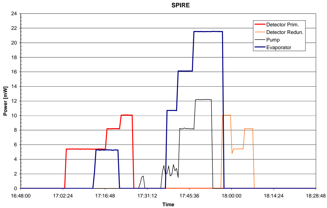
Figure 3.5-8: Electrical Power on SPIRE L0 Interfaces
