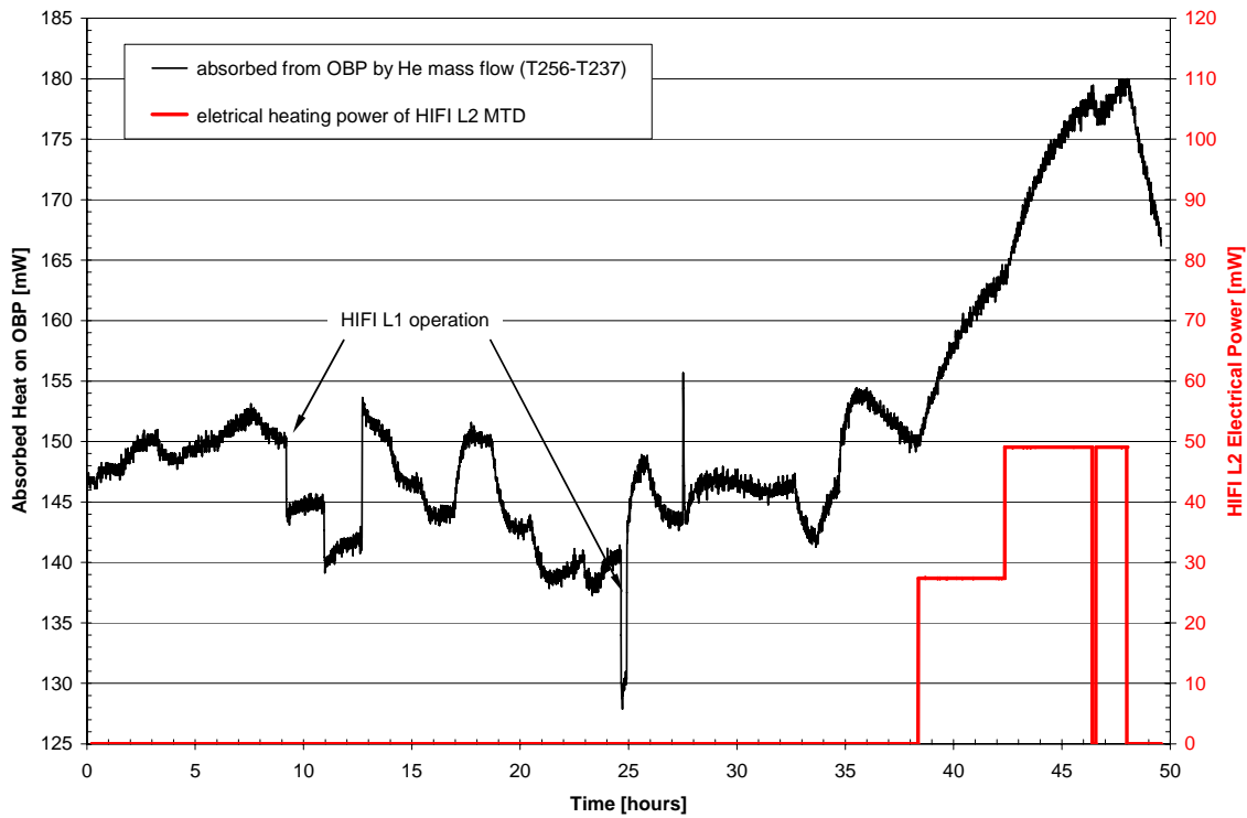
Figure 5.3-2: Absorbed Heat from OBP and HIFI L2 Power during TP6
