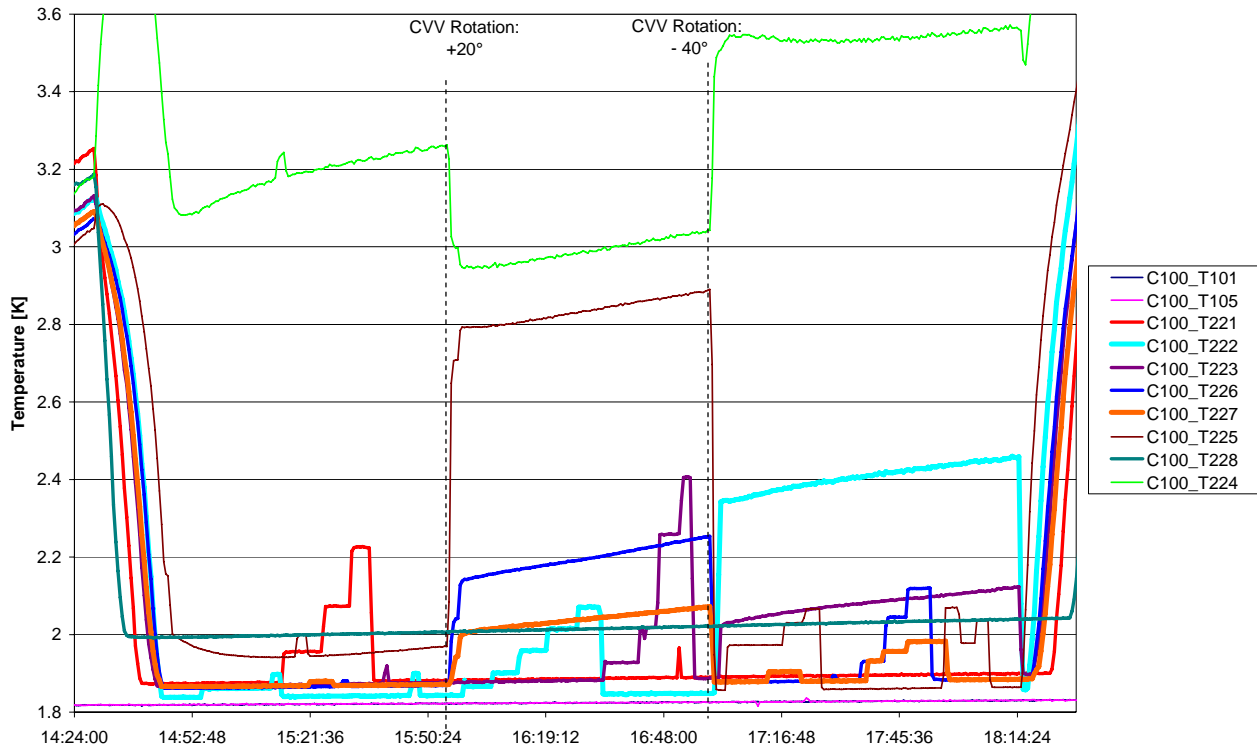
Figure 3.5-3: Temperature Evolution of all L0 Interfaces during Test
