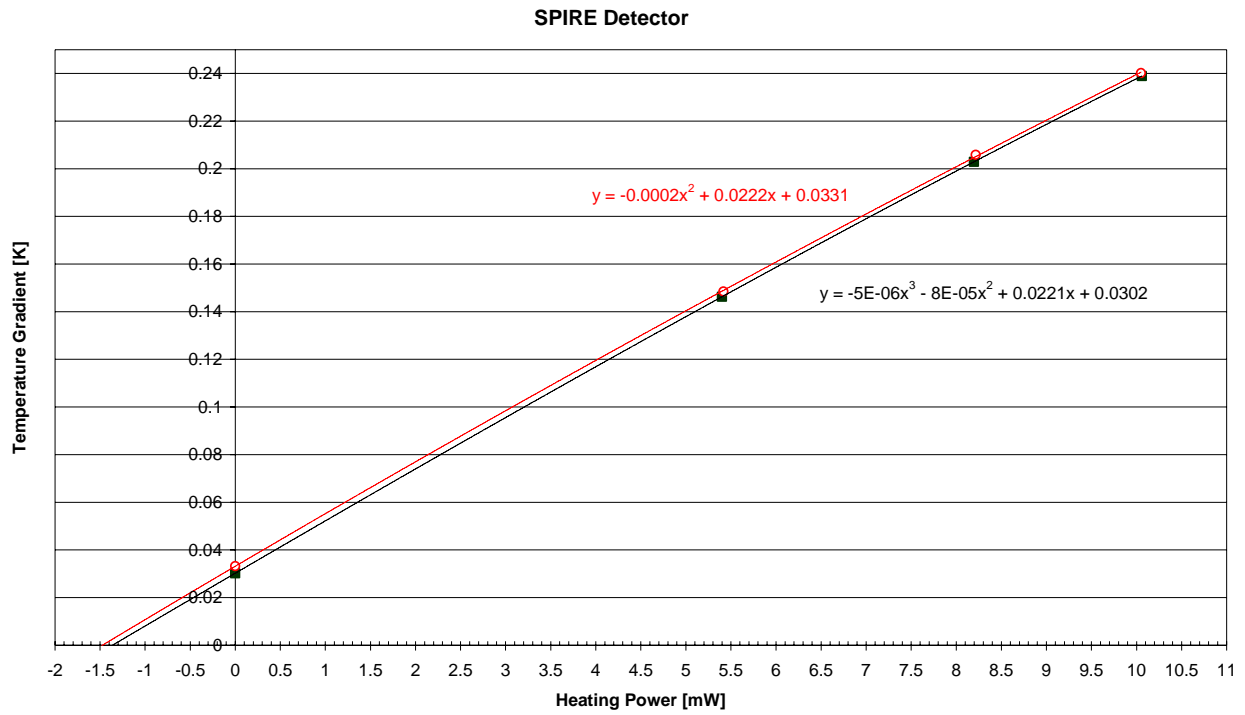
Figure 3.5-12: Temperature Gradient versus Electrical Heating Power at SPIRE Detector I/F
