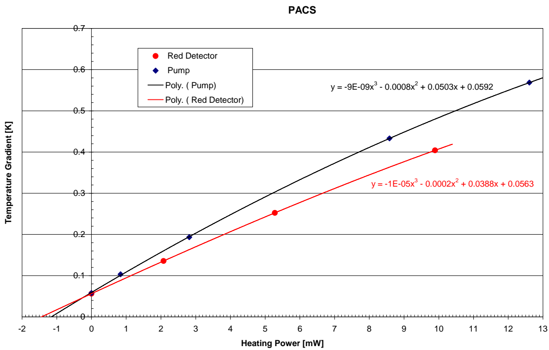
Figure 3.5-6: Temperature Gradient versus Electr. Heating Power at PACS Detector and Pump I/F
