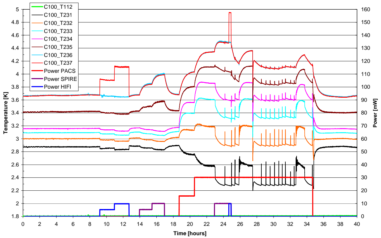
Figure 4.1-7: Temperature Evolution of Ventline (L1) during TP6
