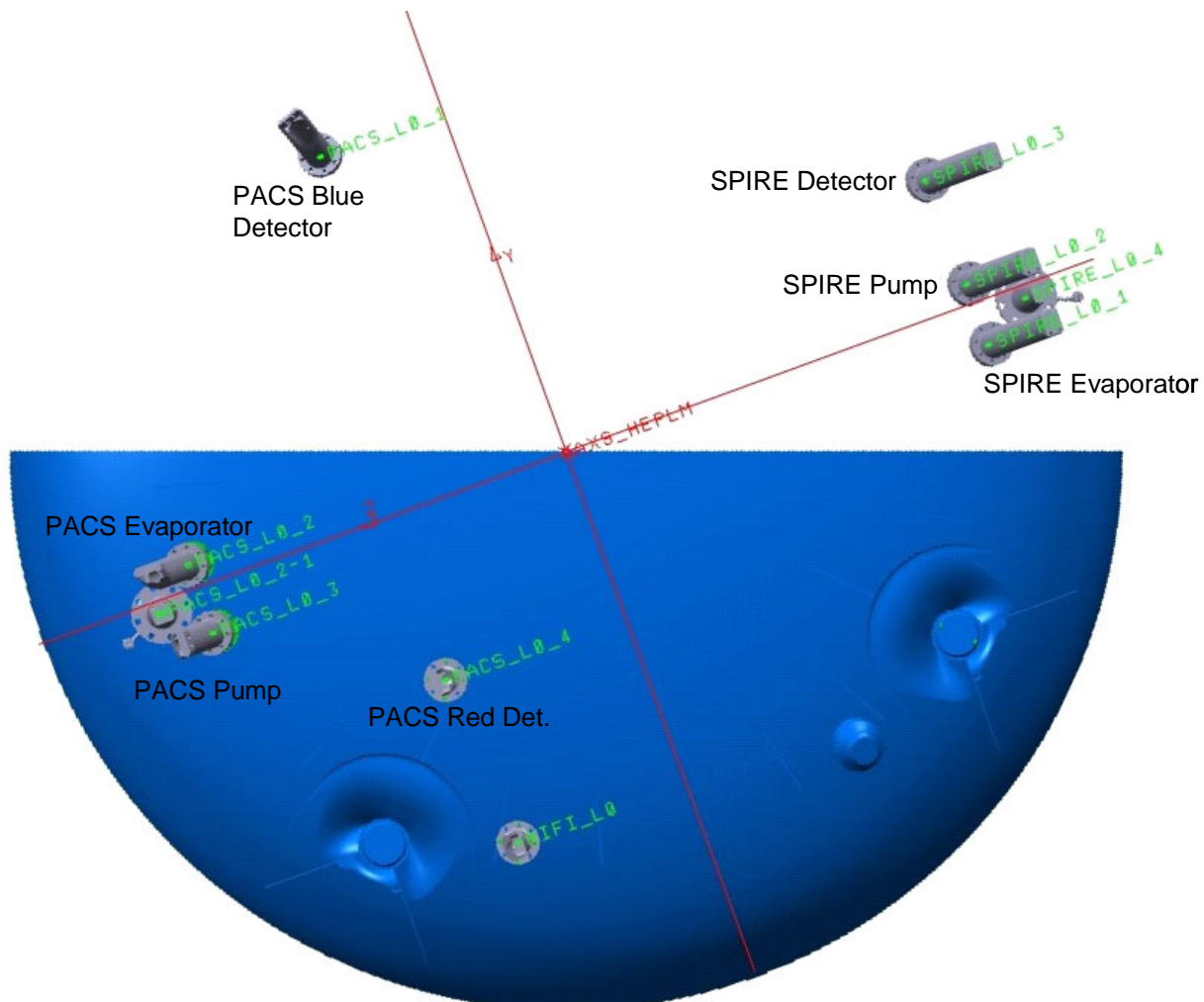
Horizontal CVV counter-clockwise rotated by 20^\circ with 50% Filling Charge in the HTT
