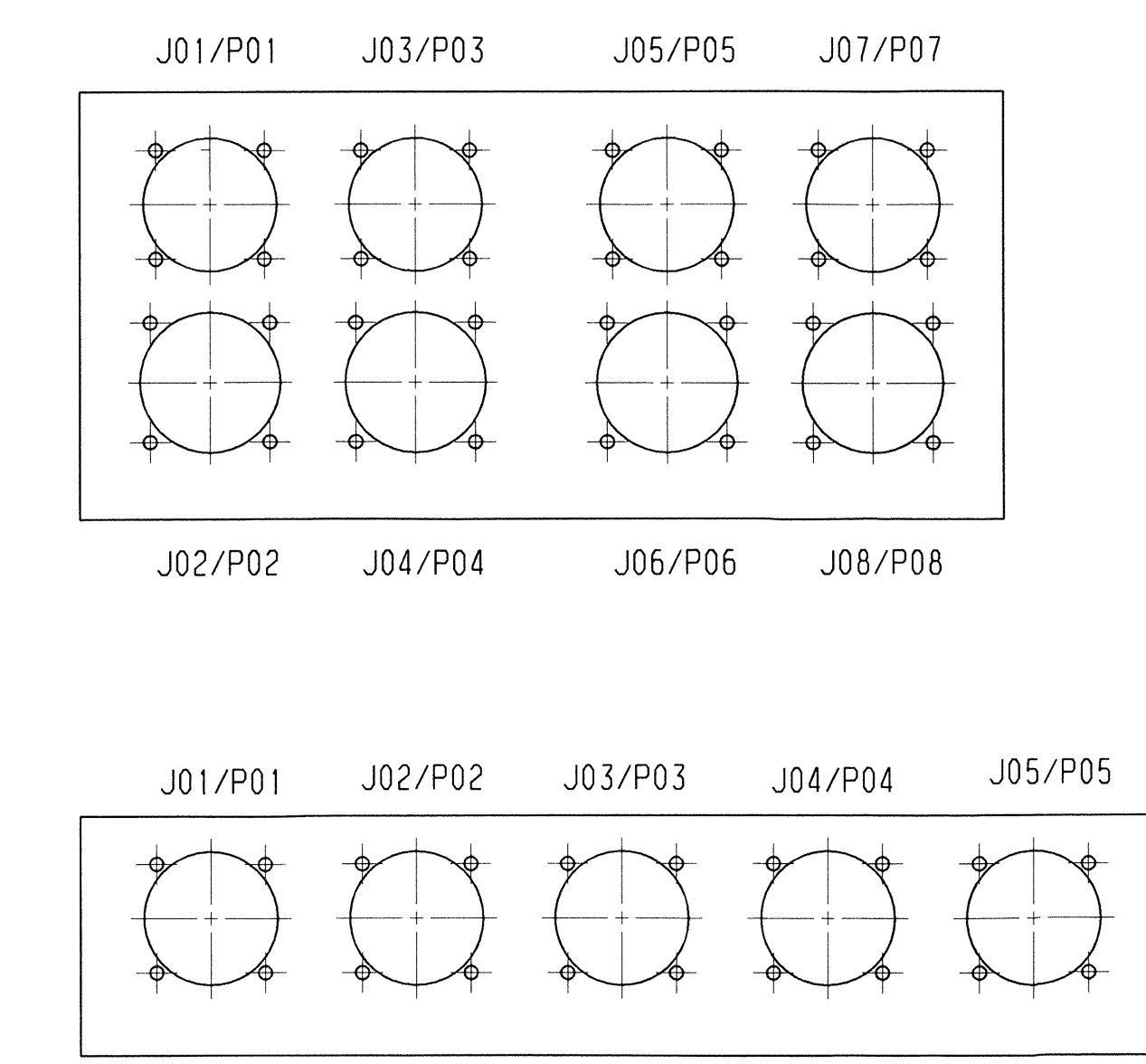
Typ. Marking of SVM Connector Brackets
