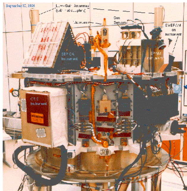
FIGURE 10. CRIS Instrument on ACE Spacecraft Bus
