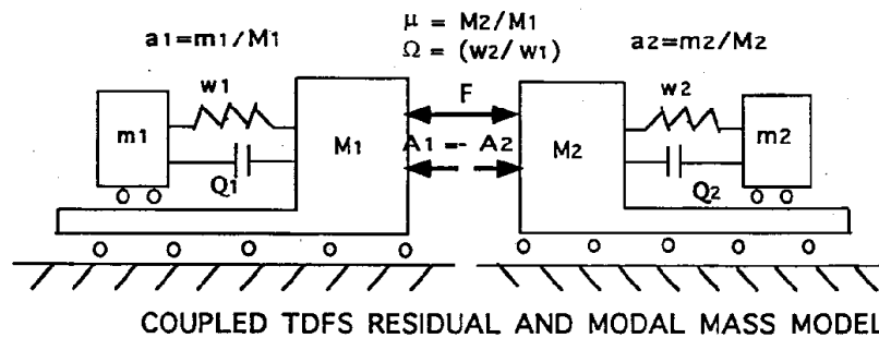
FIGURE 3. Complex TDFS With Residual and Modal Masses
