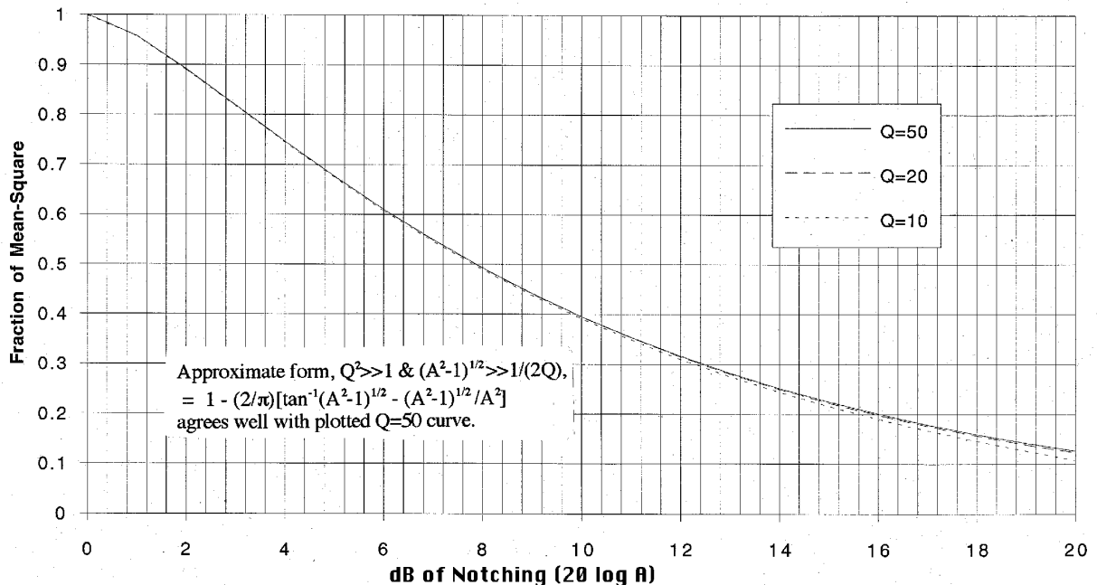
FIGURE 15. Reduction of SDFS Mean-Square Response by Notching
