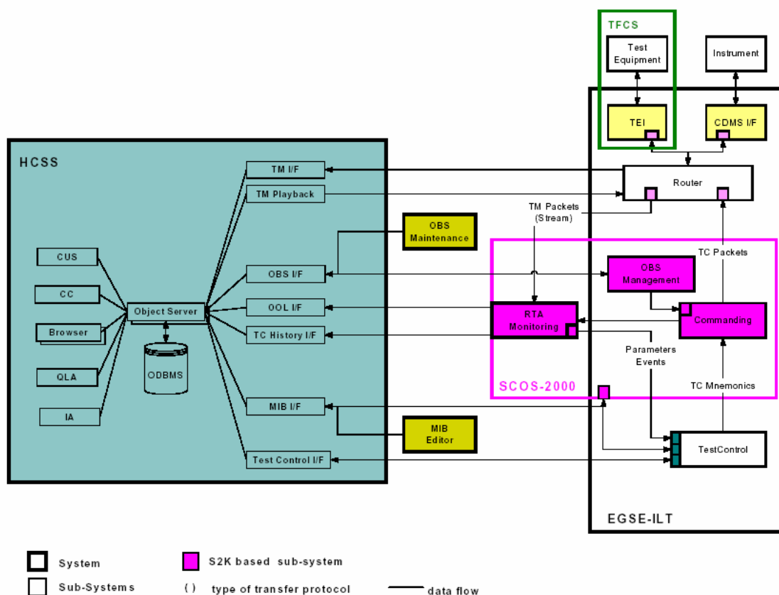
Figure 5: EGSE-ILT Configuration
