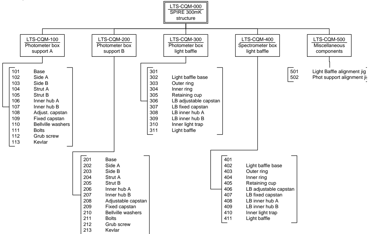
Figure 1 300mK Strap Supports & Light Baffles Hardware Tree
