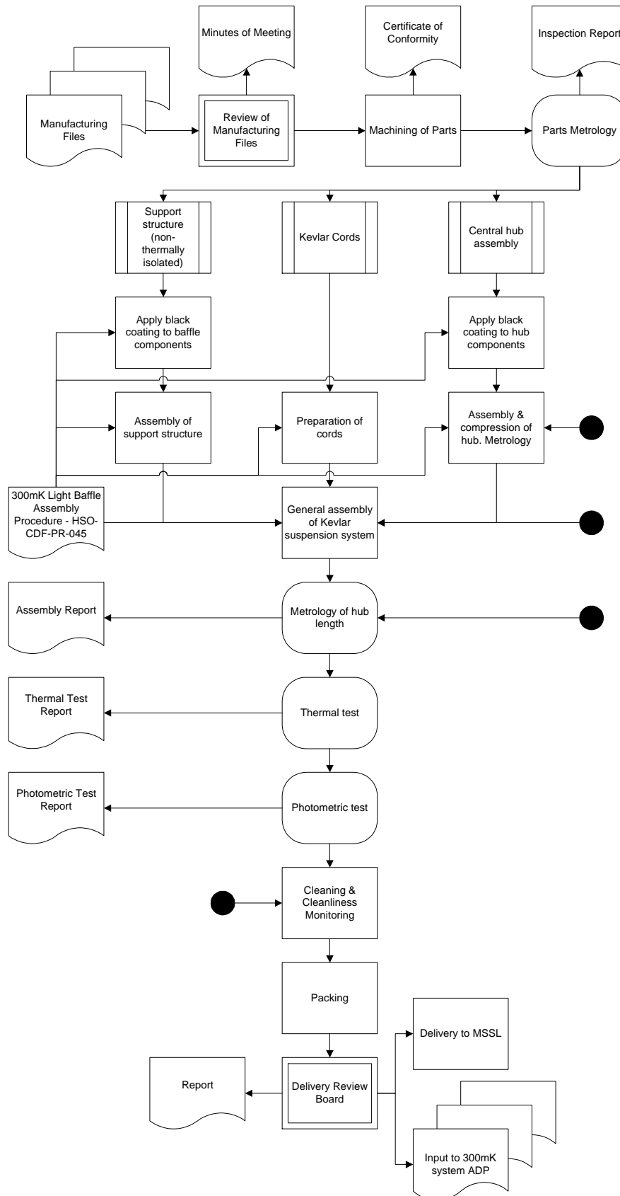
Figure 3 300mK Light Baffle MAIV Flowchart.
