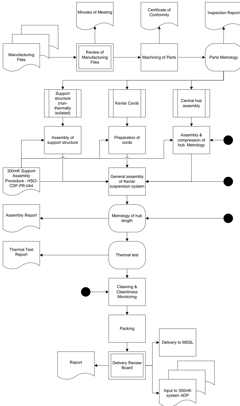
Figure 2 300mK Photometer Support MAIV Flowchart.
