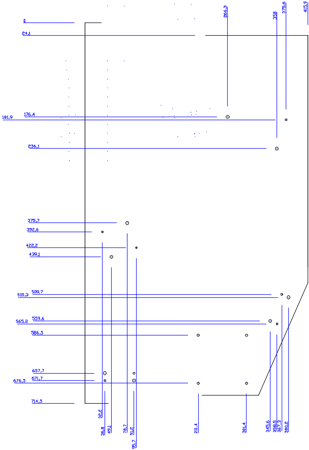
Figure 1 - Photometer side details.
