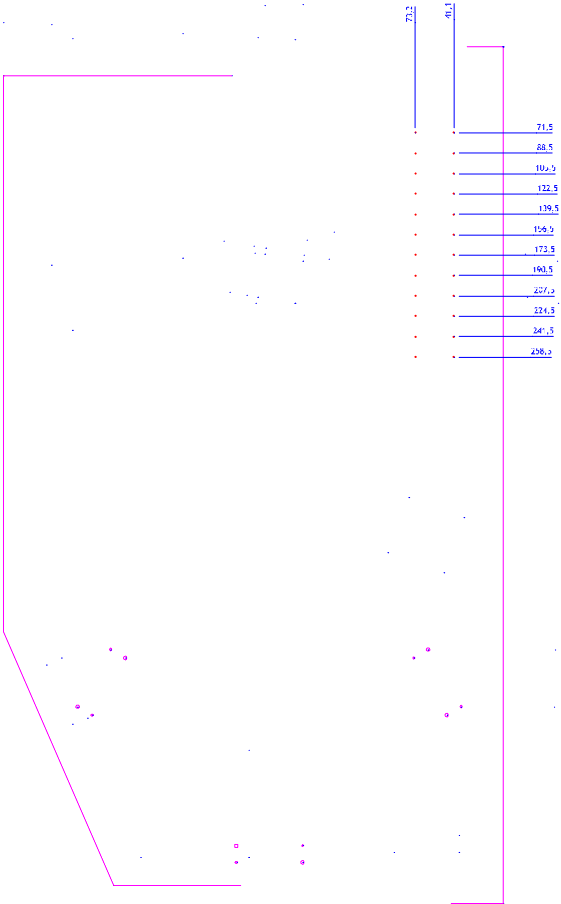
Figure 4 - Filter unit I/F holes. The surface of the filter unit is 140.9mm above the surface of the SPIRE Optical Bench
