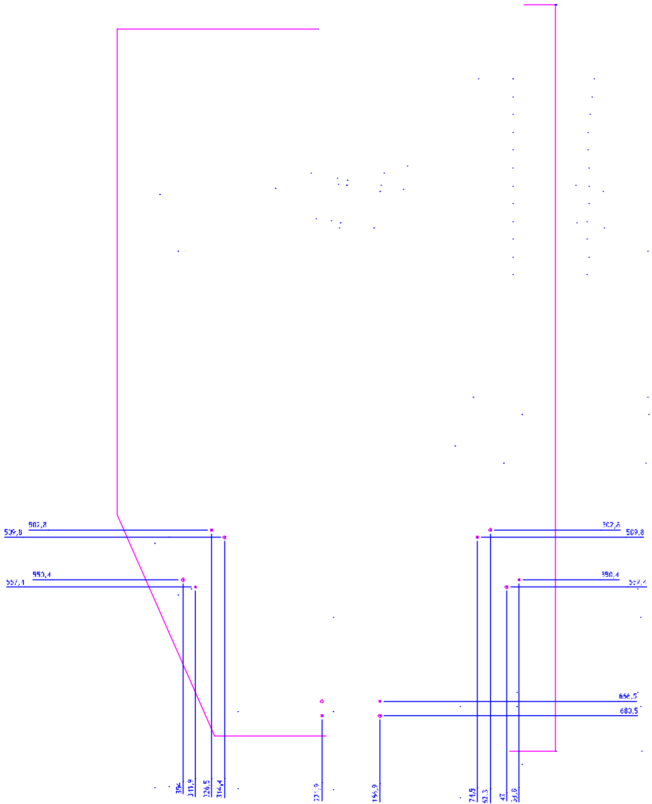
Figure 2 - Spectrometer detector box I/F boltholes.
