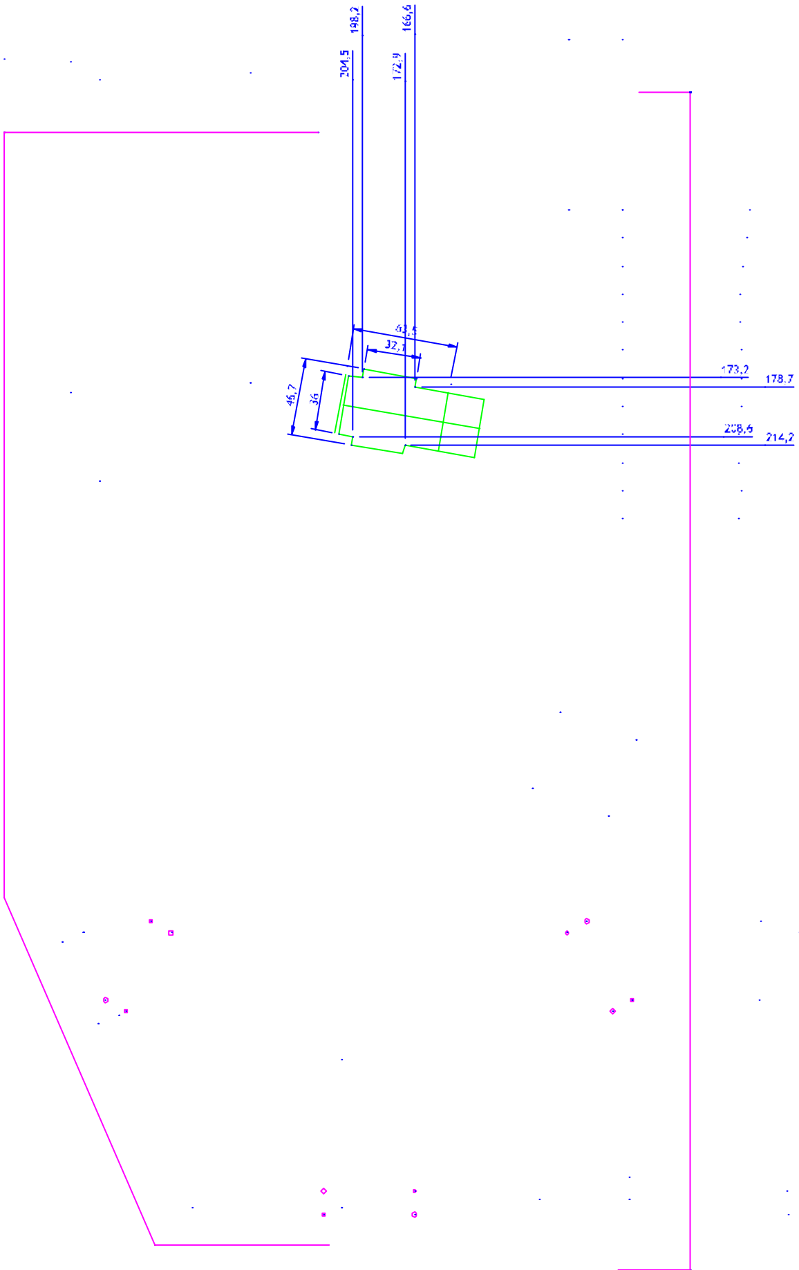
Figure 3 - S-Cal location. The centreline of the unit is 78.56mm above the level of the SPIRE Optical Bench
