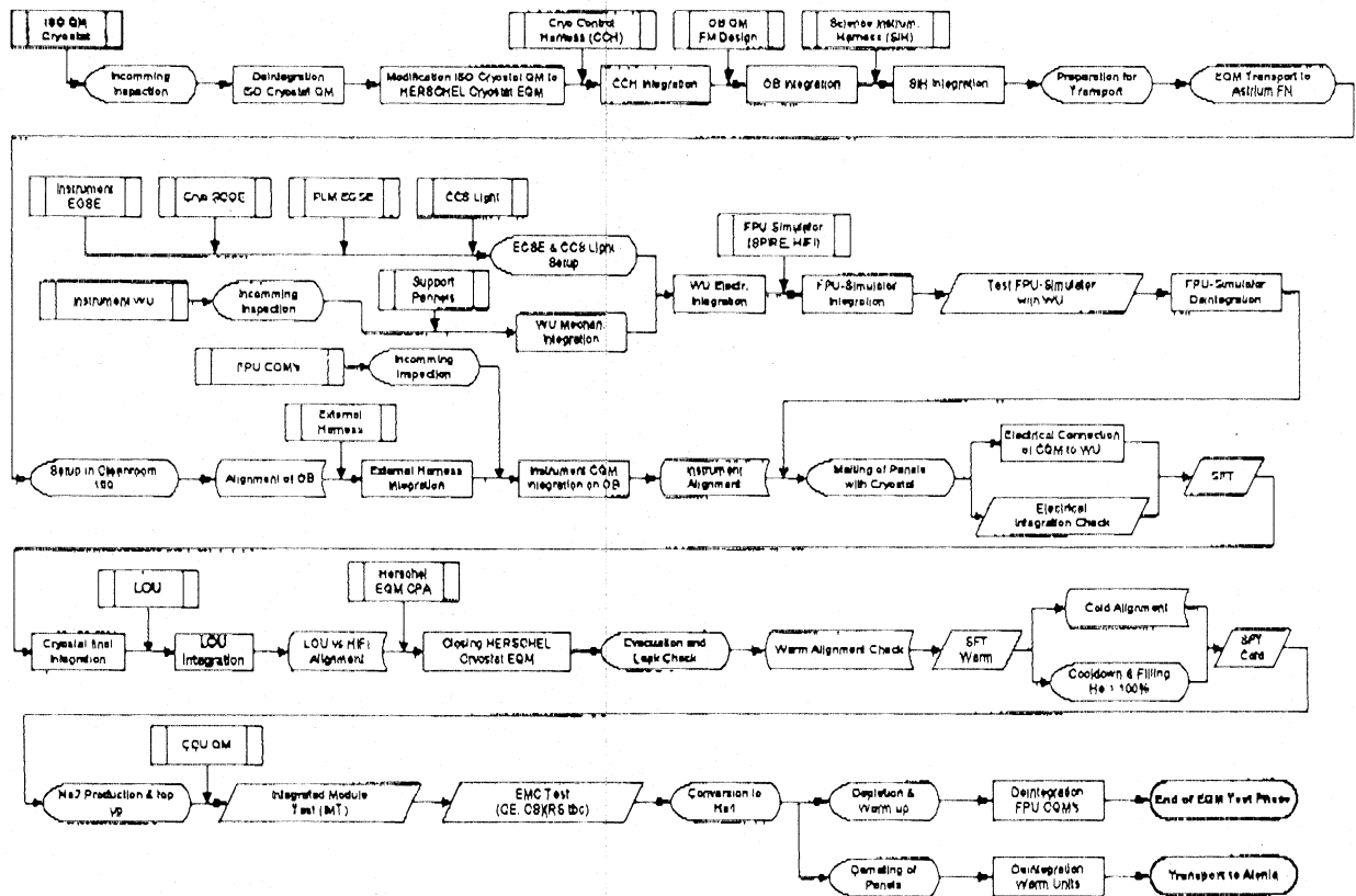
Fig. 1: AIT flow for EQM test phase
