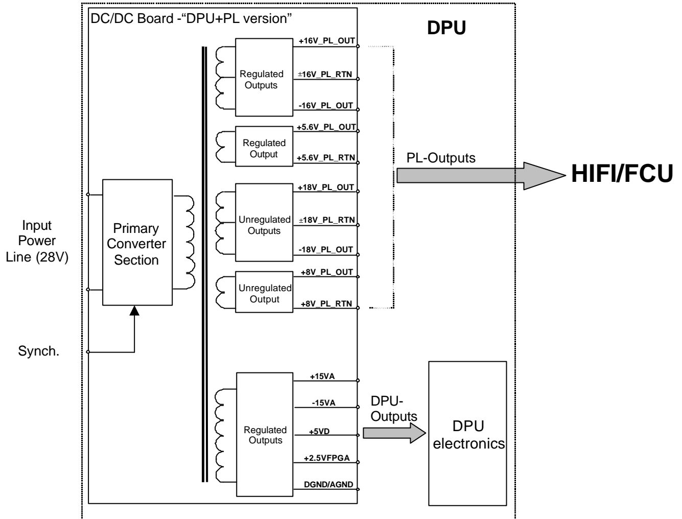
Fig. 5-1 DC/DC Board functional diagram ("DPU+PL version")
