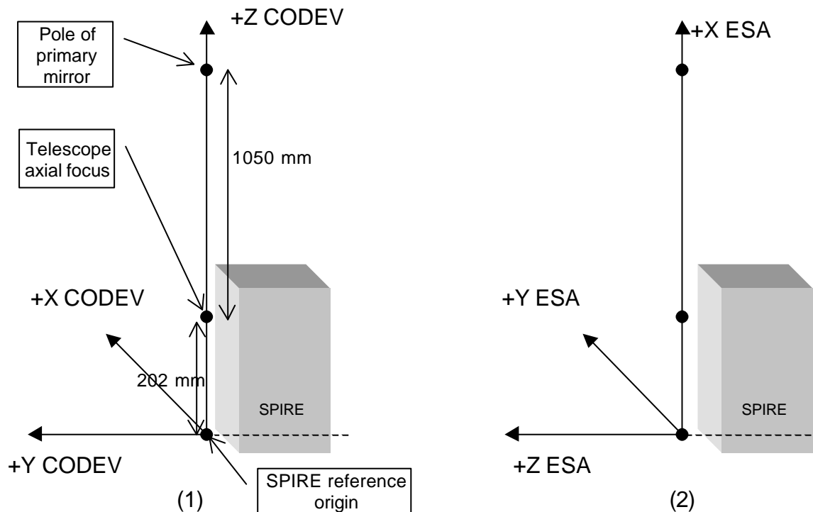
Reference co-ordinate systems used
