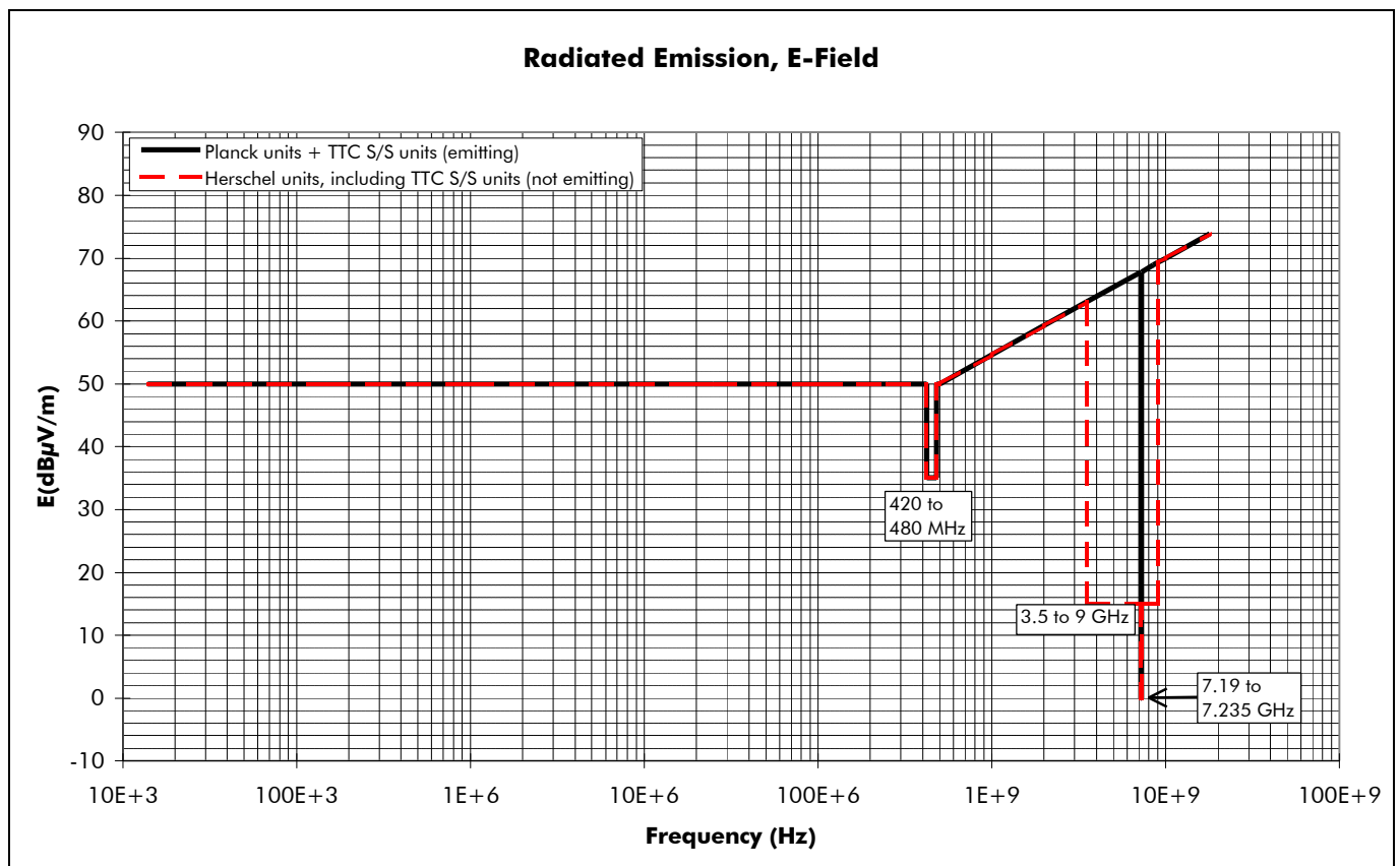
Figure 3.2.4.6-1 :Radiated emission E-field, NB
