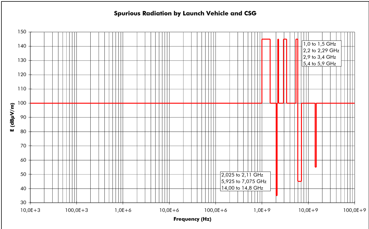
Figure 3.1.3.1-1 : Spurious radiation by launch vehicle and CSG : narrow-band electrical field
