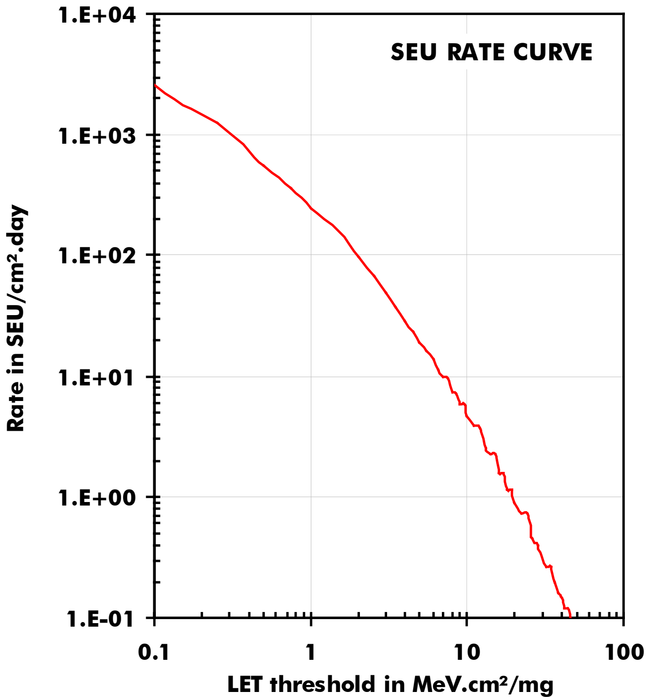
Figure 3-28: Heavy Ions Induced SEU rate
