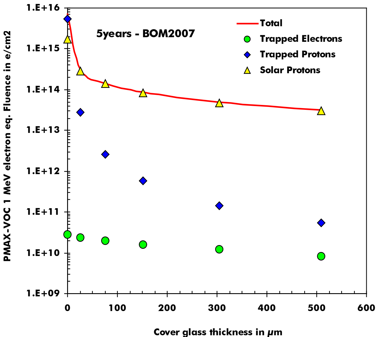
Figure 3-40: Mission 1 MeV electron Equivalent Fluence for PMAX in GaAs
