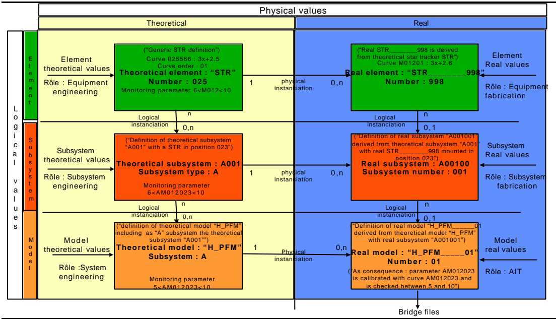
Figure 1-1 - Higher level data model
