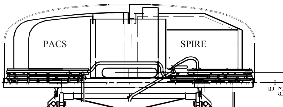
Figure 5.3-2: The HERSCHEL Focal Plane, side view towards +Y
