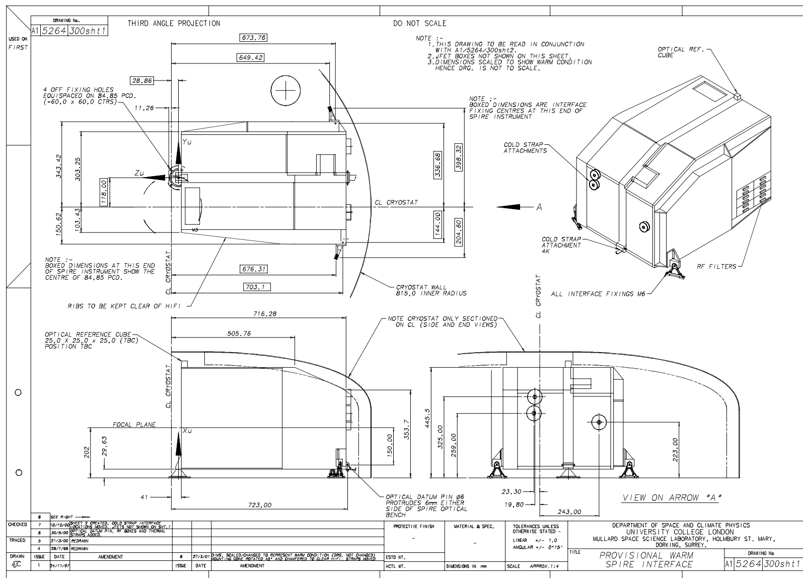
Figure 5.4-1a: Spire Focal Plane Unit.....sheet 1
