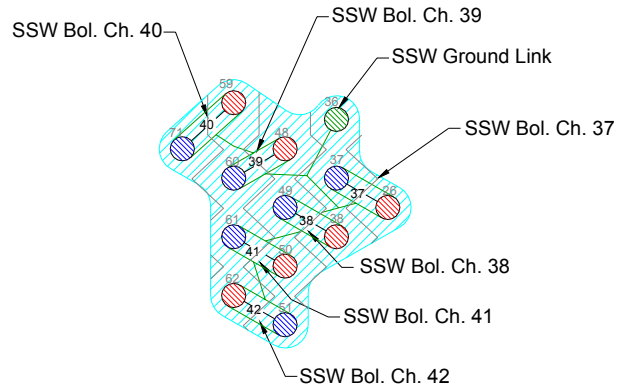
Bolometer Channel Tail D (DCU P26)
