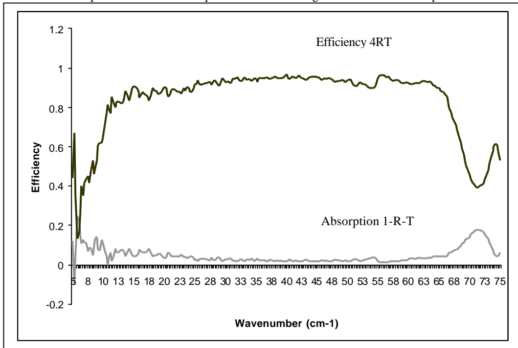
Figure 4: Measured performance of the capacitive-inductive grid broadband beam splitters of the same type
