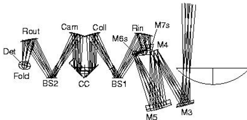
Figure 2. Optical diagram of the upper half of the SPIRE spectrometer. The symmetrical lower half is generated by reflection about the plane containing the two beam splitters.
