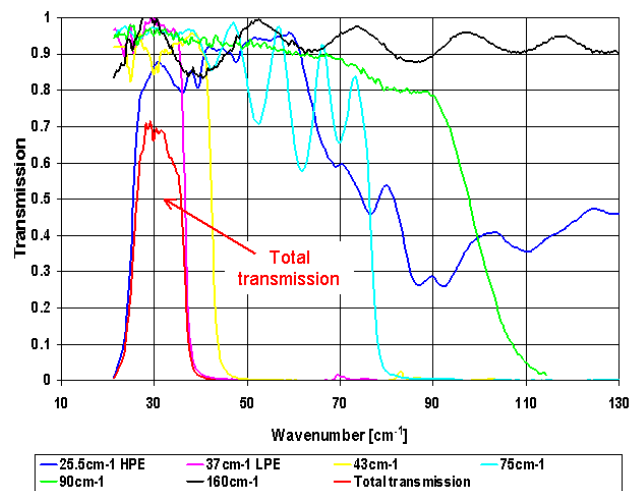
Figure 3. SPIRE 350\text{-}\mu\text{m} band prototype filtering scheme
