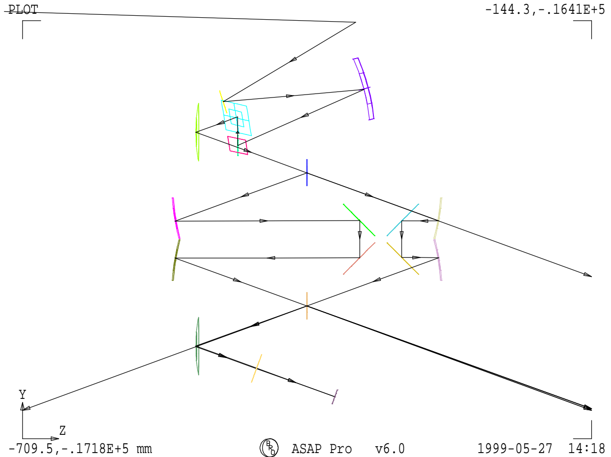
Fig.5. FTS with rooftop moved to left by \Delta z=100\text{mm} (gives \text{OPD}=8. \Delta z )
