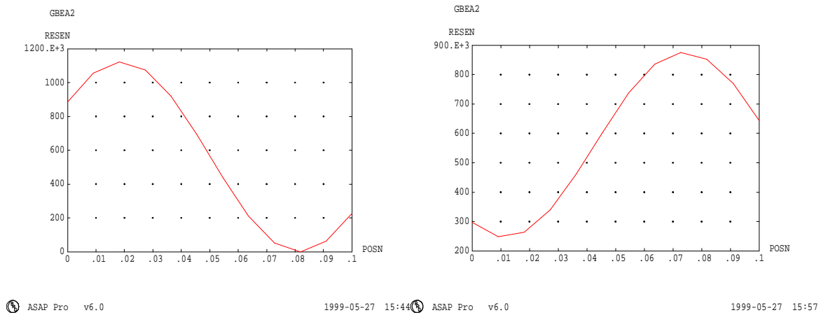
Fig.9. FTS 1/2-wave scan (detector energy vs rooftop position), for +Y FOV, Left: near OPD=0, Right: near OPD=8*100mm.
