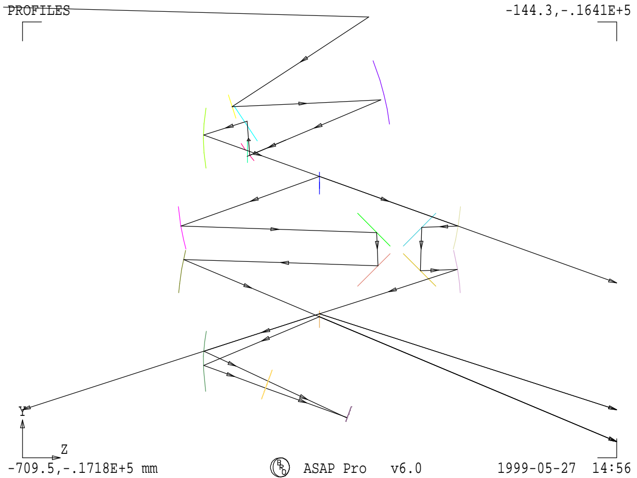
Fig.7. Beam paths at +Y extreme of FOV, max OPD.
