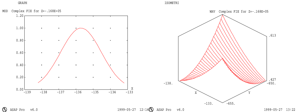
Fig.3. Single-beam pattern at detector. Modulus at left, wavefront (in number of waves) at right.
