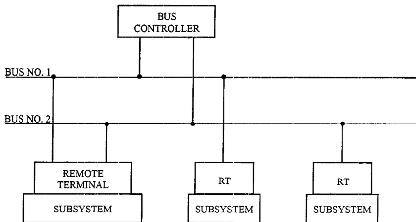
FIGURE 10.1. Illustration of Possible Redundancy
