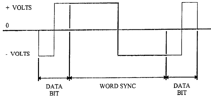
FIGURE 4. Command and Status Sync
