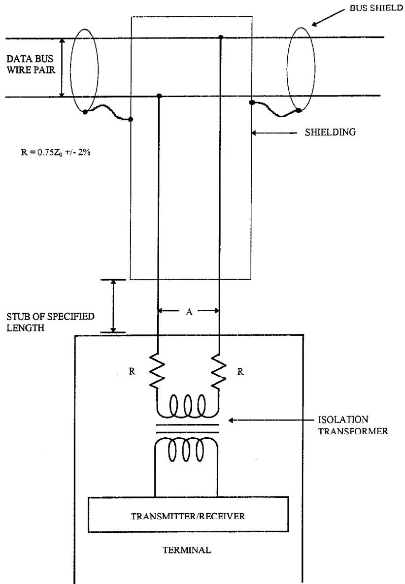
FIGURE 10. Data Bus Interface Using Direct Coupling
