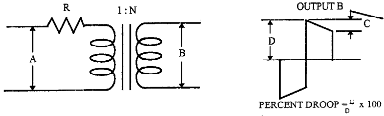
FIGURE 11. Coupling Transformer
