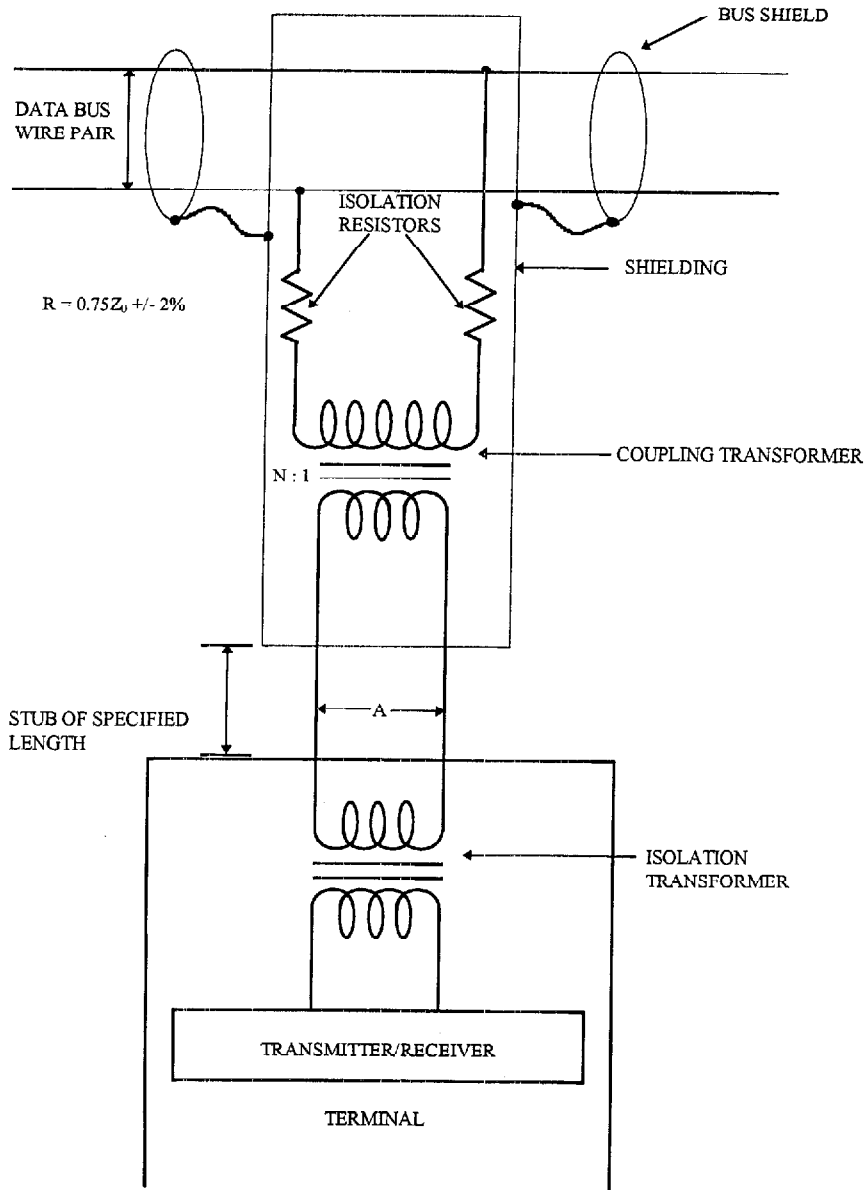
FIGURE 9. Data Bus Interface Using Transformer Coupling
