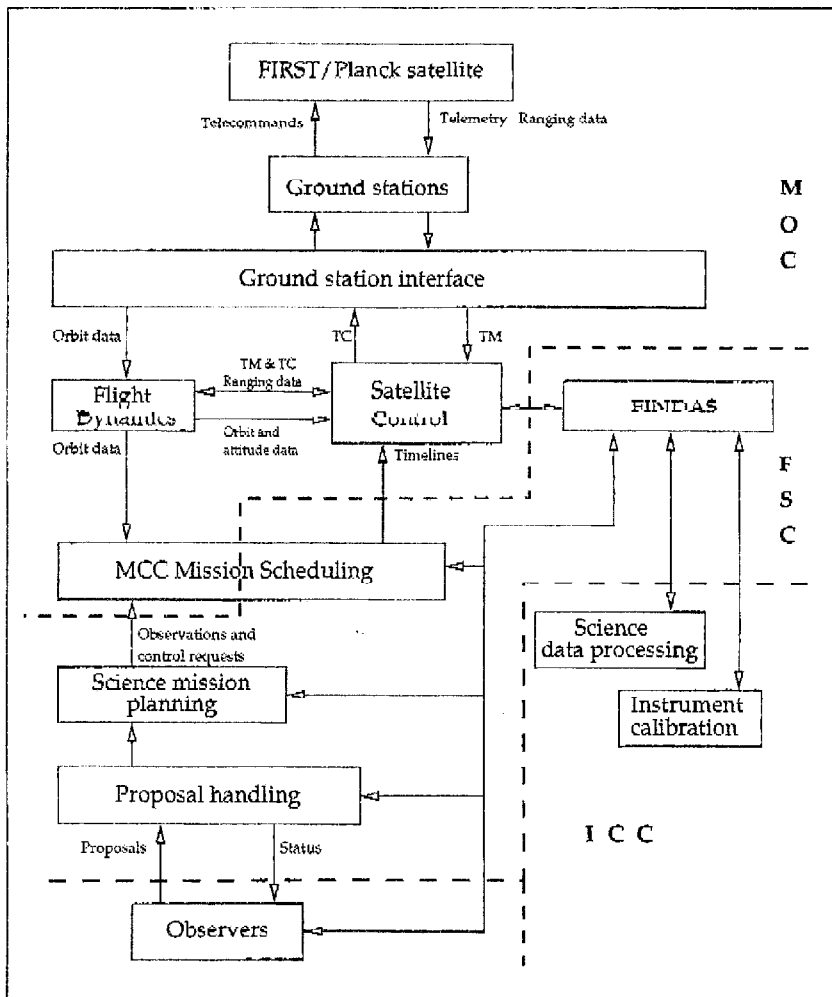
Figure 15: The mission operations phase ground segment
