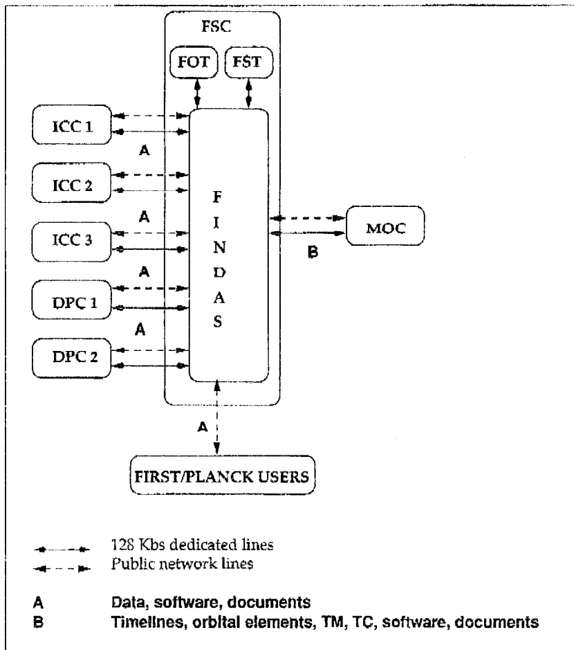
Figure 1: The FIRST/PLANCK ground segment
