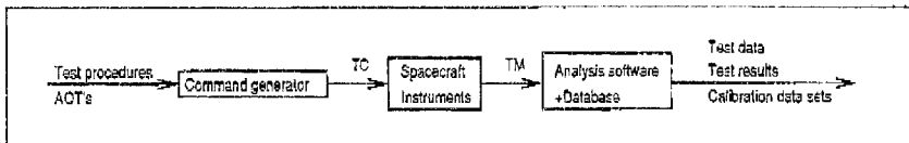
Figure 9: Instrument and spacecraft development data flow
