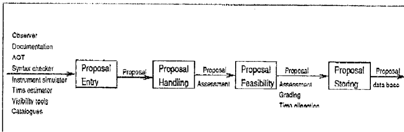
Figure 13: Mission preparations data flow
