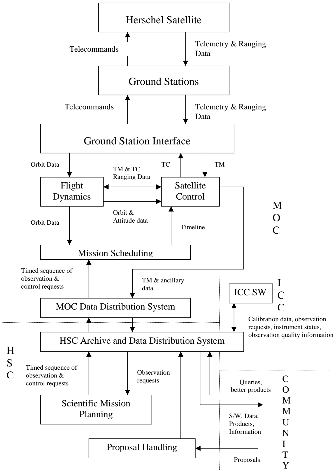
Figure 2-1 Ground Segment Overview
