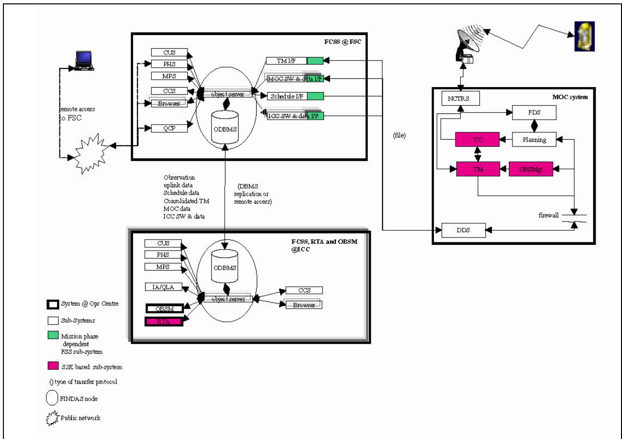
Figure 2-3 The Herschel Ground Segment in Routine Operations Phase
